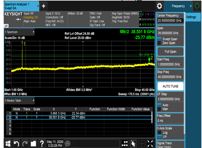
CSE n77 15M CH664832 BPSK(1,1)_
