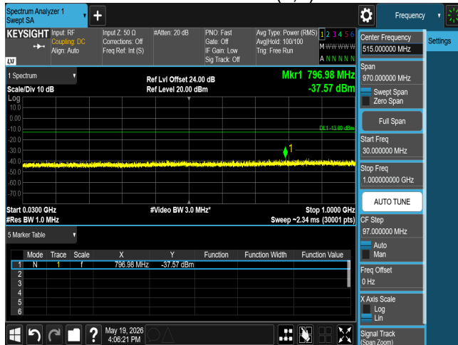
CSE n77 15M CH656000 BPSK(1,1)
