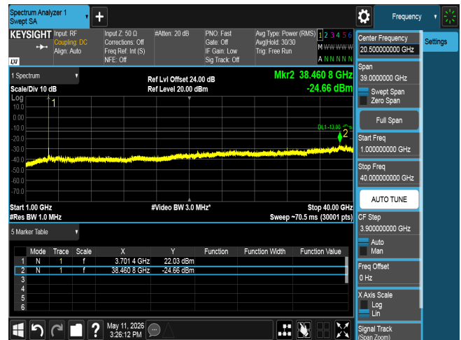
CSE n77 15M CH647168 BPSK(1,1)
