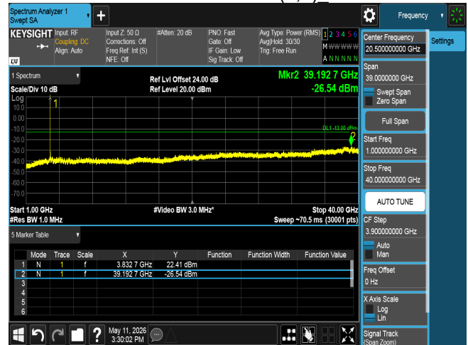
CSE n77 15M CH656000 BPSK(1,1)
