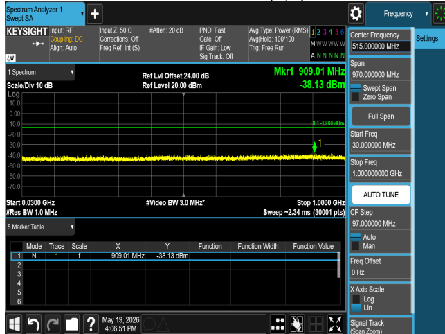
CSE n77 15M CH664832 BPSK(1,1)
