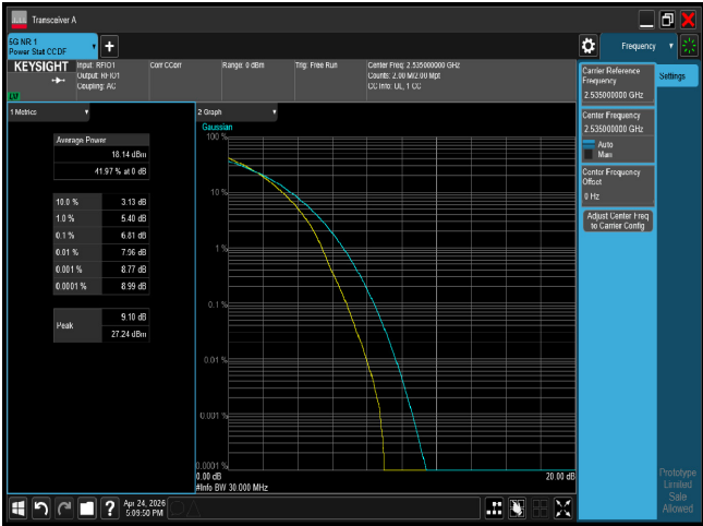
PTAR n7 30M CH507000 256QAM
