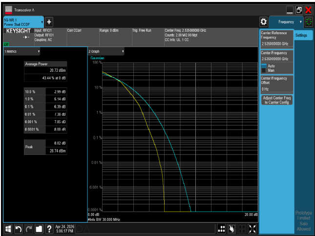
PTAR n7 30M CH507000 16QAM
