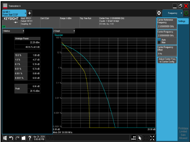
PTAR n7 30M CH507000 BPSK
