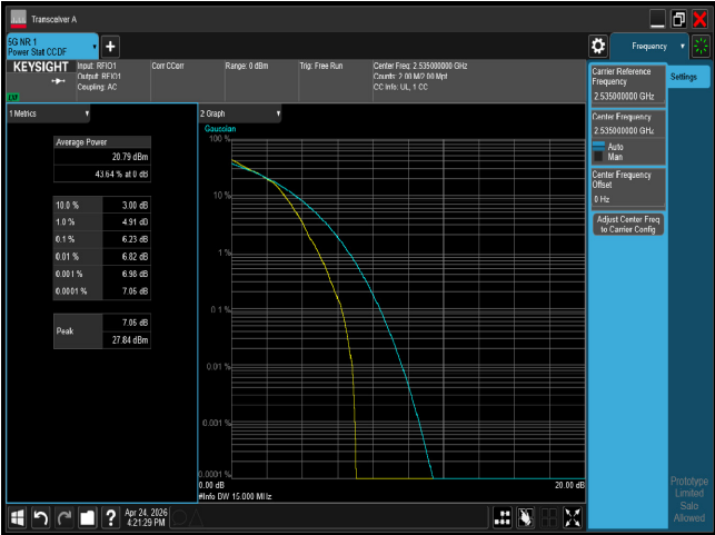
PTAR n7 15M CH507000 16QAM
