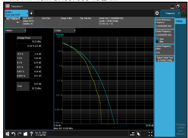
PTAR n7 10M CH507000 256QAM
