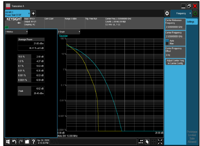
PTAR n7 15M CH507000 QPSK
