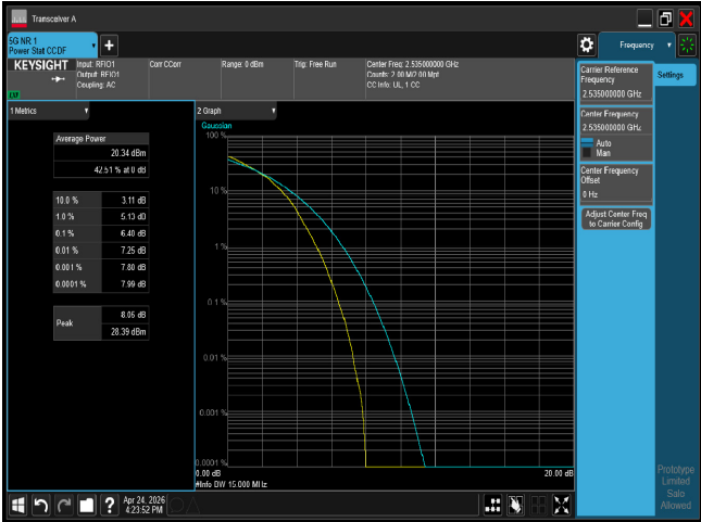
PTAR n7 15M CH507000 64QAM
