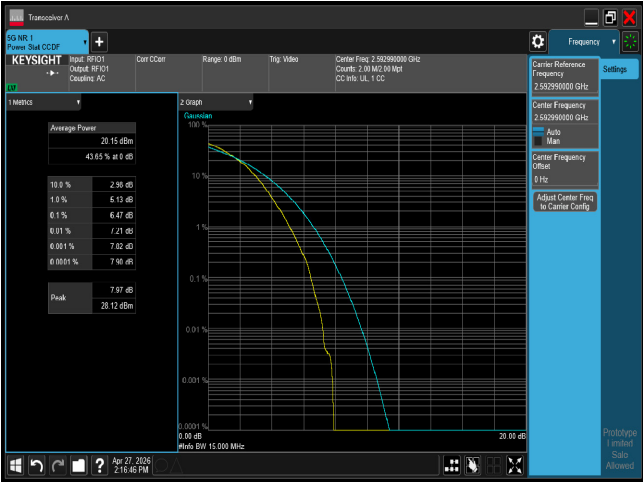
PTAR n41 15M CH518598 64QAM
