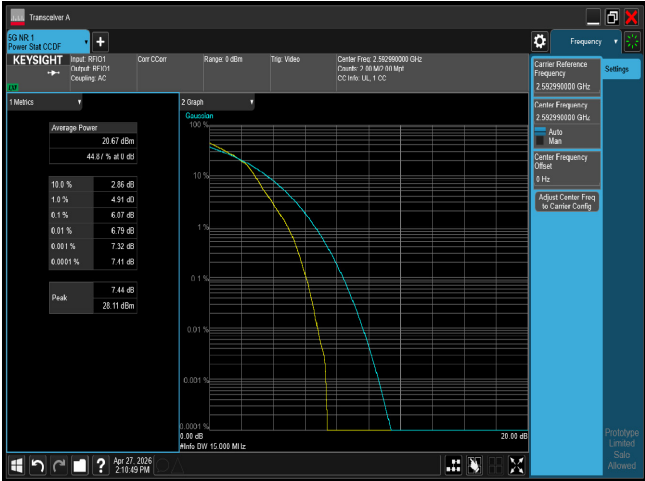
PTAR n41 15M CH518598 16QAM
