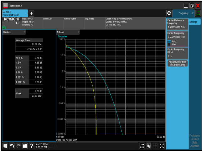
PTAR n41 20M CH518598 QPSK
