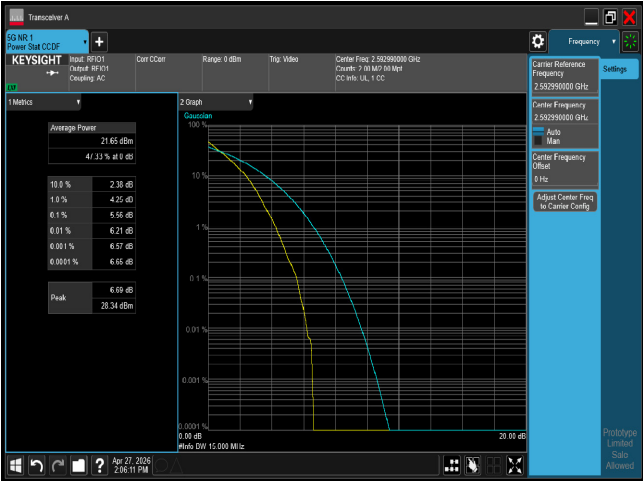
PTAR n41 15M CH518598 QPSK
