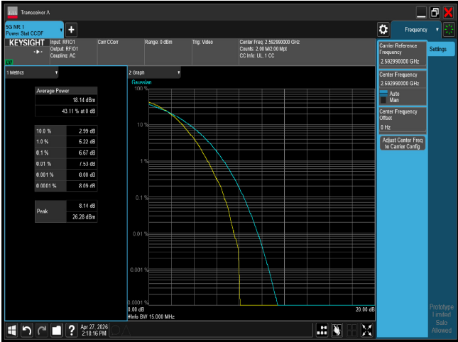
PTAR n41 15M CH518598 256QAM
