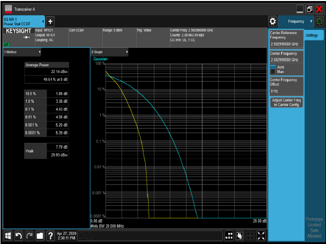
PTAR n41 20M CH518598 BPSK
