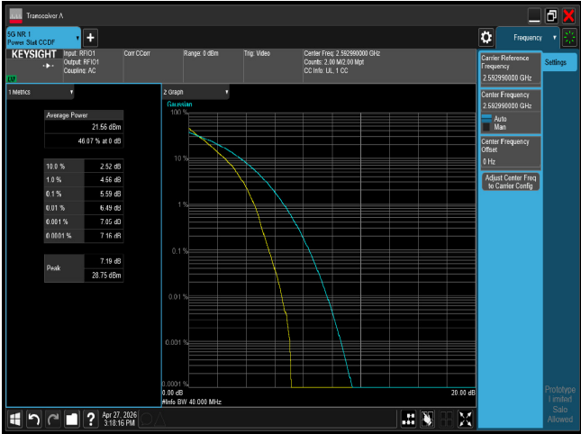
PTAR n41 40M CH518598 QPSK
