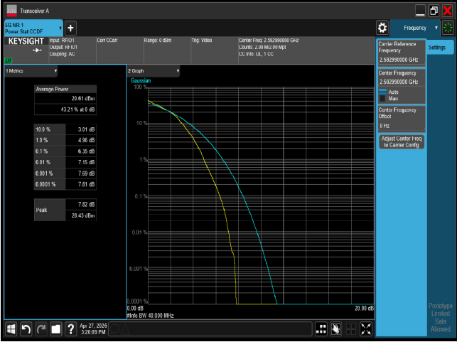
PTAR n41 40M CH518598 16QAM
