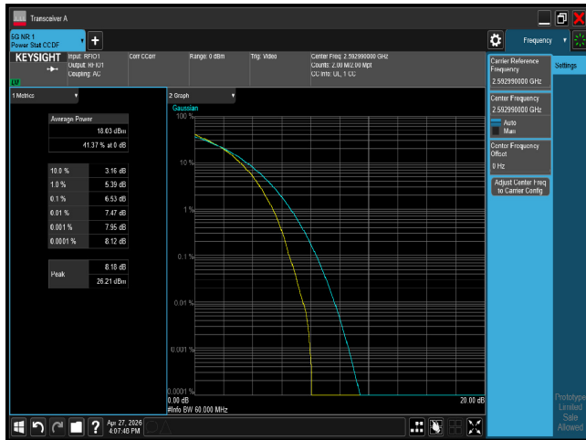
PTAR n41 60M CH518598 256QAM
