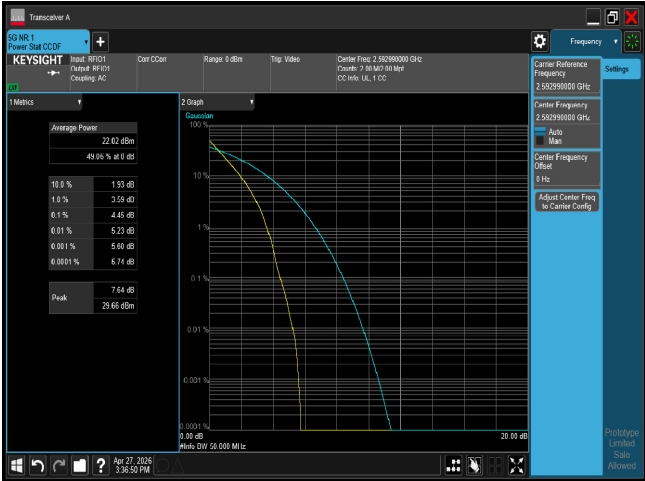
PTAR n41 50M CH518598 BPSK
