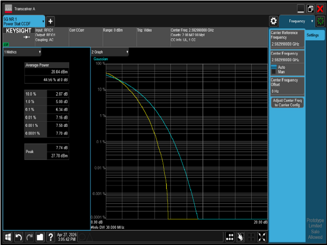
PTAR n41 30M CH518598 64QAM
