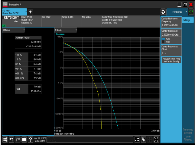
PTAR n41 40M CH518598 64QAM
