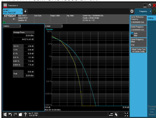
PTAR n41 60M CH518598 16QAM
