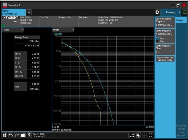
PTAR n41 50M CH518598 64QAM
