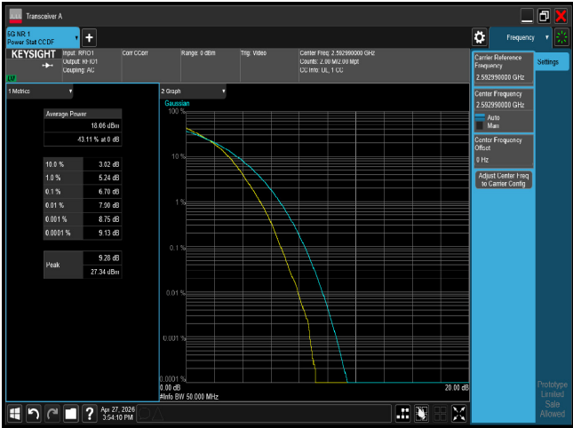
PTAR n41 50M CH518598 256QAM
