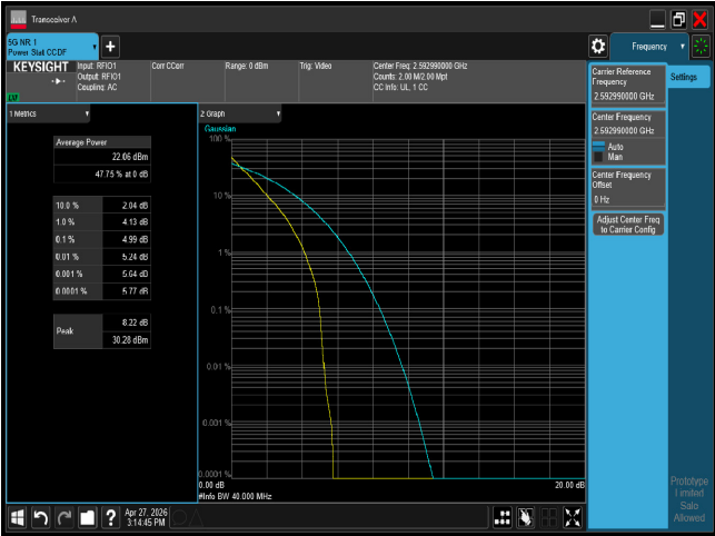
PTAR n41 40M CH518598 BPSK
