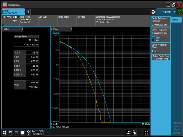
PTAR n41 40M CH518598 256QAM
