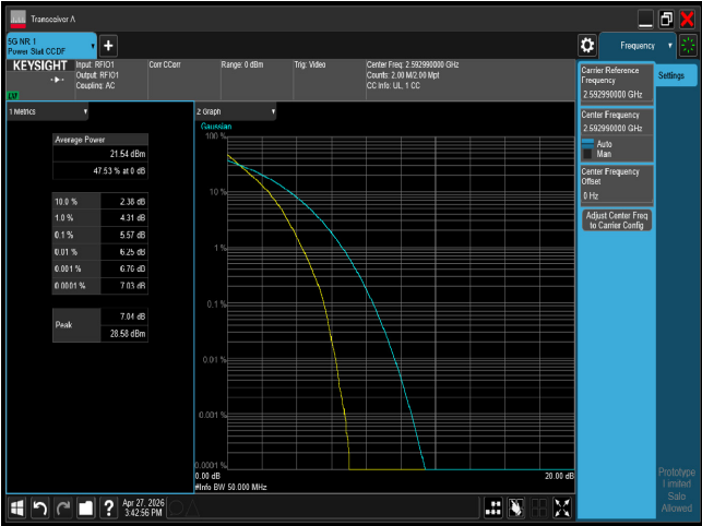
PTAR n41 50M CH518598 QPSK
