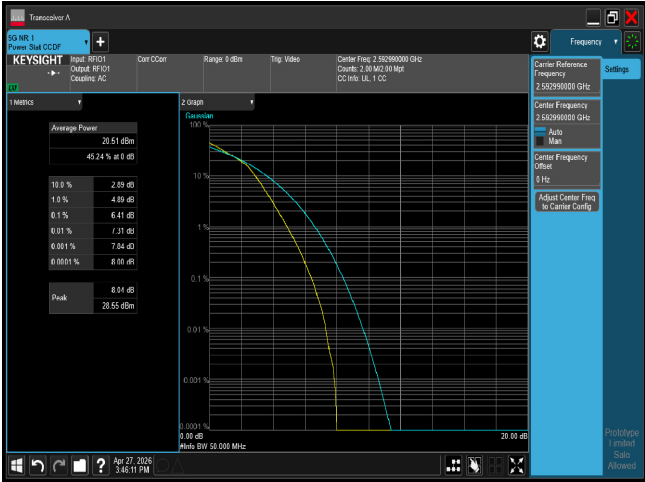
PTAR n41 50M CH518598 16QAM
