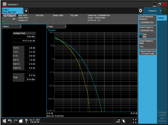
PTAR n41 30M CH518598 256QAM
