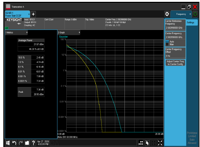
PTAR n41 60M CH518598 QPSK
