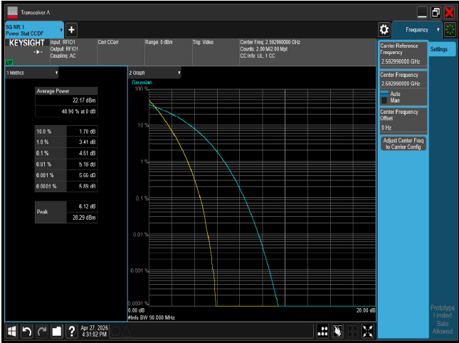
PTAR n41 90M CH518598 BPSK
