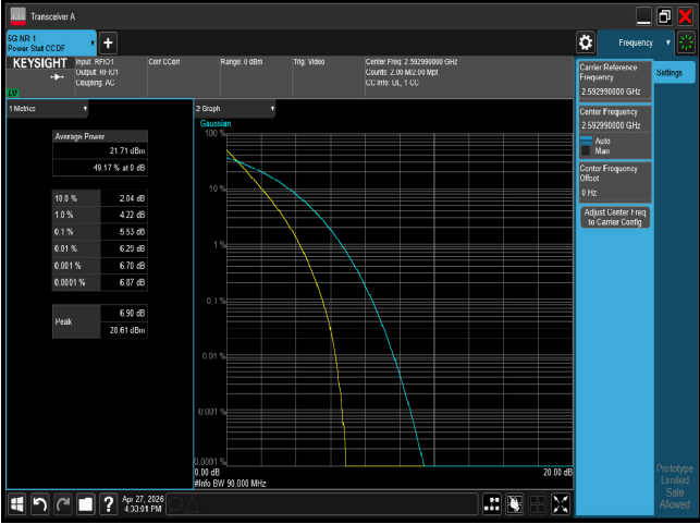
PTAR n41 90M CH518598 QPSK
