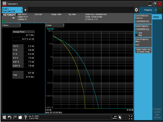
PTAR n41 90M CH518598 16QAM
