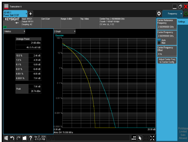
PTAR n41 70M CH518598 QPSK
