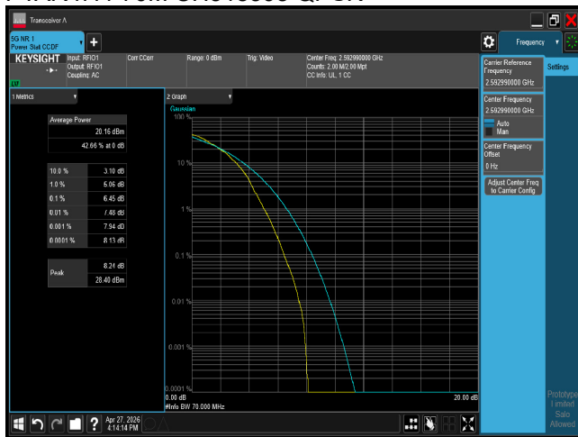
PTAR n41 70M CH518598 64QAM
