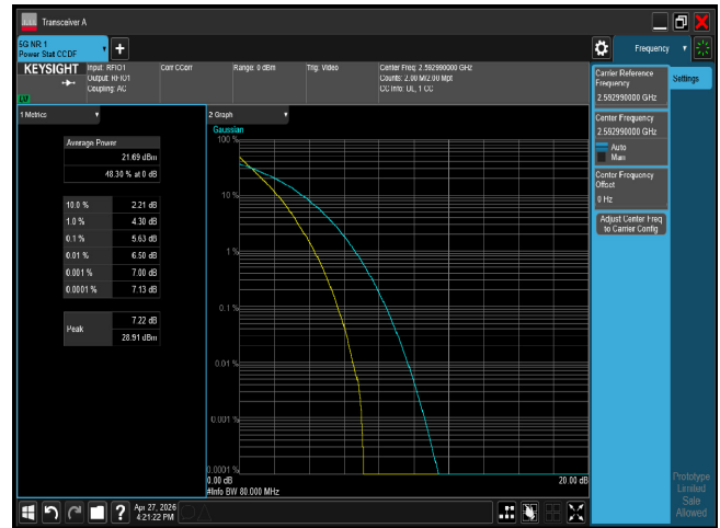
PTAR n41 80M CH518598 QPSK
