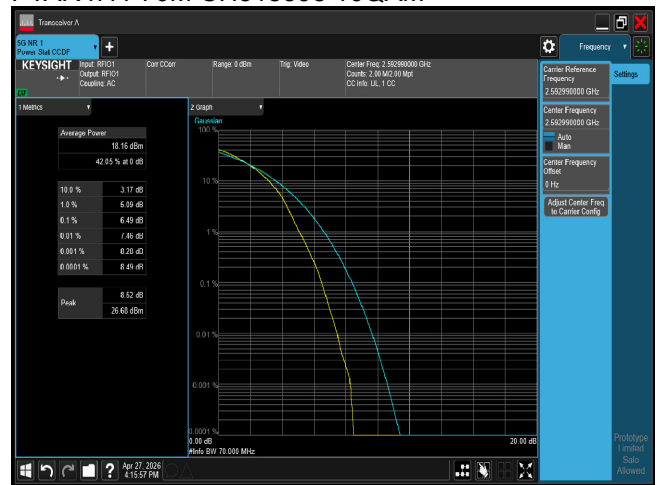
PTAR n41 70M CH518598 256QAM
