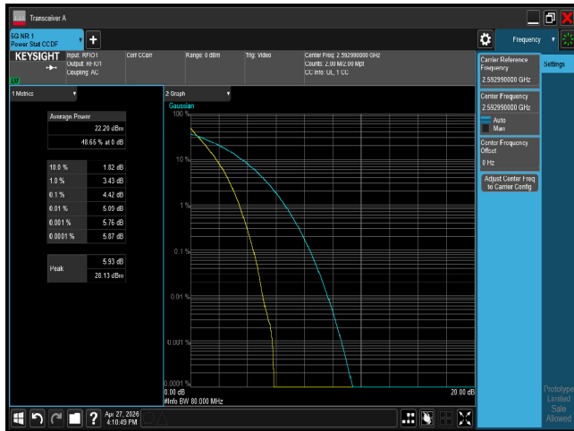
PTAR n41 80M CH518598 BPSK
