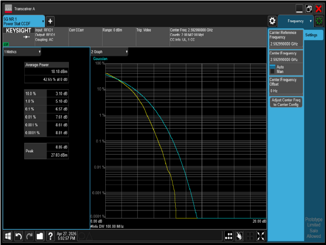
PTAR n41 100M CH518598 256QAM
