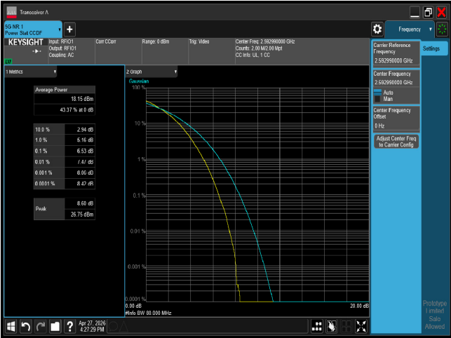
PTAR n41 80M CH518598 256QAM
