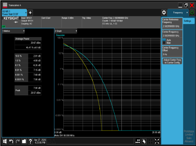
PTAR n41 80M CH518598 16QAM
