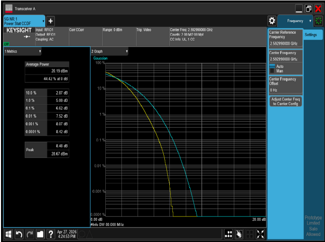
PTAR n41 80M CH518598 64QAM
