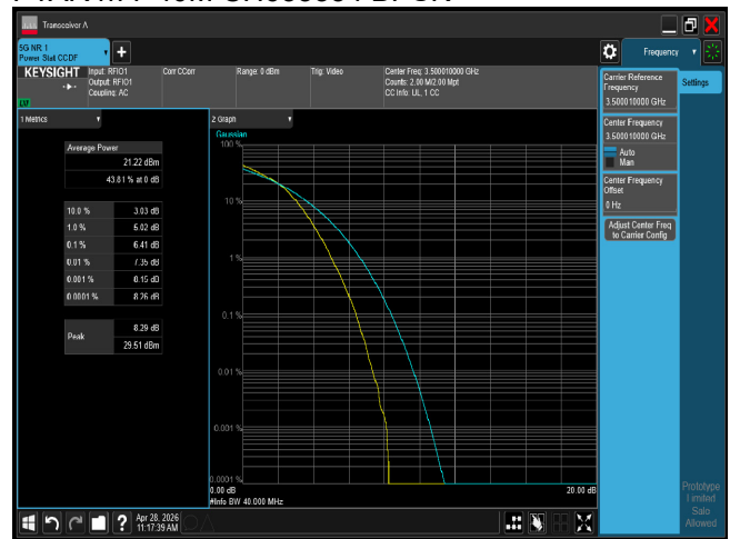
PTAR n77 40M CH633334 16QAM
