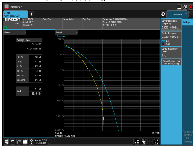
PTAR n77 15M CH633334 64QAM
