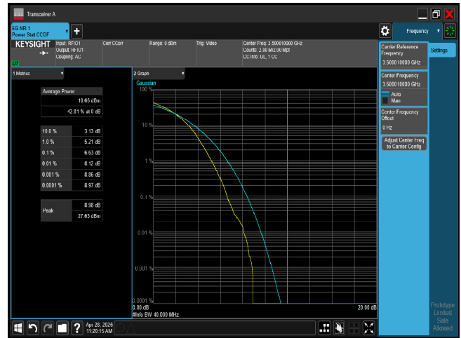
PTAR n77 40M CH633334 256QAM
