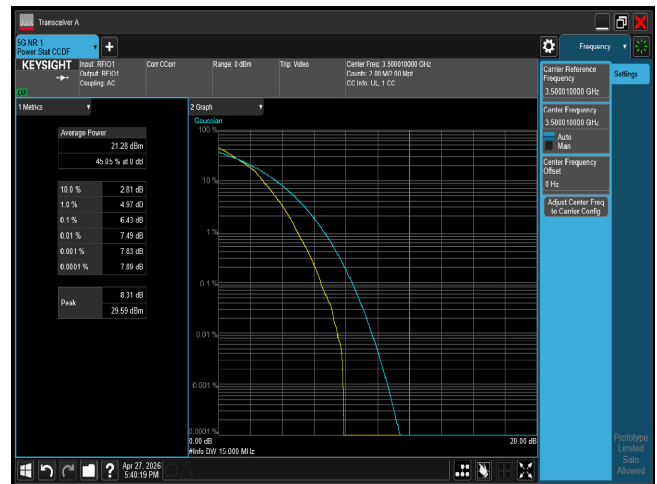
PTAR n77 15M CH633334 16QAM
