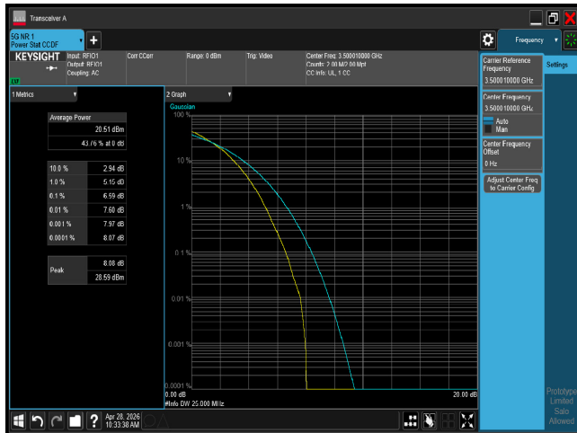
PTAR n77 25M CH633334 64QAM
