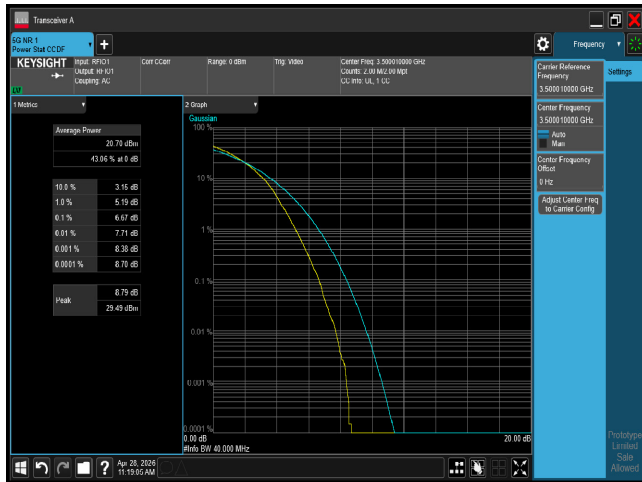
PTAR n77 40M CH633334 64QAM
