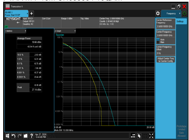
PTAR n77 15M CH633334 256QAM
