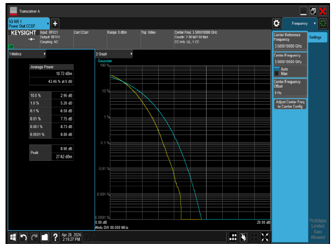
PTAR n77 80M CH633334 256QAM
