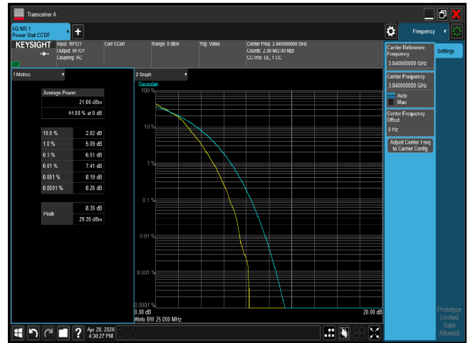
PTAR n77 25M CH656000 16QAM
