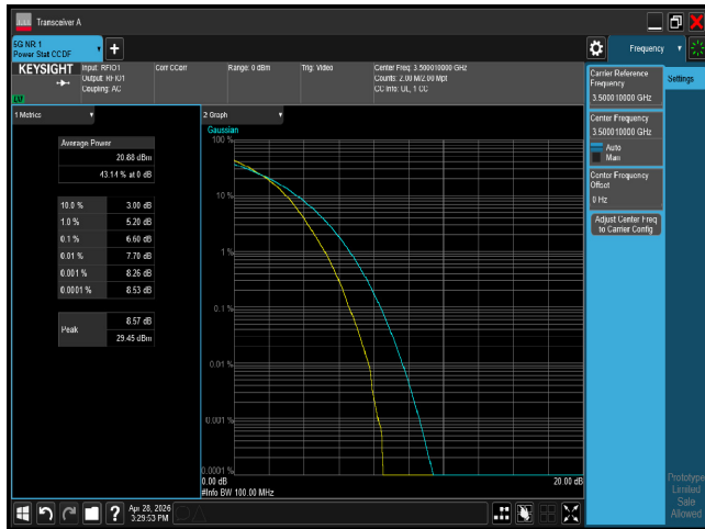
PTAR n77 100M CH633334 64QAM
