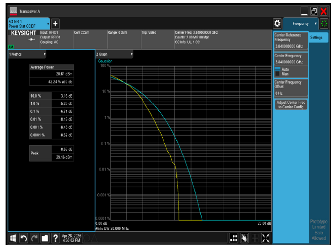
PTAR n77 20M CH656000 64QAM
