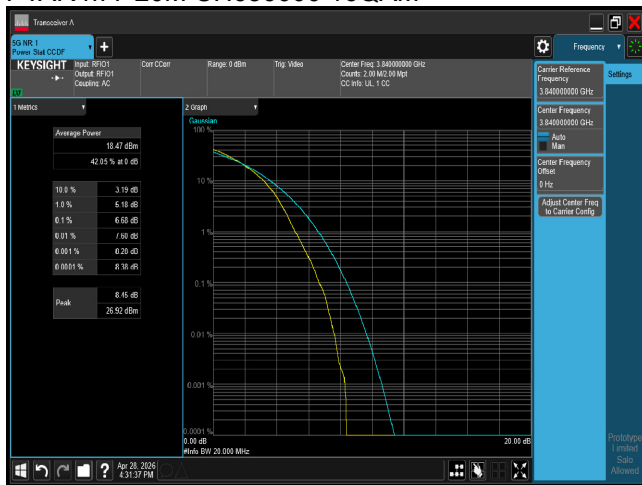
PTAR n77 20M CH656000 256QAM
