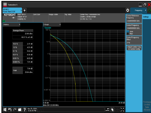
PTAR n77 25M CH656000 QPSK
