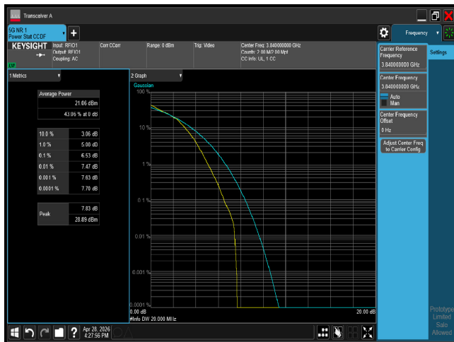
PTAR n77 20M CH656000 16QAM
