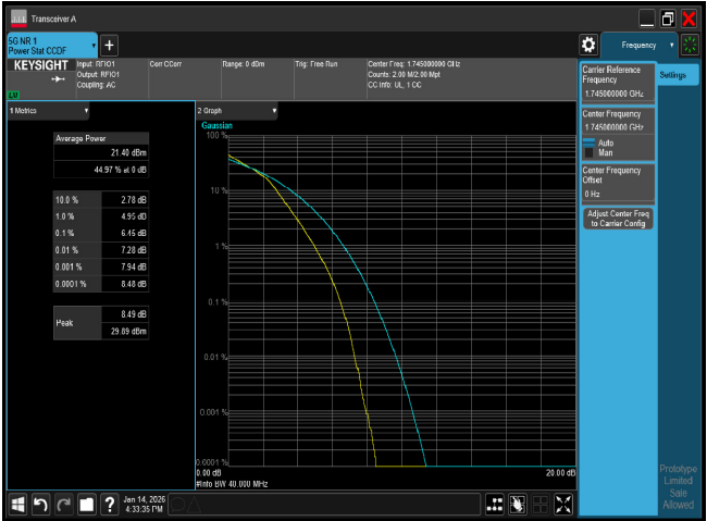
PTAR n66 40M CH349000 16QAM
