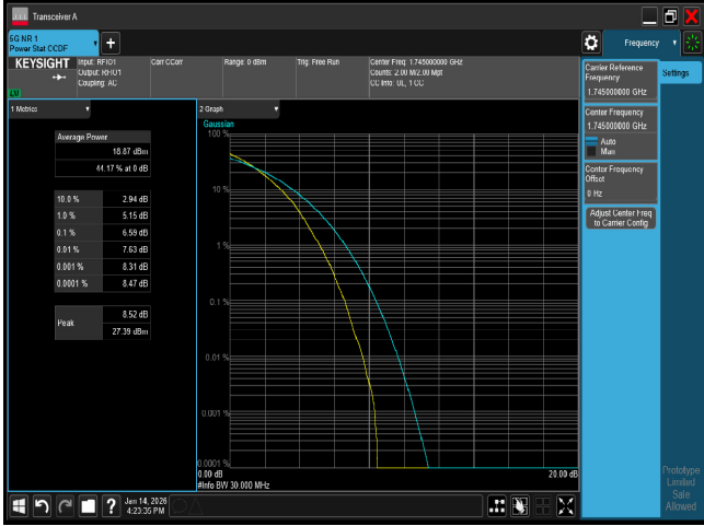
PTAR n66 30M CH349000 256QAM
