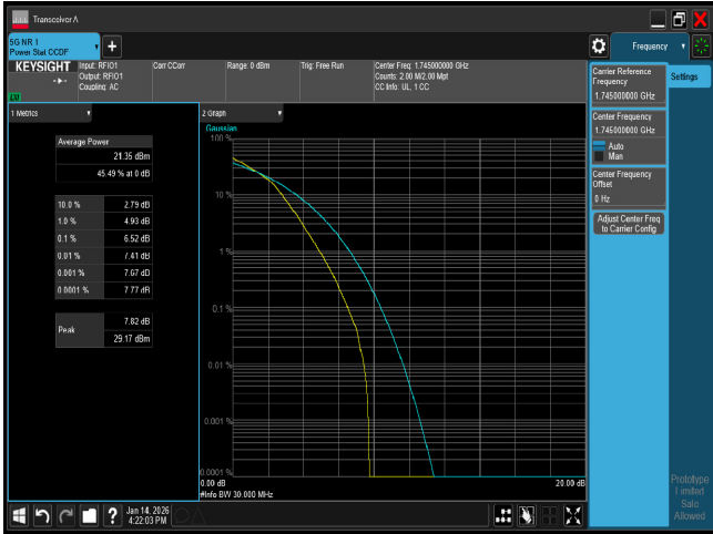
PTAR n66 30M CH349000 16QAM
