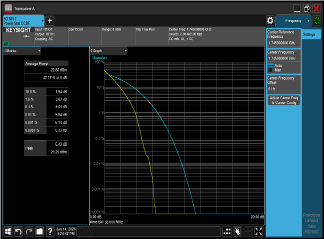
PTAR n66 35M CH349000 BPSK
