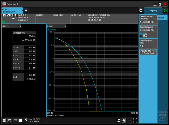
PTAR n66 35M CH349000 16QAM
