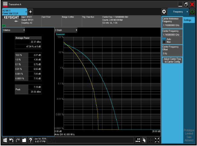
PTAR n66 45M CH349000 QPSK
