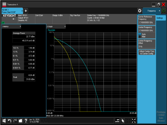
PTAR n66 25M CH349000 BPSK
