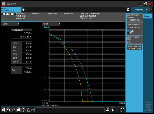
PTAR n66 35M CH349000 64QAM
