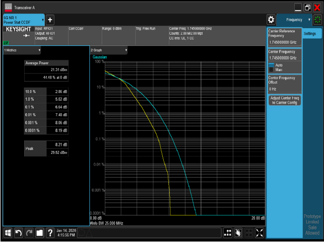
PTAR n66 25M CH349000 16QAM
