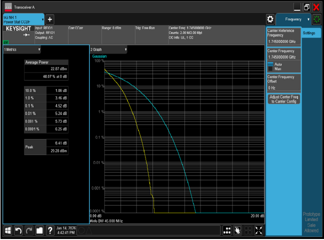
PTAR n66 45M CH349000 BPSK
