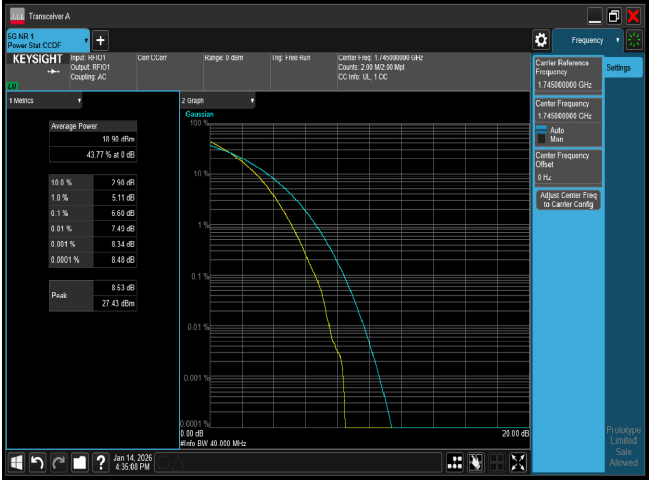
PTAR n66 40M CH349000 256QAM
