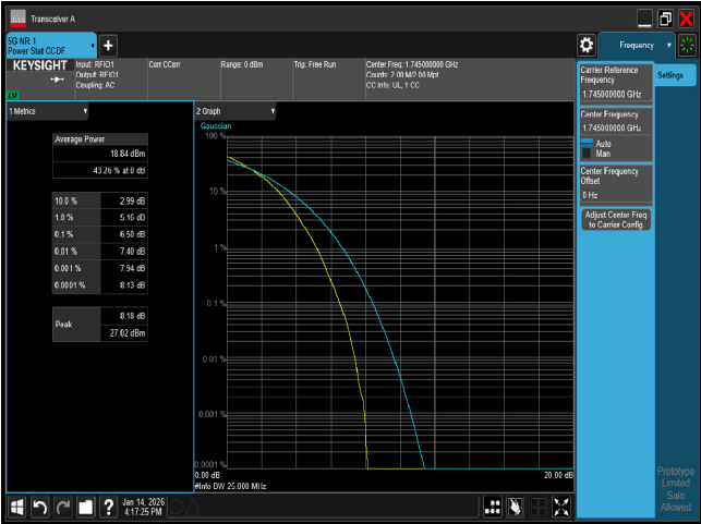
PTAR n66 25M CH349000 25QAM
