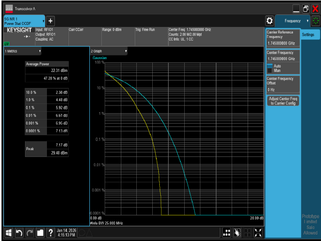
PTAR n66 25M CH349000 QPSK
