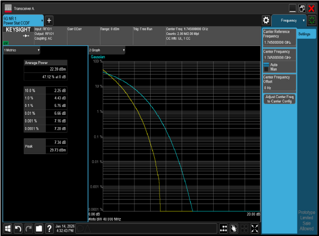
PTAR n66 40M CH349000 QPSK
