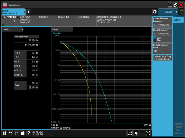
PTAR n66 30M CH349000 QPSK
