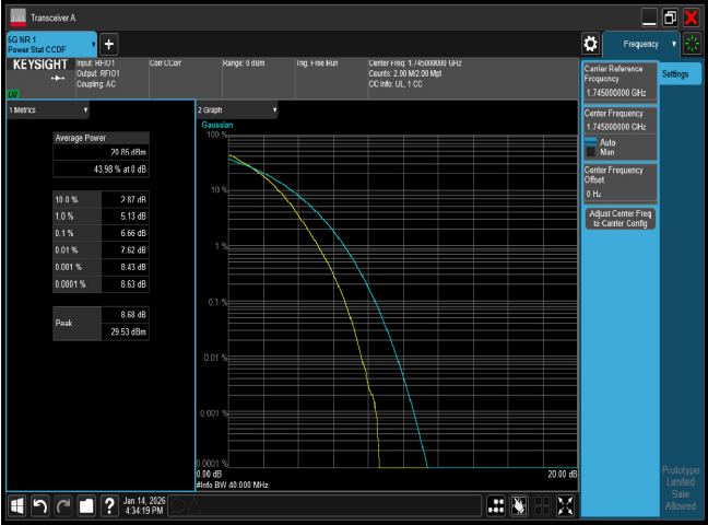
PTAR n66 40M CH349000 64QAM
