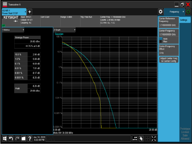
PTAR n66 30M CH349000 64QAM
