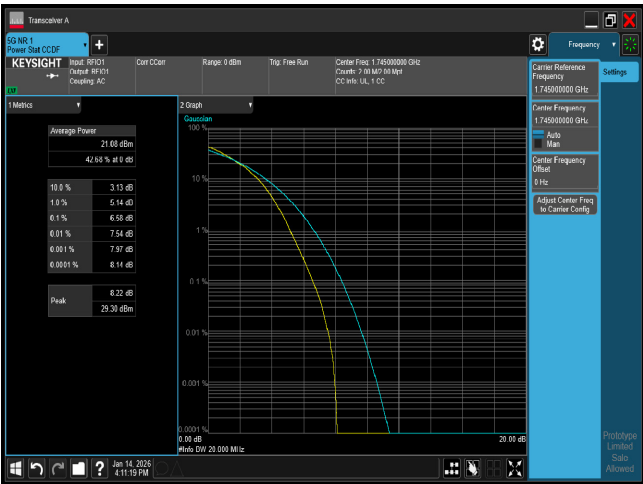
PTAR n66 20M CH349000 64QAM
