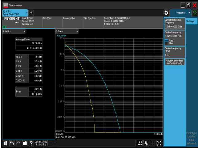
PTAR n66 30M CH349000 BPSK
