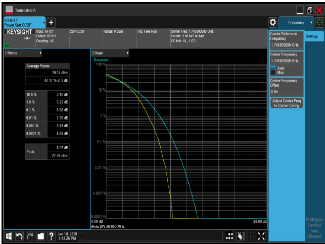
PTAR n66 20M CH349000 256QAM
