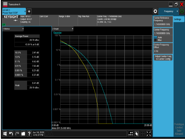
PTAR n66 25M CH349000 64QAM
