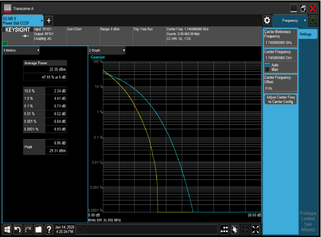
PTAR n66 35M CH349000 QPSK
