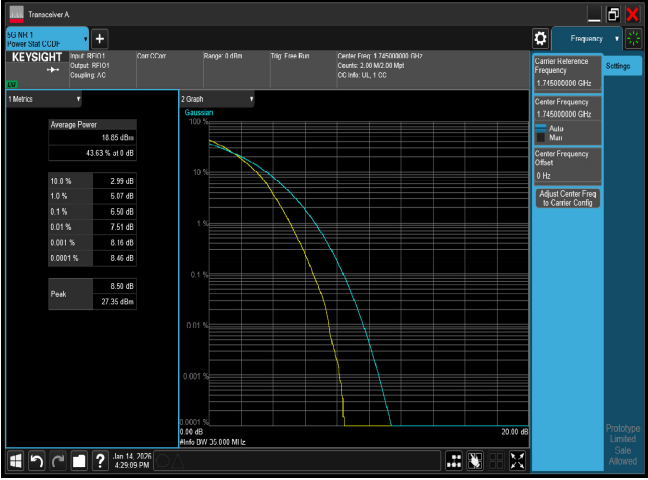
PTAR n66 35M CH349000 256QAM
