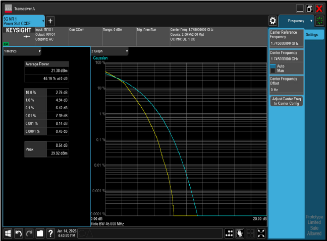
PTAR n66 45M CH349000 16QAM
