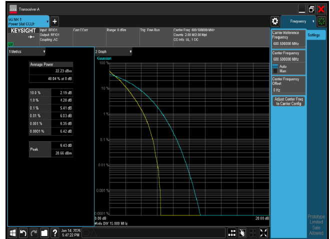
PTAR n71 15M CH136100 QPSK
