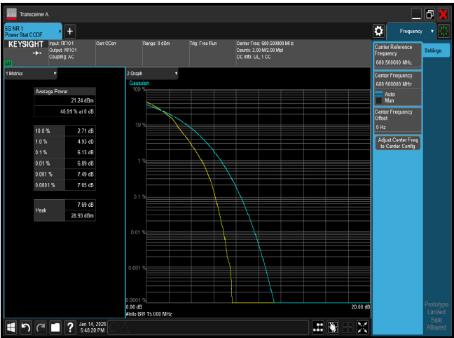
PTAR n71 15M CH136100 16QAM
