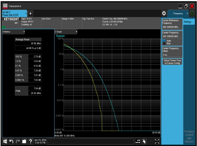
PTAR n71 15M CH136100 64QAM
