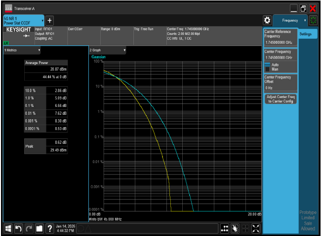
PTAR n66 45M CH349000 64QAM
