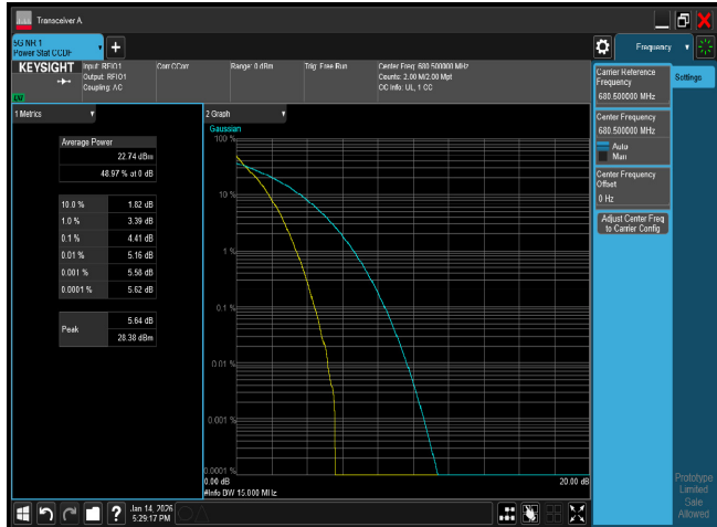
PTAR n71 15M CH136100 BPSK
