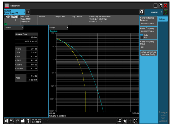
PTAR n71 10M CH136100 16QAM
