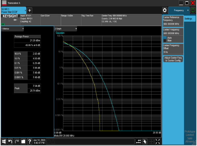
PTAR n71 20M CH136100 16QAM
