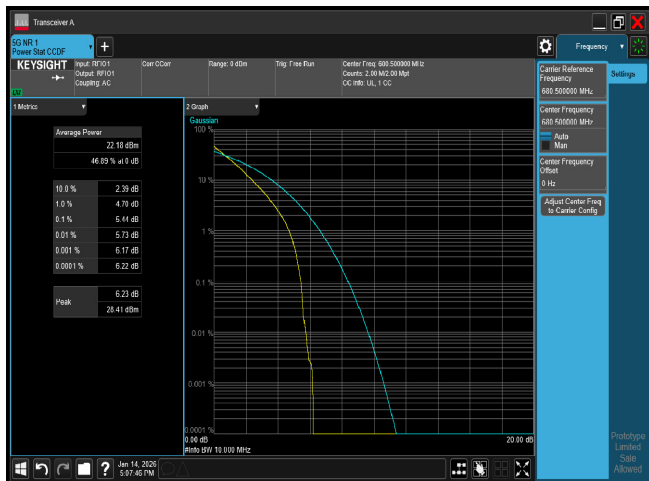
PTAR n71 10M CH136100 QPSK
