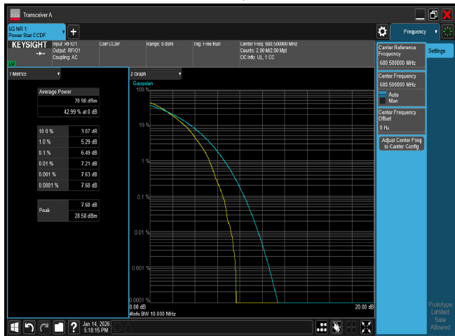
PTAR n71 10M CH136100 64QAM
