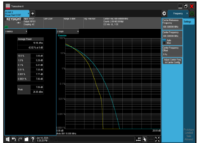
PTAR n71 10M CH136100 256QAM
