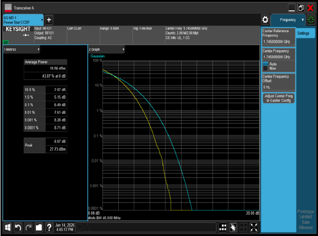
PTAR n66 45M CH349000 256QAM
