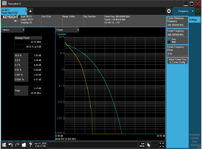
PTAR n71 20M CH136100 BPSK
