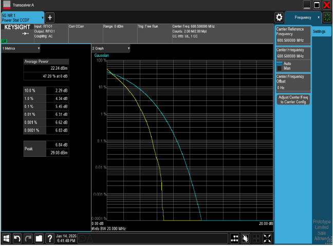
PTAR n71 20M CH136100 QPSK
