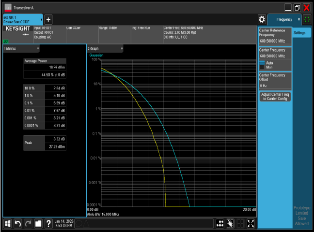
PTAR n71 15M CH136100 256QAM
