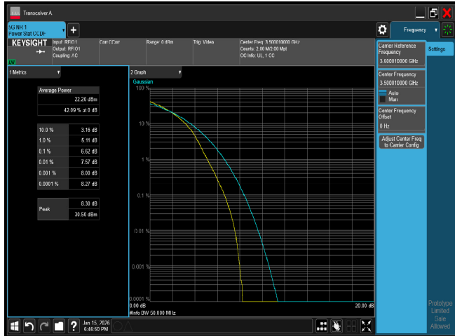
PTAR n77 50M CH633334 256QAM
