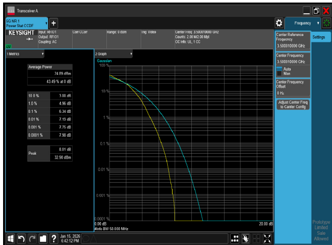
PTAR n77 50M CH633334 16QAM
