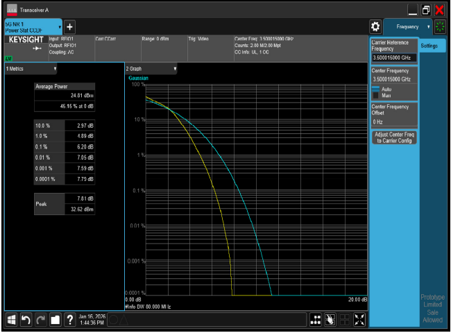
PTAR n77 80M CH633334 16QAM
