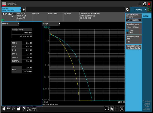
PTAR n77 100M CH633334 16QAM
