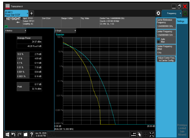
PTAR B77 15M CH656000 16QAM
