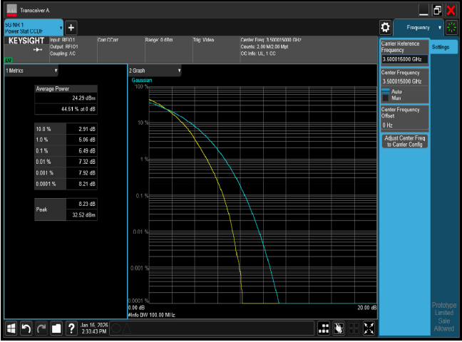
PTAR n77 100M CH633334 64QAM
