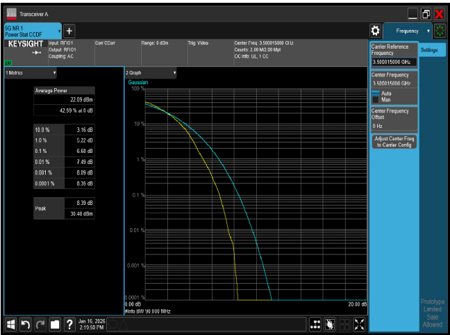
PTAR n77 90M CH633334 256QAM
