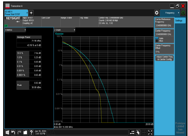
PTAR B77 15M CH656000 256QAM
