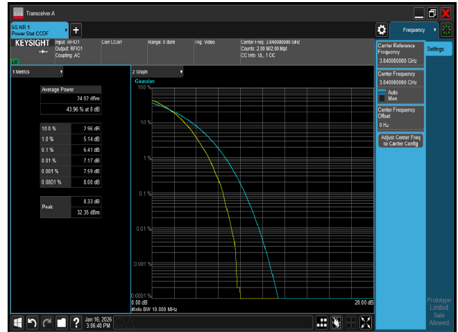
PTAR B77 10M CH656000 64QAM
