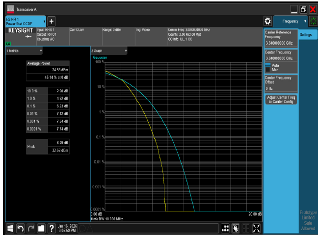
PTAR B77 10M CH656000 16QAM
