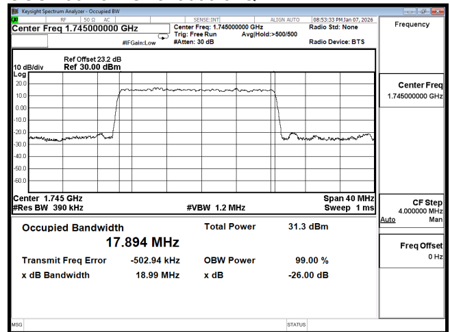
OCC n66 20M CH349000 BPSK
