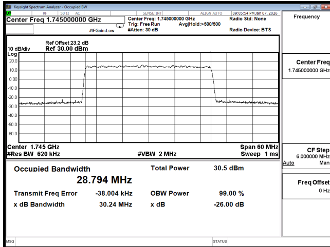
OCC n66 30M CH349000 QPSK
