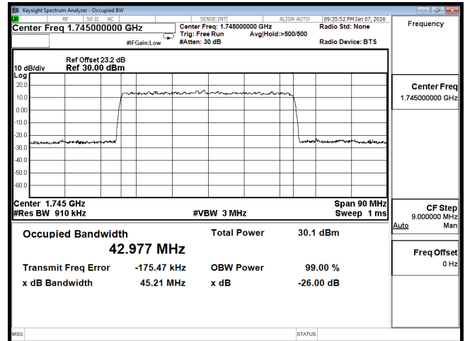
OCC n66 45M CH349000 QPSK
