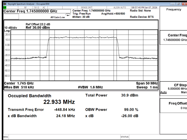
OCC n66 25M CH349000 BPSK
