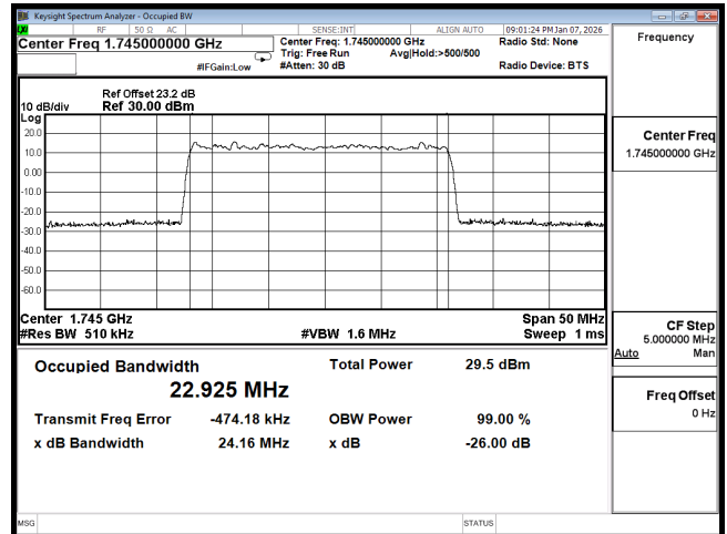
OCC n66 25M CH349000 64QAM
