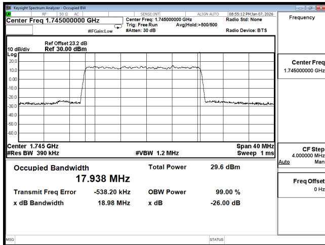
OCC n66 20M CH349000 64QAM
