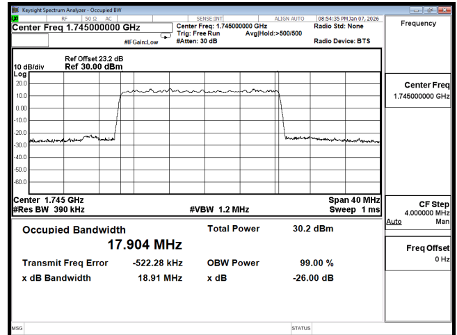
OCC n66 20M CH349000 16QAM
