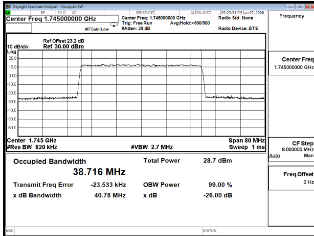
OCC n66 40M CH349000 64QAM
