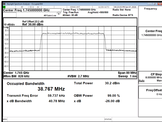
OCC n66 40M CH349000 QPSK
