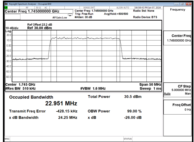
OCC n66 25M CH349000 QPSK
