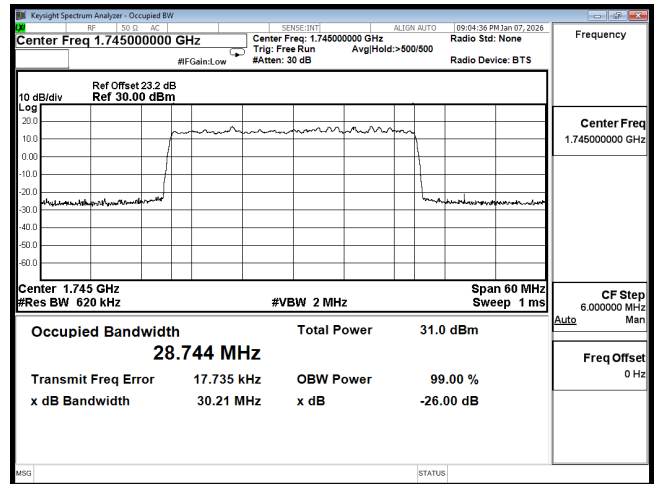
OCC n66 30M CH349000 BPSK
