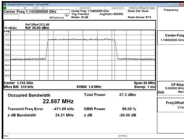
OCC n66 25M CH349000 256QAM
