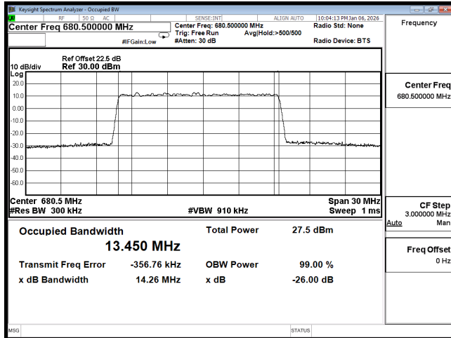
OCC n71 15M CH136100 256QAM
