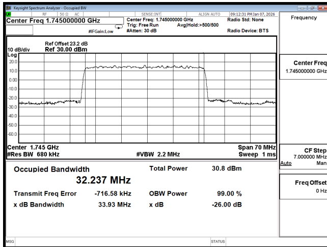
OCC n66 35M CH349000 BPSK
