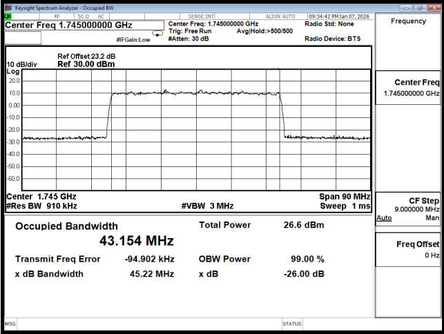
OCC n66 45M CH349000 256QAM
