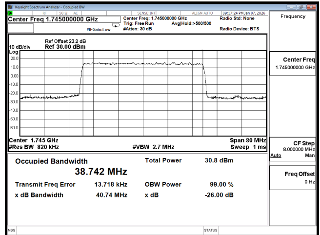
OCC n66 40M CH349000 BPSK
