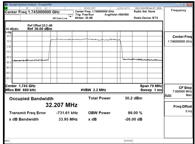
OCC n66 35M CH349000 QPSK
