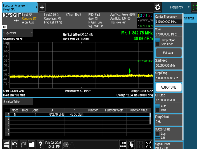
CSE n7 50M CH505000 BPSK(1,1)
