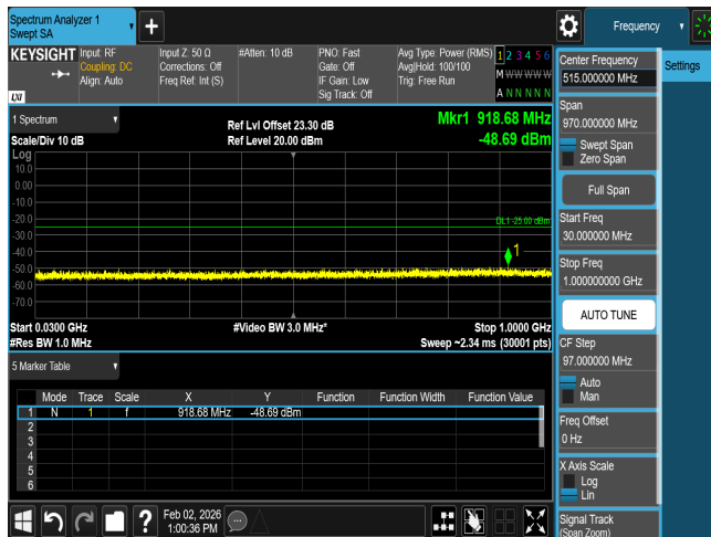
CSE n7 40M CH504000 BPSK(1,1)
