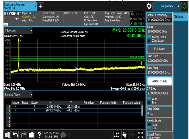
CSE n7 40M CH510000 BPSK(1,1)_
