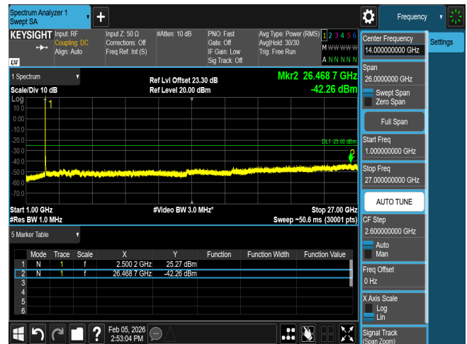
CSE n7 30M CH503000 BPSK(1,1)
