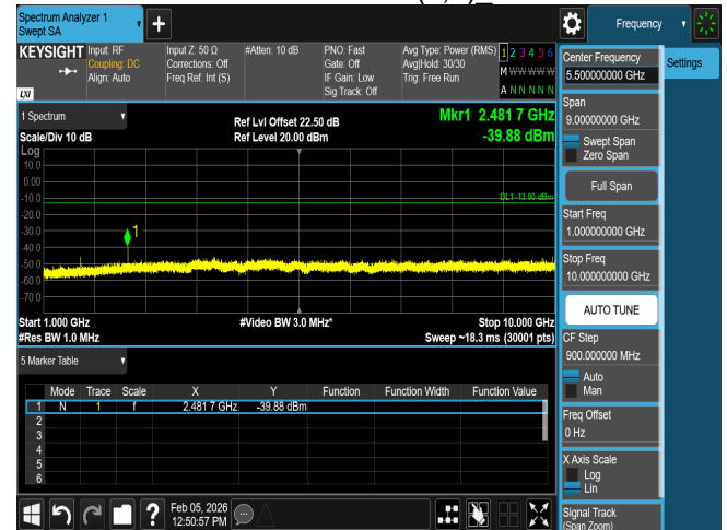
CSE n5 20M CH167300 BPSK(1,1)
