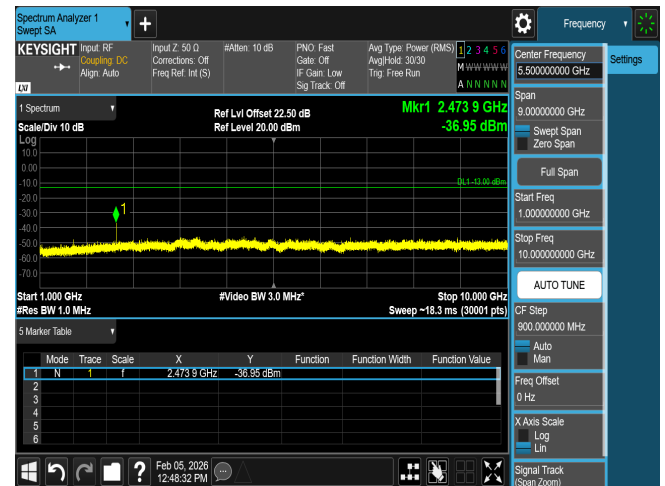
CSE n5 20M CH166800 BPSK(1,1)
