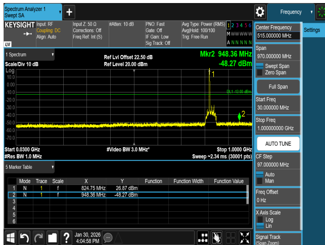
CSE n5 20M CH166800 BPSK(1,1)
