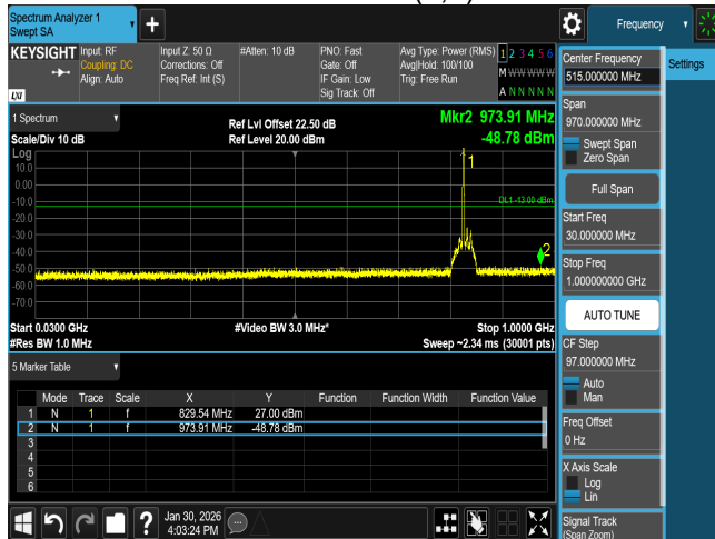
CSE n5 15M CH167300 BPSK(1,1)
