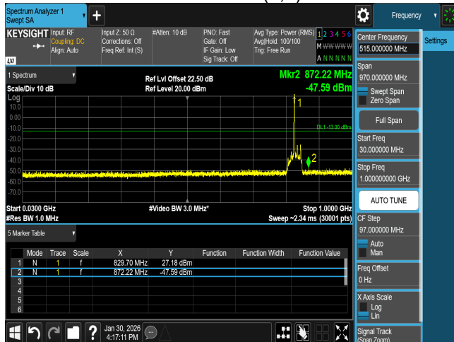
CSE n5 20M CH167800 BPSK(1,1)
