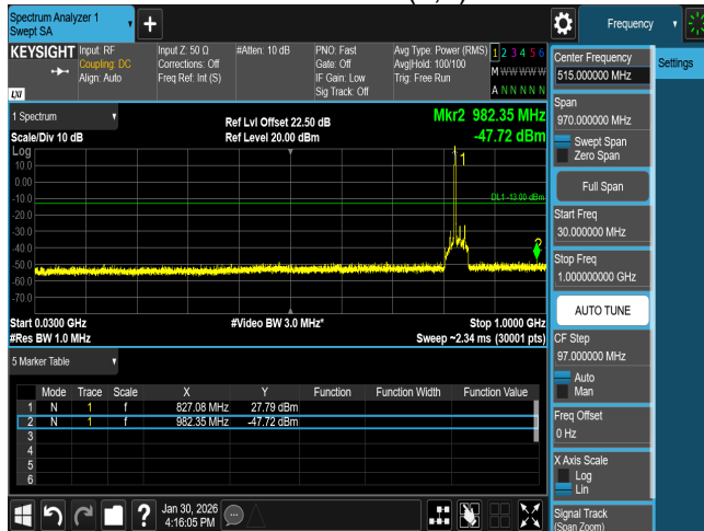
CSE n5 20M CH167300 BPSK(1,1)
