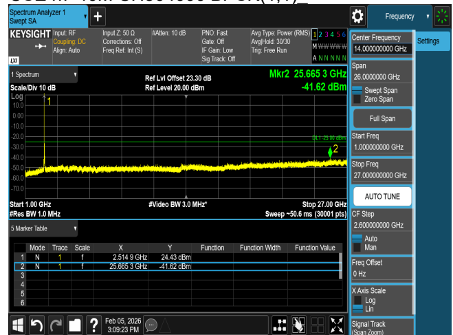
CSE n7 40M CH507000 BPSK(1,1)
