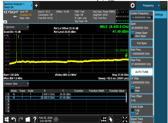
CSE n7 25M CH511500 BPSK(1,1)_
