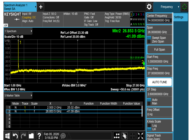
CSE n7 50M CH505000 BPSK(1,1)
