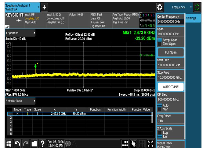
CSE n5 15M CH166300 BPSK(1,1)
