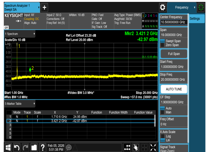
CSE n66 20M CH344000 BPSK(1,1)
