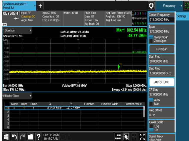
CSE n66 25M CH353500 BPSK(1,1)
