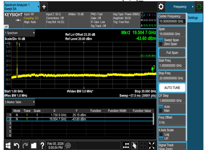
CSE n66 30M CH349000 BPSK(1,1)
