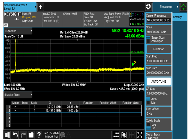
CSE n66 15M CH343500 BPSK(1,1)
