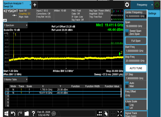
CSE n66 20M CH354000 BPSK(1,1)_
