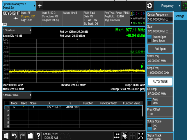
CSE n66 10M CH355000 BPSK(1,1)
