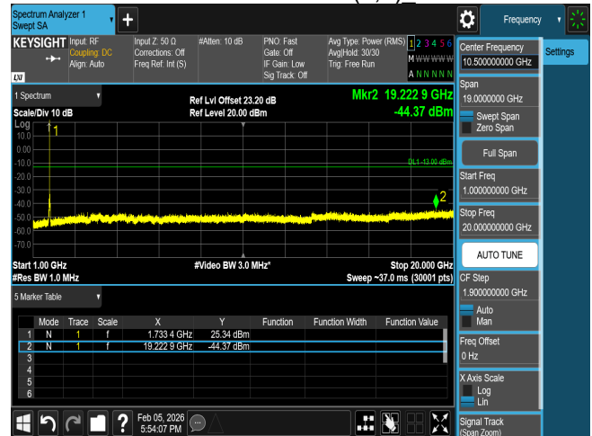
CSE n66 25M CH349000 BPSK(1,1)
