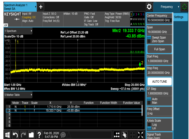
CSE n66 10M CH343000 BPSK(1,1)
