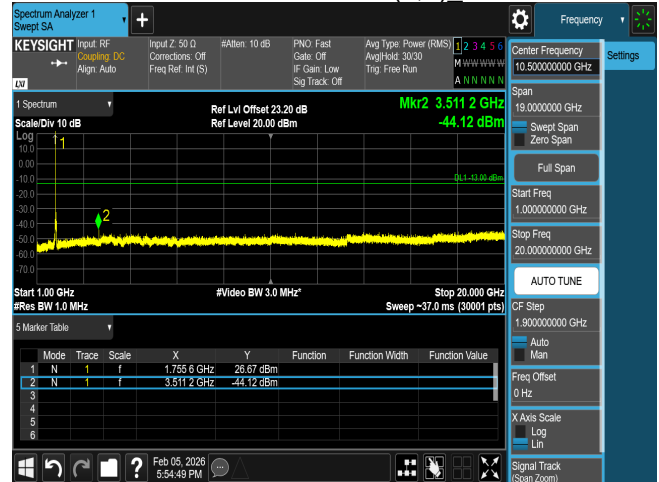
CSE n66 25M CH353500 BPSK(1,1)_
