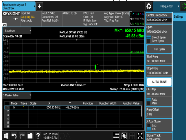
CSE n66 25M CH349000 BPSK(1,1)
