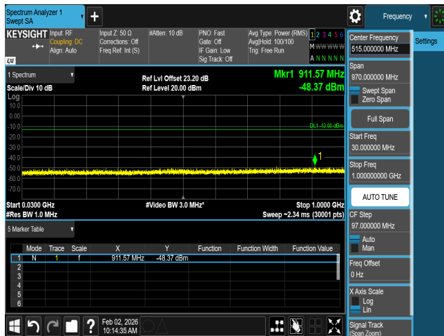
CSE n66 25M CH344500 BPSK(1,1)
