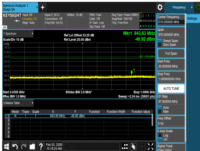
CSE n66 30M CH345000 BPSK(1,1)
