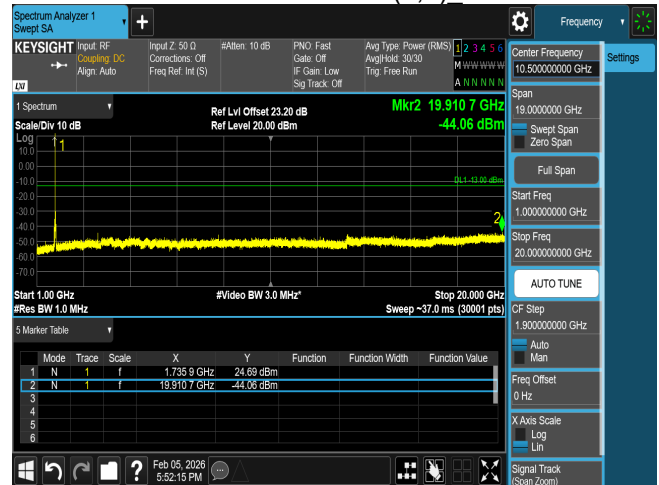
CSE n66 20M CH349000 BPSK(1,1)
