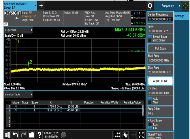
CSE n66 10M CH355000 BPSK(1,1)_
