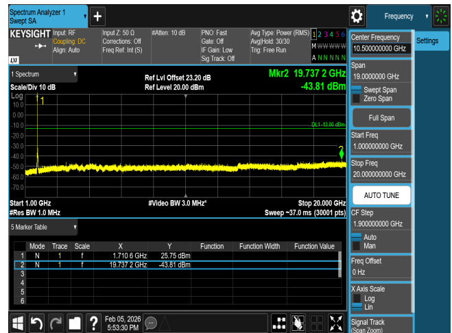
CSE n66 25M CH344500 BPSK(1,1)
