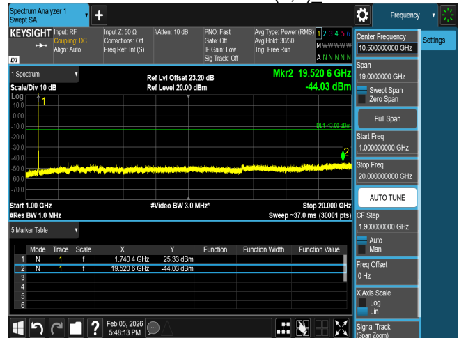
CSE n66 10M CH349000 BPSK(1,1)
