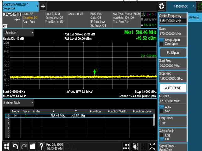
CSE n66 20M CH354000 BPSK(1,1)
