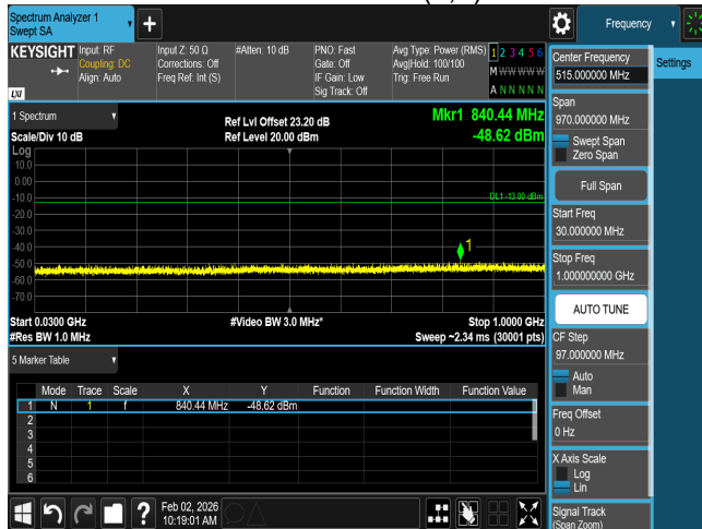
CSE n66 30M CH349000 BPSK(1,1)
