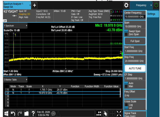
CSE n66 15M CH354500 BPSK(1,1)_
