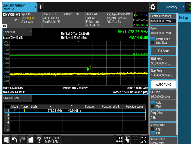
CSE n66 10M CH343000 BPSK(1,1)
