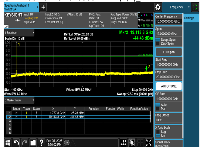
CSE n66 15M CH349000 BPSK(1,1)
