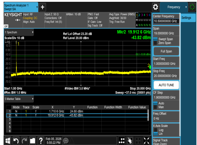
CSE n66 30M CH345000 BPSK(1,1)
