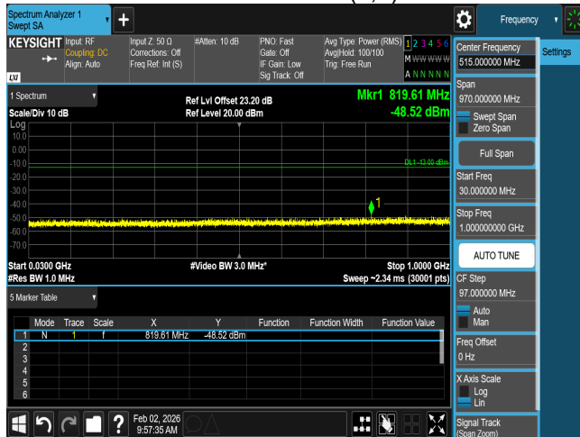
CSE n66 10M CH349000 BPSK(1,1)
