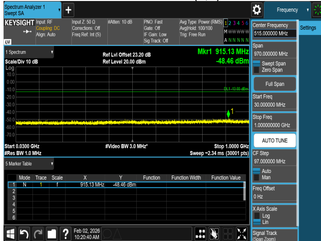
CSE n66 30M CH353000 BPSK(1,1)
