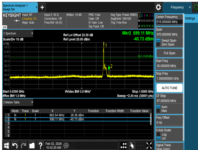
CSE n71 10M CH133600 BPSK(1,1)
