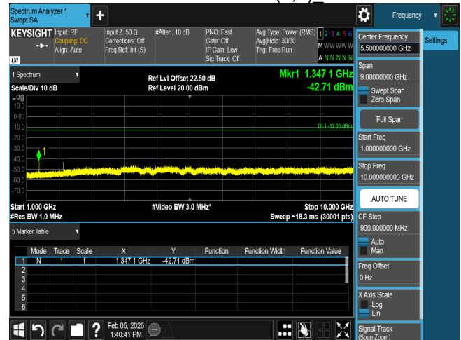
CSE n71 15M CH136100 BPSK(1,1)
