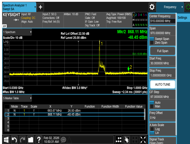
CSE n71 20M CH134600 BPSK(1,1)
