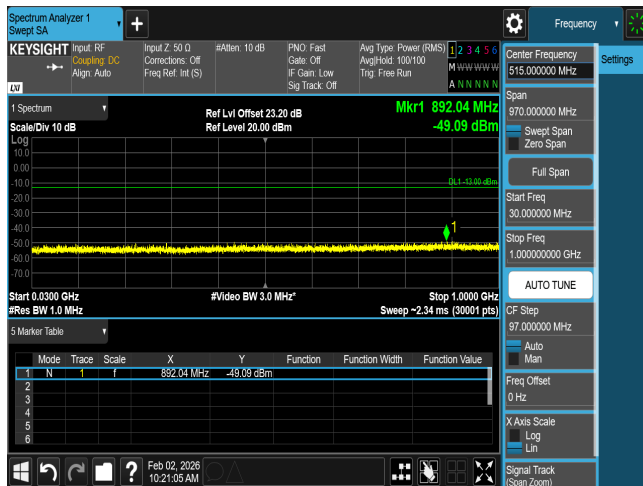
CSE n66 35M CH345500 BPSK(1,1)
