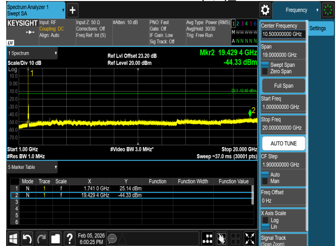
CSE n66 40M CH352000 BPSK(1,1)_
