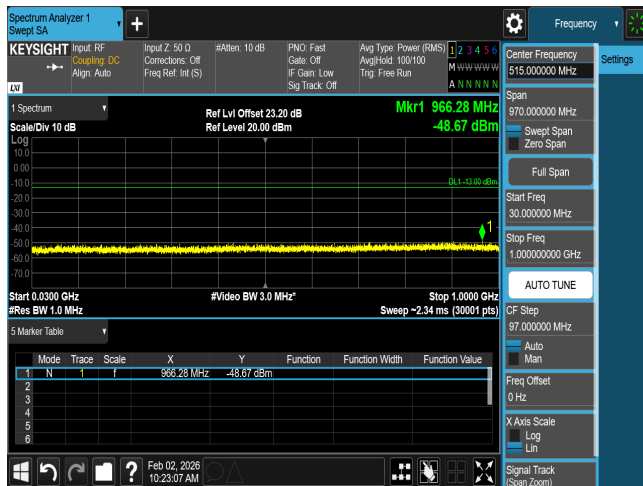
CSE n66 40M CH346000 BPSK(1,1)
