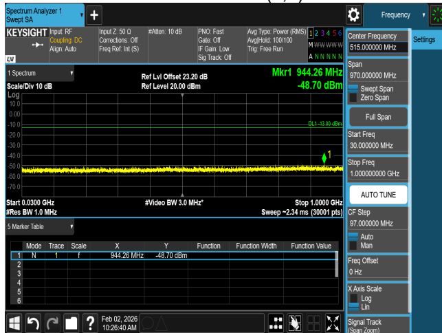
CSE n66 45M CH349000 BPSK(1,1)
