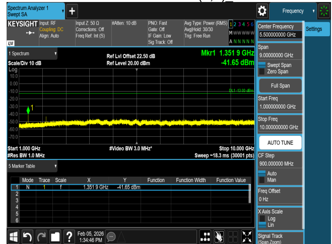
CSE n71 10M CH136100 BPSK(1,1)
