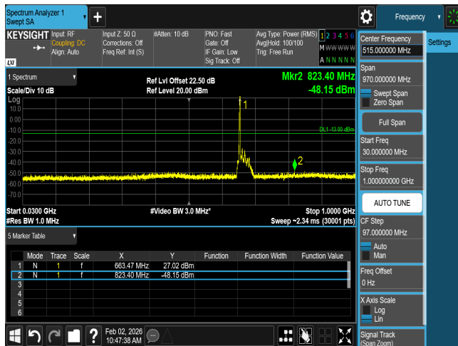
CSE n71 15M CH134100 BPSK(1,1)
