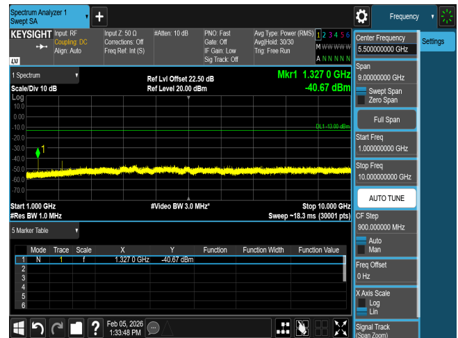
CSE n71 10M CH133600 BPSK(1,1)
