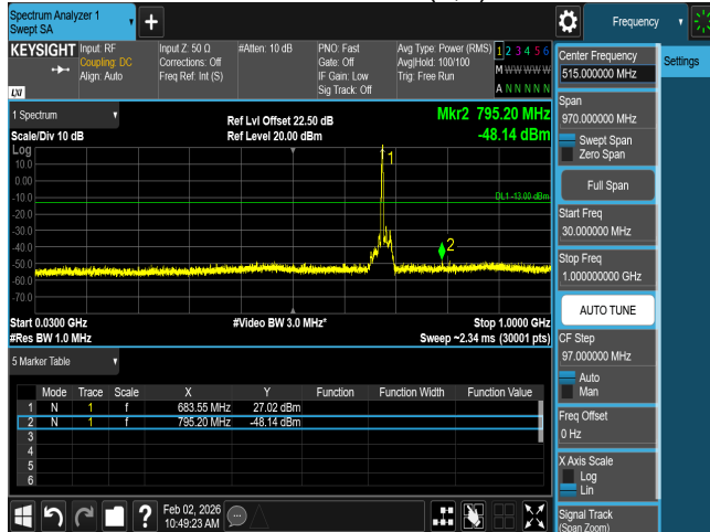
CSE n71 15M CH138100 BPSK(1,1)
