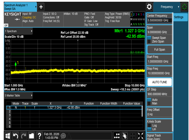
CSE n71 20M CH134600 BPSK(1,1)
