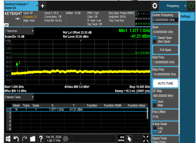
CSE n71 10M CH138600 BPSK(1,1)_
