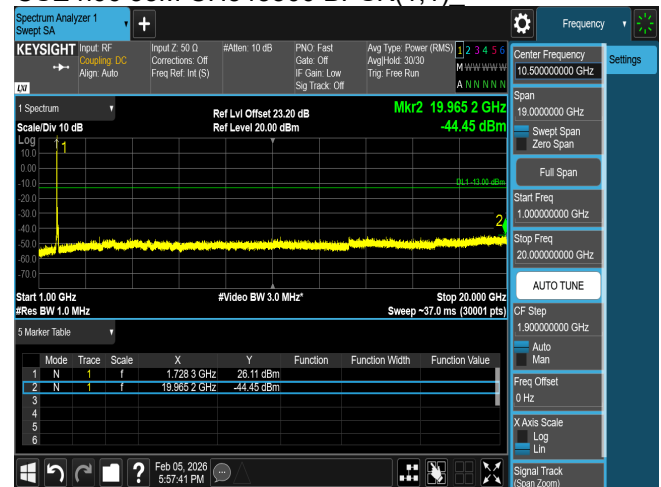
CSE n66 35M CH345500 BPSK(1,1)
