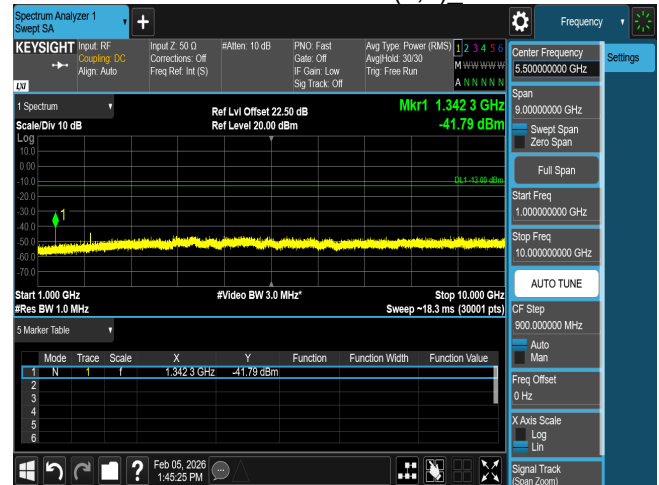
CSE n71 20M CH136100 BPSK(1,1)
