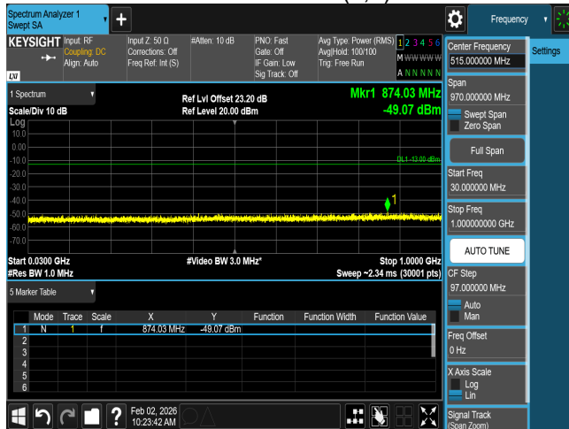
CSE n66 40M CH349000 BPSK(1,1)
