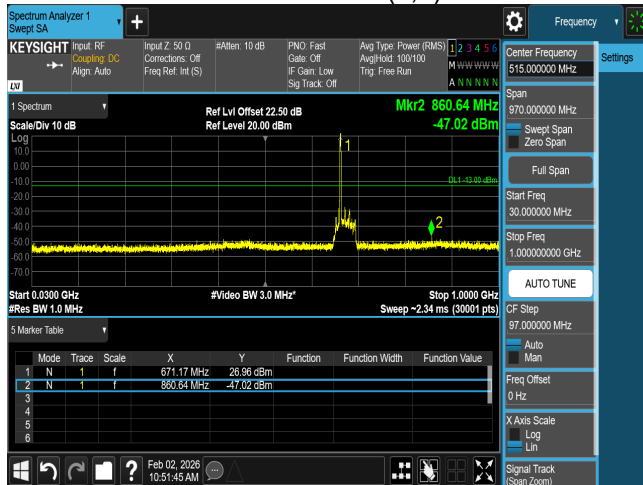
CSE n71 20M CH136100 BPSK(1,1)
