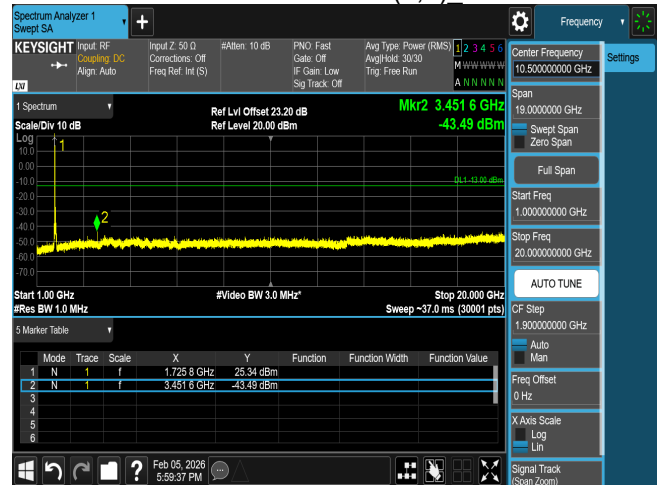
CSE n66 40M CH349000 BPSK(1,1)
