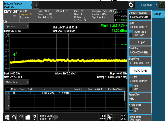
CSE n71 15M CH138100 BPSK(1,1)_
