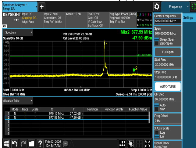
CSE n71 10M CH136100 BPSK(1,1)
