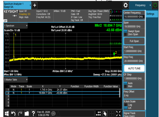
CSE n66 35M CH349000 BPSK(1,1)_
