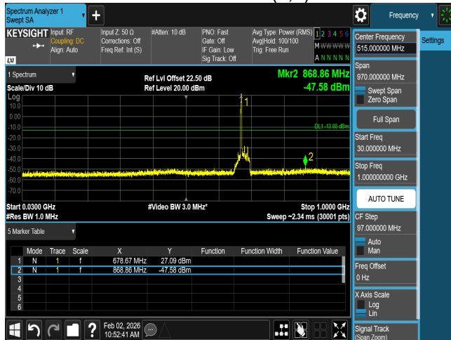
CSE n71 20M CH137600 BPSK(1,1)
