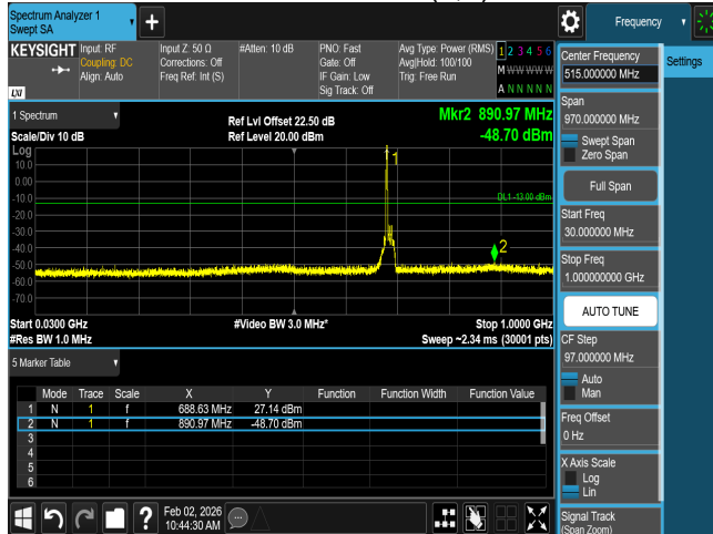
CSE n71 10M CH138600 BPSK(1,1)
