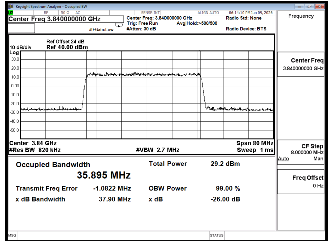
OCC n77 40M CH656000 16QAM
