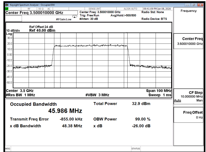
OCC n77 50M CH633334 QPSK
