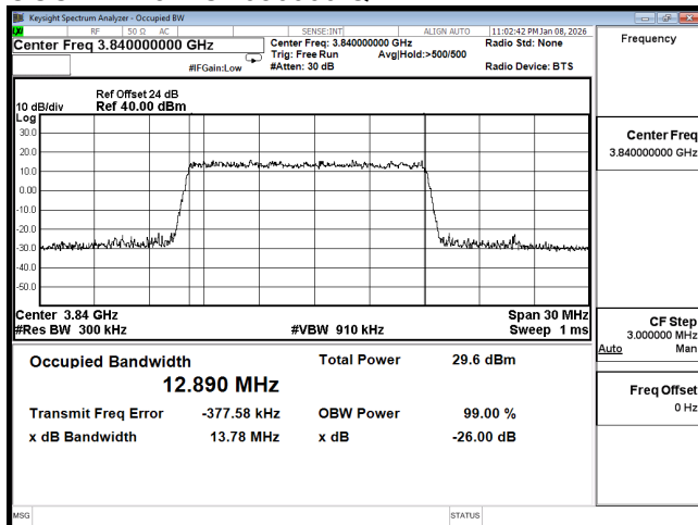
OCC n77 15M CH656000 64QAM
