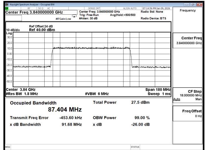
OCC n77 90M CH656000 64QAM
