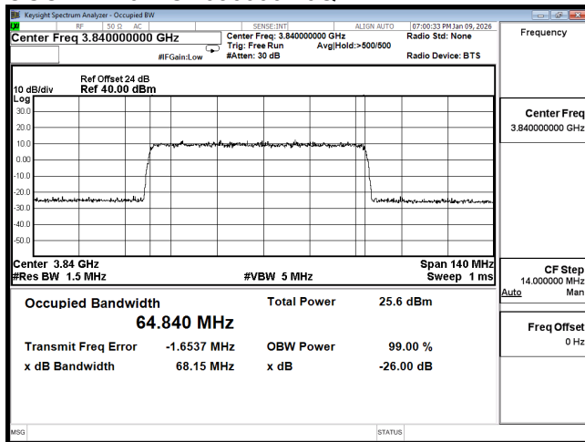
OCC n77 70M CH656000 256QAM
