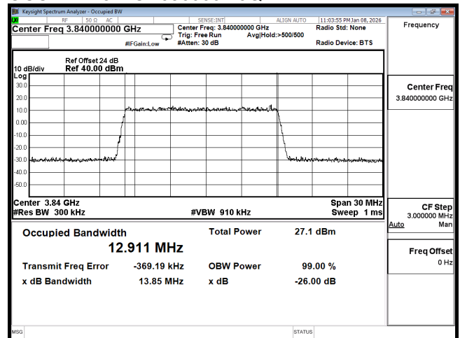
OCC n77 15M CH656000 256QAM
