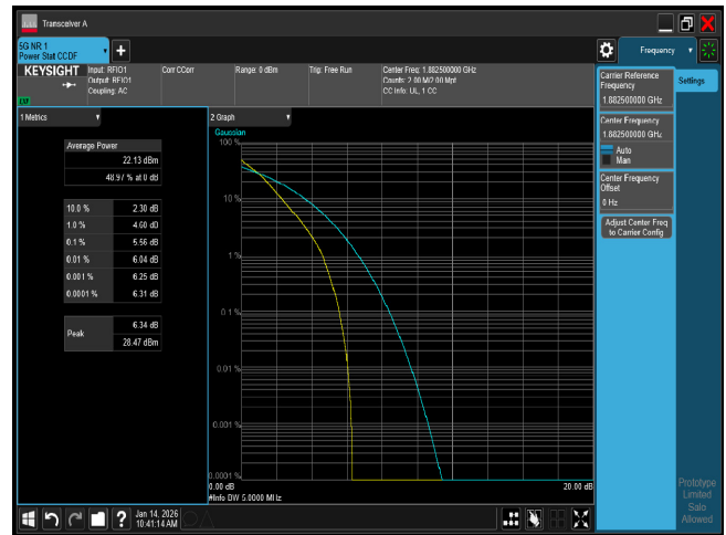
PTAR n25 5M CH376500 QPSK
