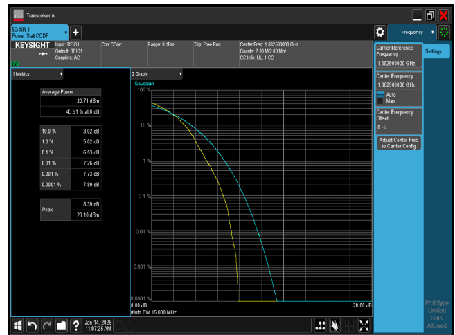
PTAR n25 15M CH376500 64QAM
