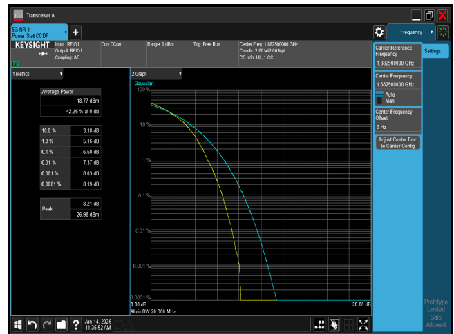
PTAR n25 20M CH376500 256QAM
