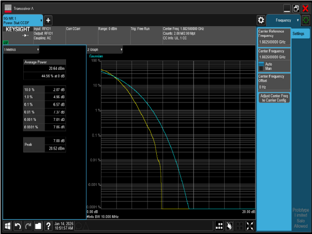
PTAR n25 10M CH376500 64QAM
