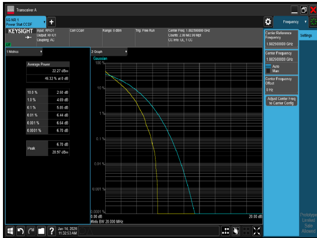
PTAR n25 20M CH376500 QPSK
