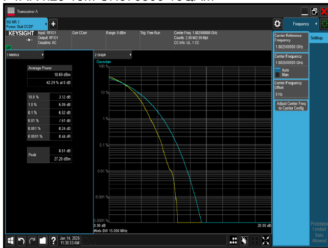
PTAR n25 15M CH376500 256QAM
