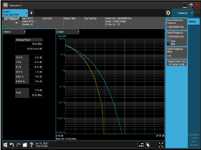
PTAR n25 10M CH376500 256QAM
