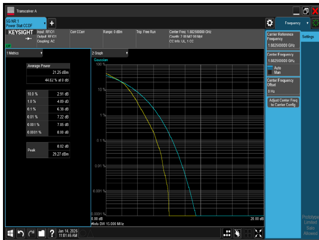
PTAR n25 15M CH376500 16QAM
