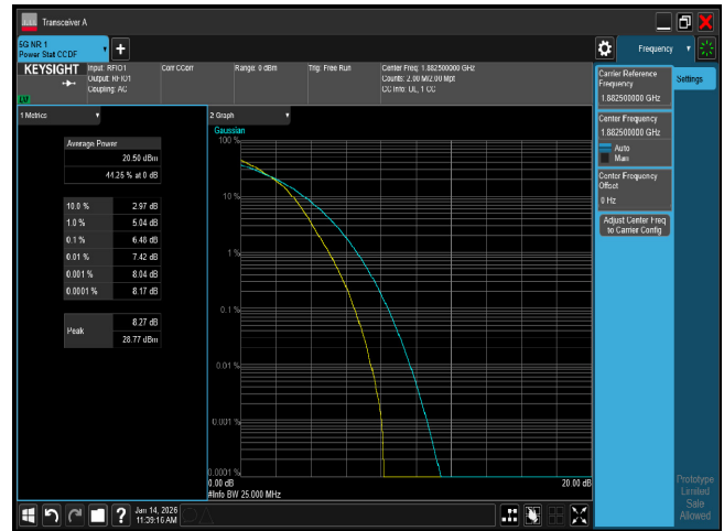
PTAR n25 25M CH376500 64QAM
