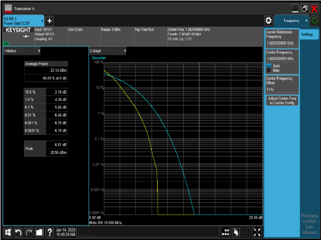
PTAR n25 10M CH376500 QPSK
