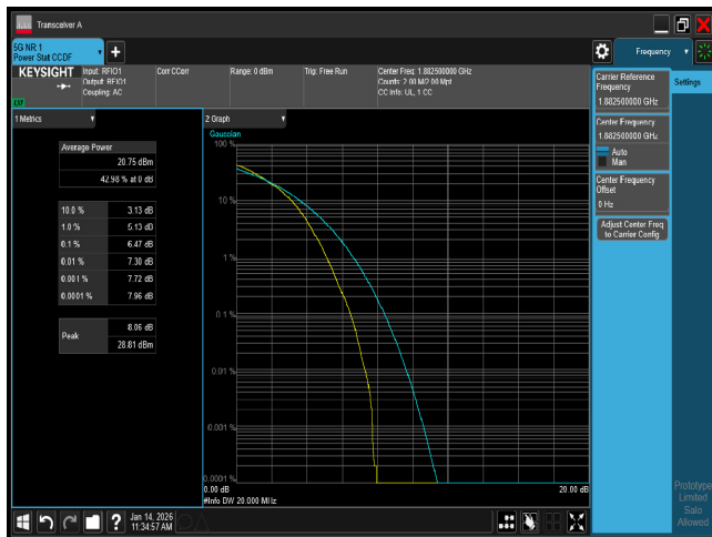
PTAR n25 20M CH376500 64QAM
