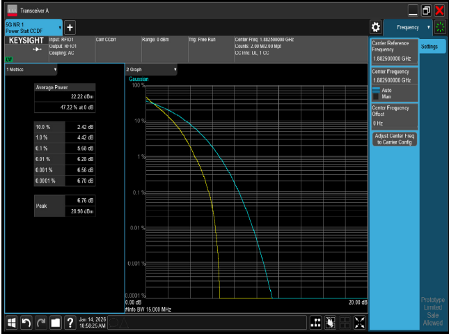
PTAR n25 15M CH376500 QPSK
