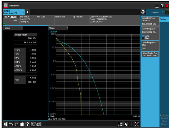
PTAR n25 5M CH376500 BPSK
