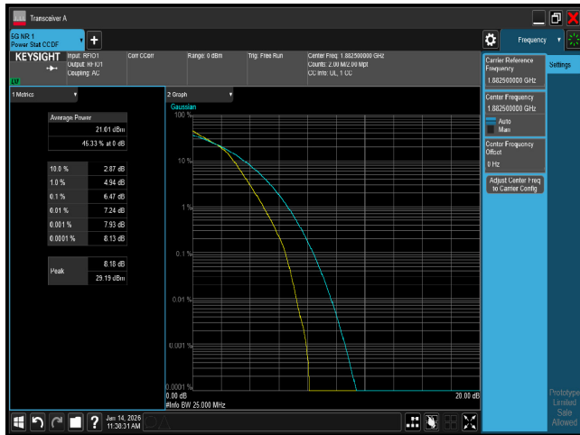
PTAR n25 25M CH376500 16QAM
