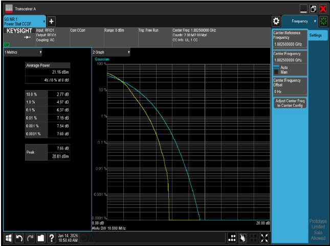
PTAR n25 10M CH376500 16QAM
