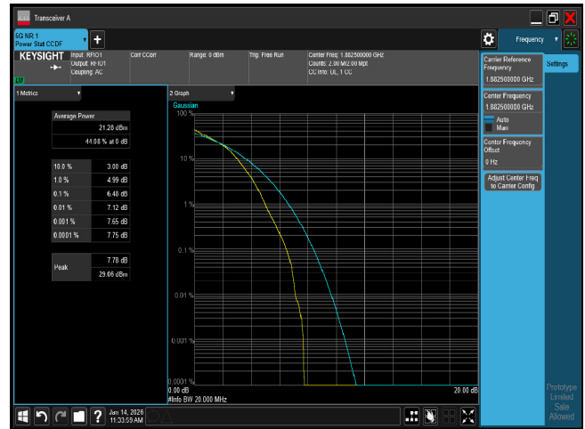
PTAR n25 20M CH376500 16QAM
