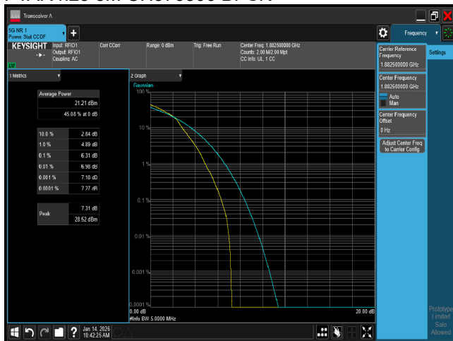
PTAR n25 5M CH376500 16QAM
