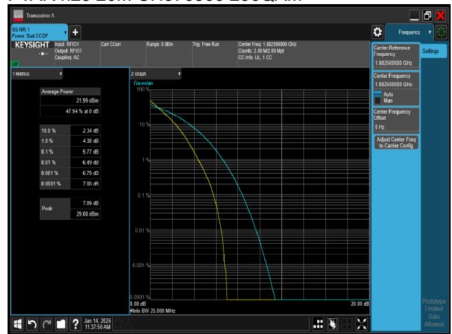
PTAR n25 25M CH376500 QPSK
