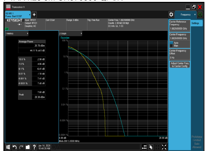
PTAR n25 5M CH376500 64QAM
