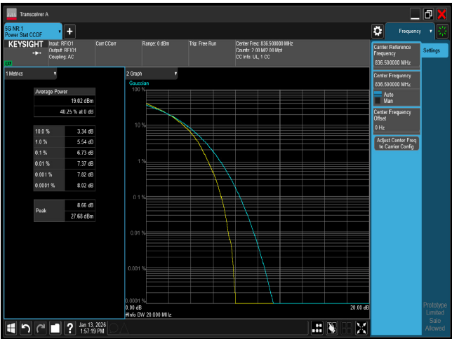
PTAR n5 20M CH167300 64QAM
