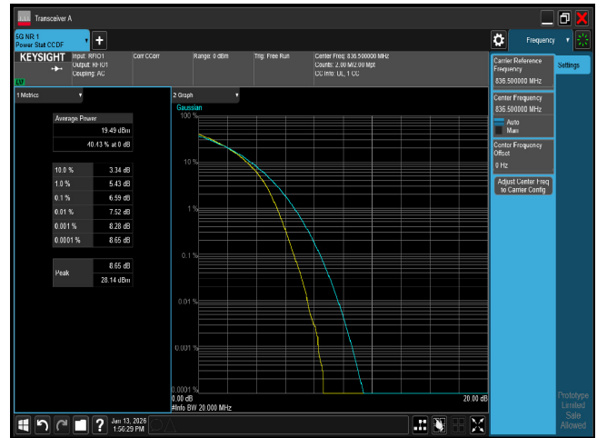
PTAR n5 20M CH167300 16QAM
