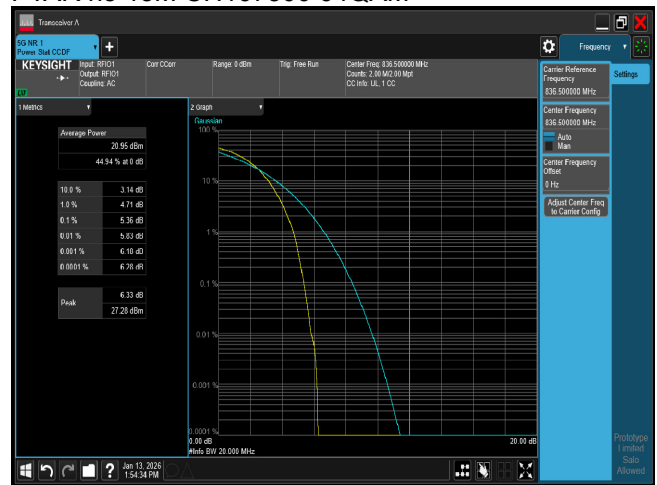
PTAR n5 20M CH167300 BPSK
