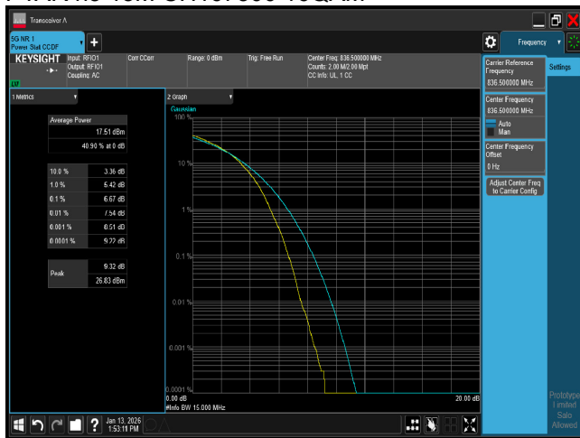
PTAR n5 15M CH167300 256QAM
