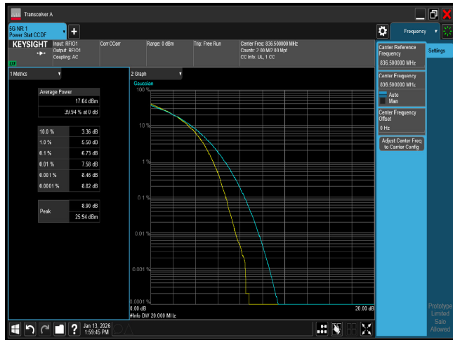
PTAR n5 20M CH167300 256QAM
