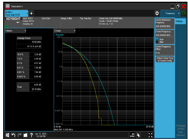
PTAR n5 15M CH167300 64QAM
