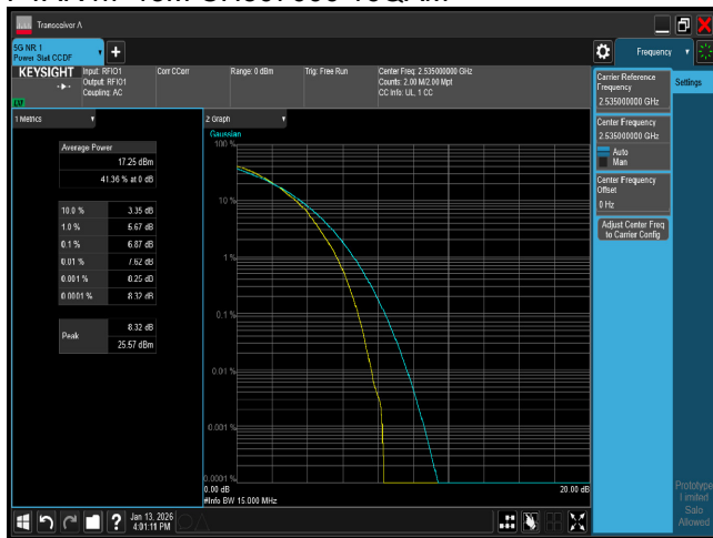
PTAR n7 15M CH507000 256QAM
