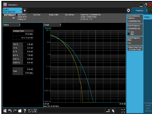
PTAR n7 20M CH507000 64QAM
