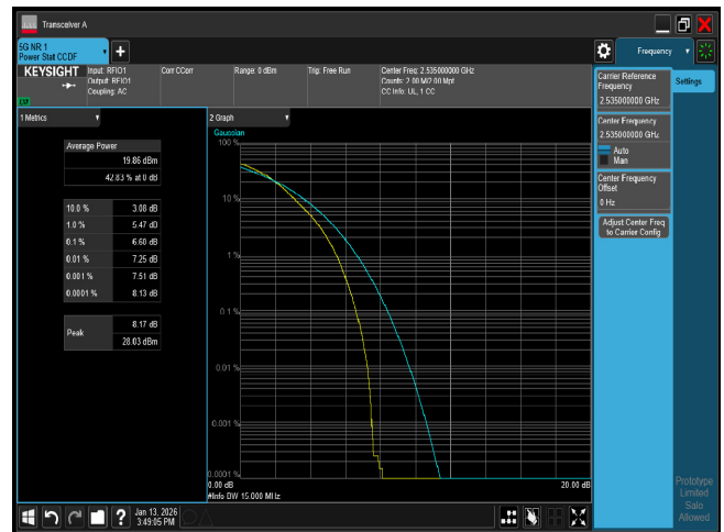
PTAR n7 15M CH507000 64QAM
