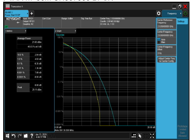
PTAR n7 30M CH507000 16QAM
