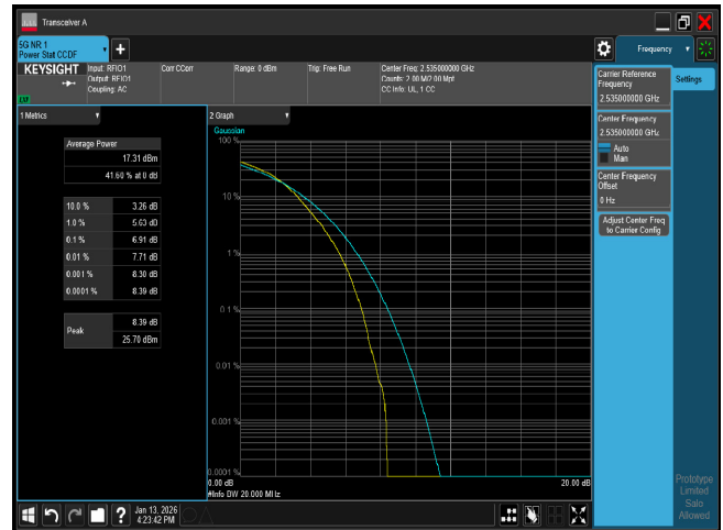
PTAR n7 20M CH507000 256QAM
