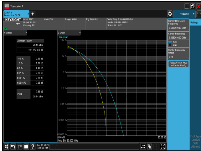
PTAR n7 30M CH507000 64QAM
