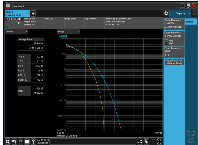
PTAR n7 25M CH507000 64QAM
