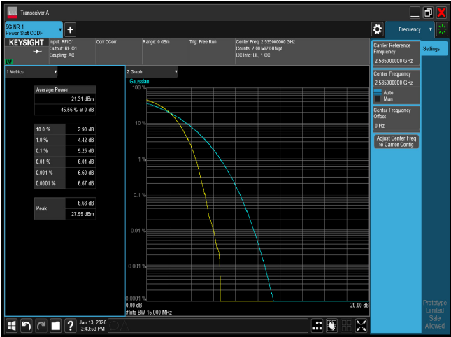
PTAR n7 15M CH507000 QPSK
