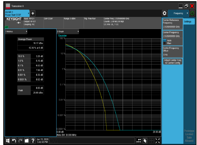
PTAR n7 30M CH507000 256QAM
