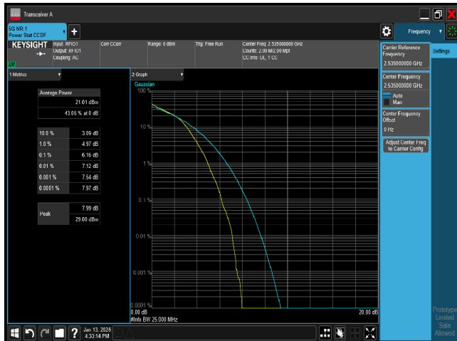
PTAR n7 25M CH507000 16QAM
