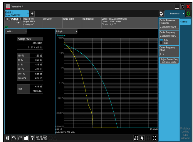
PTAR n7 30M CH507000 BPSK
