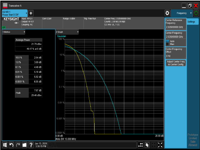
PTAR n7 15M CH507000 BPSK
