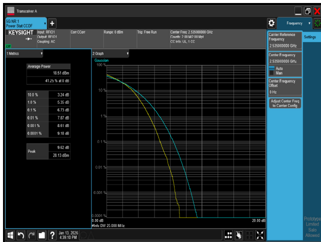
PTAR n7 25M CH507000 256QAM
