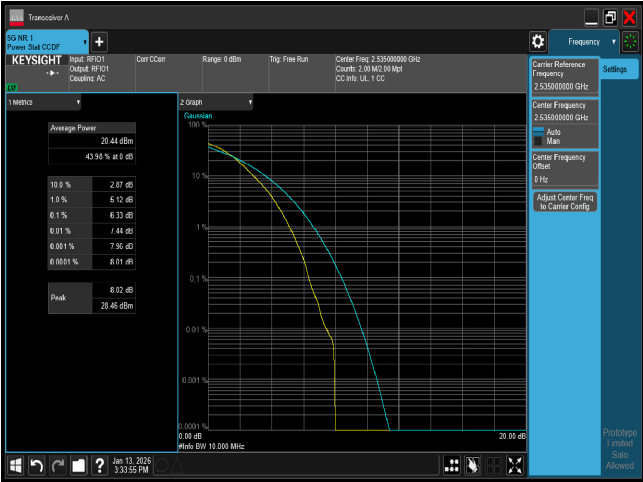
PTAR n7 10M CH507000 64QAM
