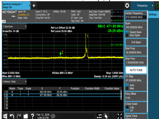
CSE B71 15M CH133397 QPSK(1,0)
