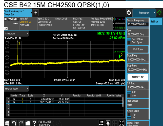
CSE B42 15M CH42590 QPSK(1,0)
