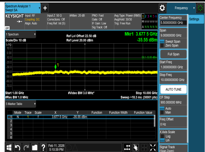
CSE B71 10M CH133172 QPSK(1,0)
