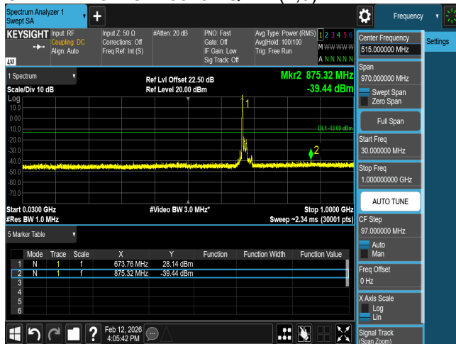
CSE B71 15M CH133297 QPSK(1,0)
