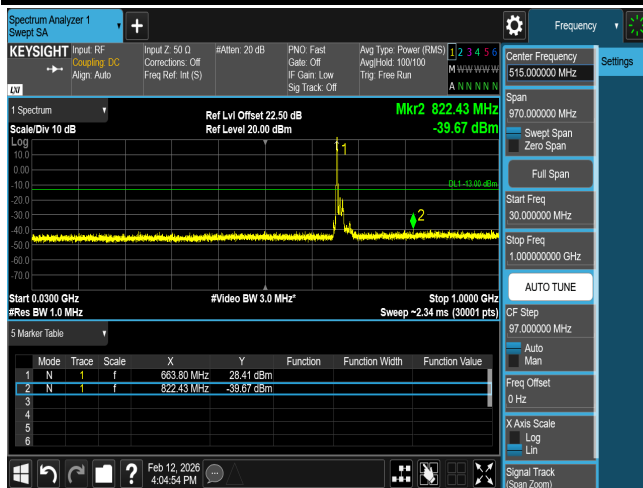
CSE B71 15M CH133197 QPSK(1,0)
