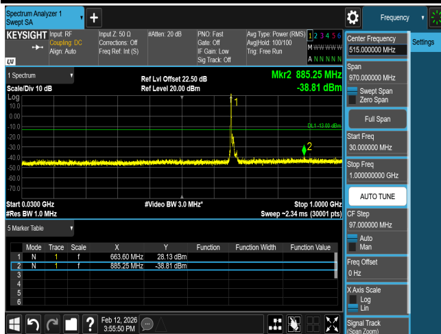
CSE B71 10M CH133172 QPSK(1,0)
