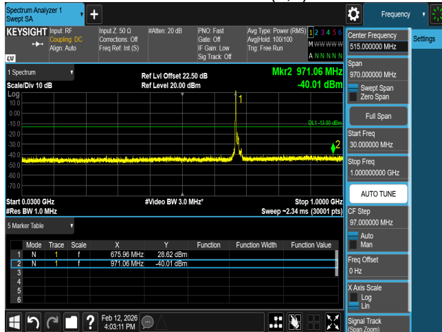
CSE B71 10M CH133297 QPSK(1,0)
