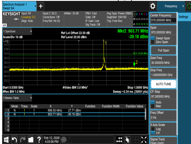
CSE B71 10M CH133422 QPSK(1,0)
