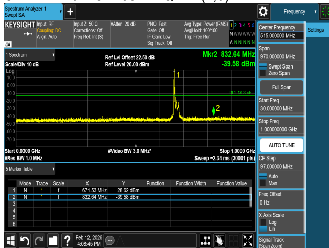
CSE B71 20M CH133297 QPSK(1,0)
