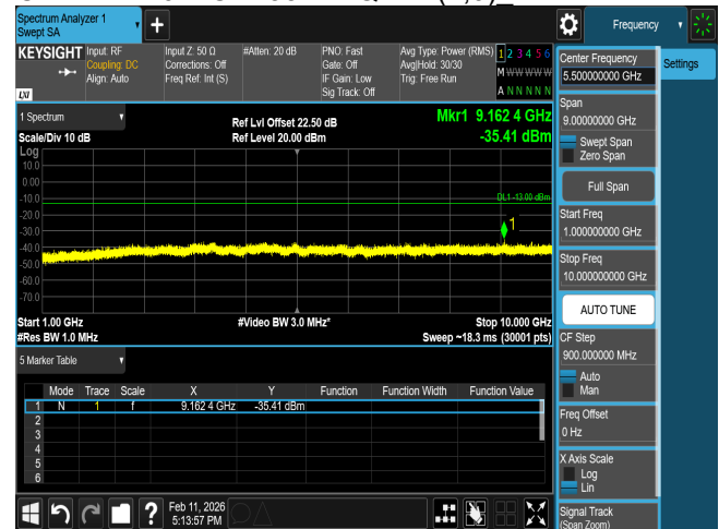
CSE B71 20M CH133297 QPSK(1,0)
