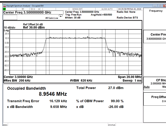
OCC B42 10M CH42590 256QAM
