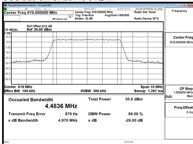
OCC B26 5M CH26740 64QAM
