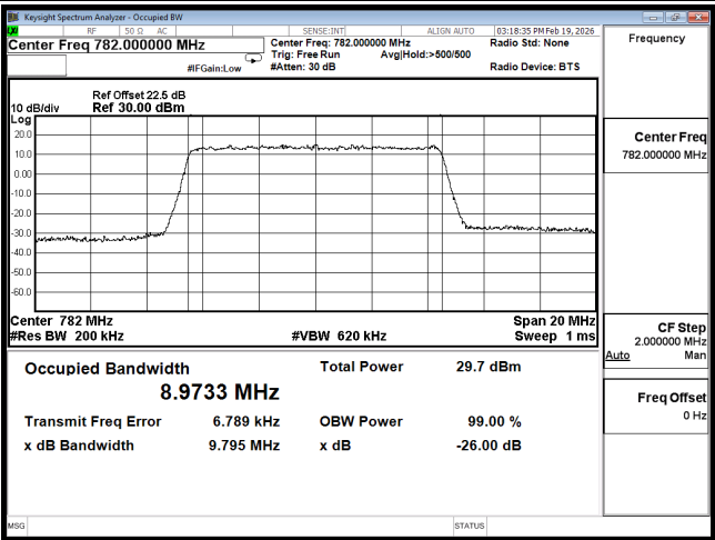
OCC B13 10M CH23230 64QAM
