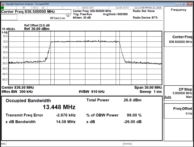
OCC B26 15M CH26915 256QAM
