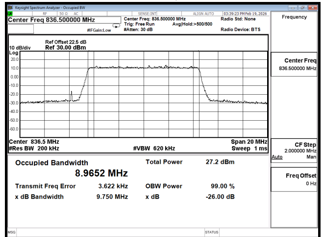
OCC B26 10M CH26915 256QAM
