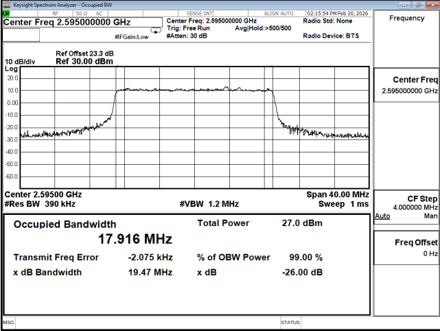
OCC B38 20M CH38000 256QAM
