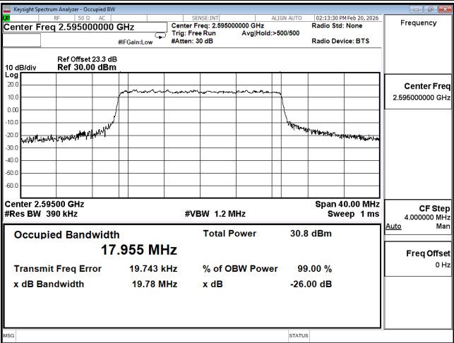
OCC B38 20M CH38000 QPSK
