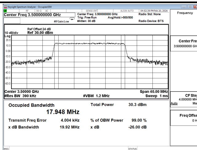
OCC B42 20M CH42590 16QAM
