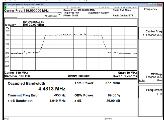
OCC B26 5M CH26740 256QAM
