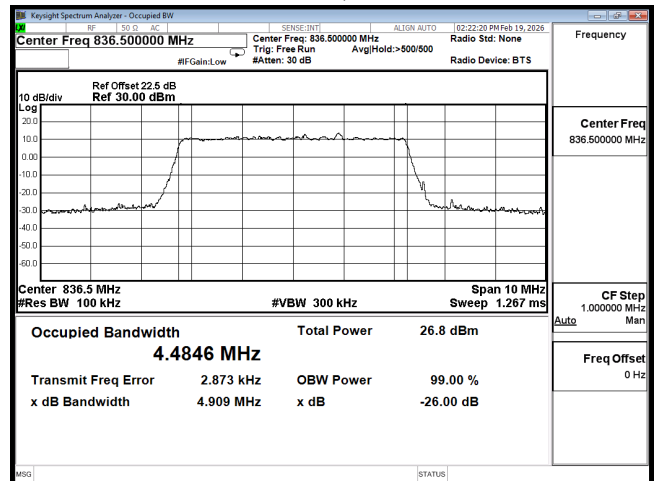
OCC B26 5M CH26915 256QAM
