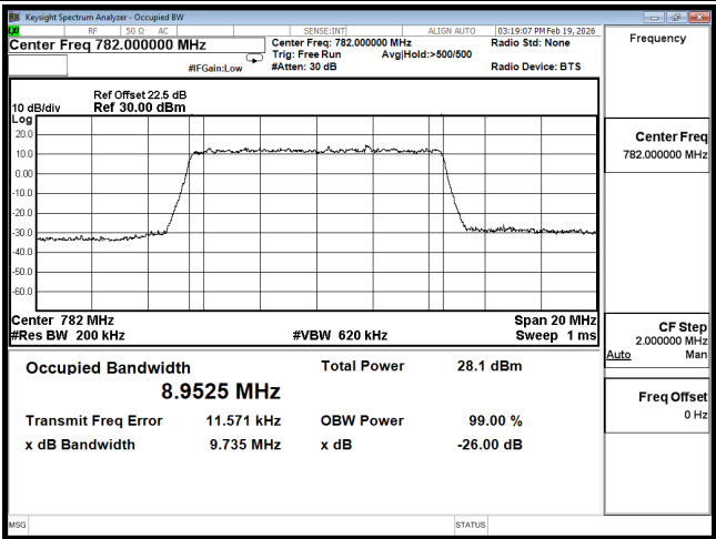
OCC B13 10M CH23230 256QAM
