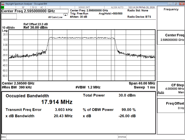
OCC B38 20M CH38000 16QAM
