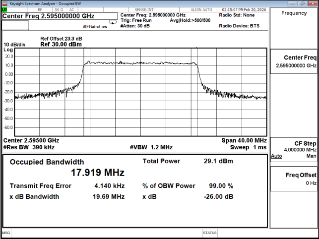
OCC B38 20M CH38000 64QAM
