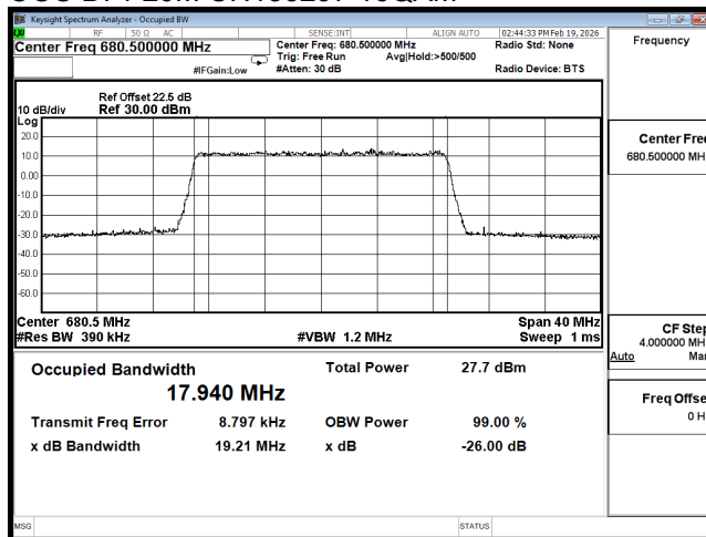
OCC B71 20M CH133297 256QAM
