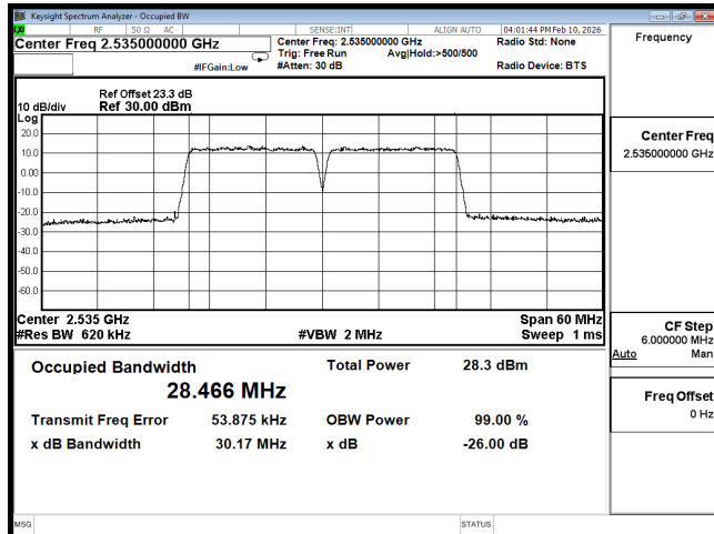
OOC B7 15M CH21025(75,0),15M CH21175(75,0) 64QAM
