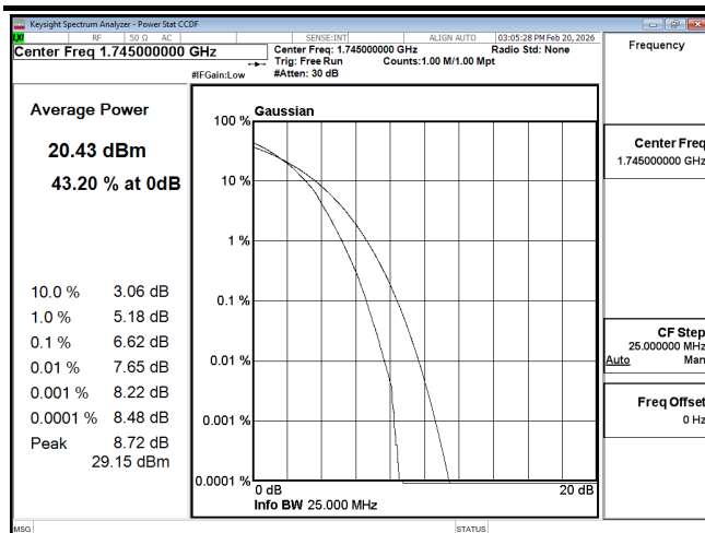
PTAR B66 15M CH132322 64QAM
