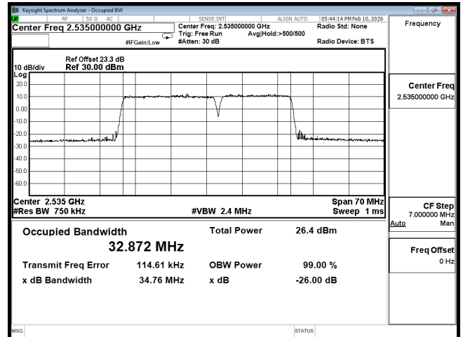
OOC B7 20M CH21026(100,0),15M CH21197(75,0) 256QAM
