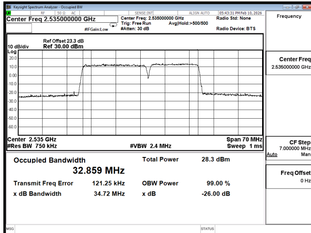
OOC B7 20M CH21026(100,0),15M CH21197(75,0) 64QAM
