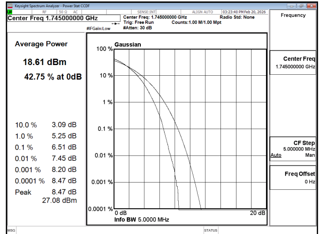
PTAR B66 5M CH132322 256QAM
