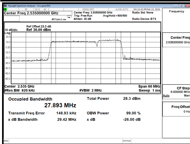
OOC B7 20M CH21051(100,0),10M CH21195(50,0) 64QAM
