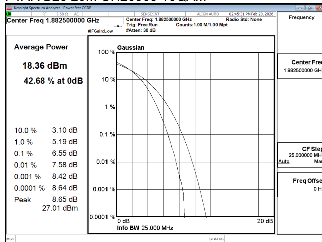
PTAR B25 20M CH26365 256QAM
