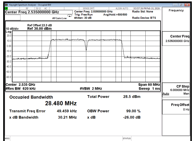
OOC B7 15M CH21025(75,0),15M CH21175(75,0) 16QAM
