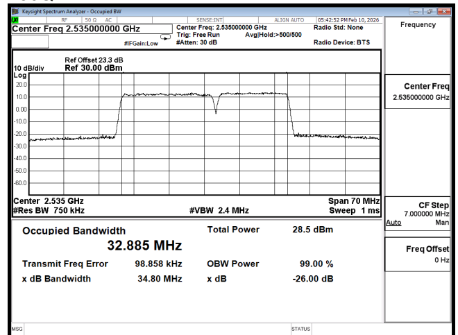
OOC B7 20M CH21026(100,0),15M CH21197(75,0) 16QAM
