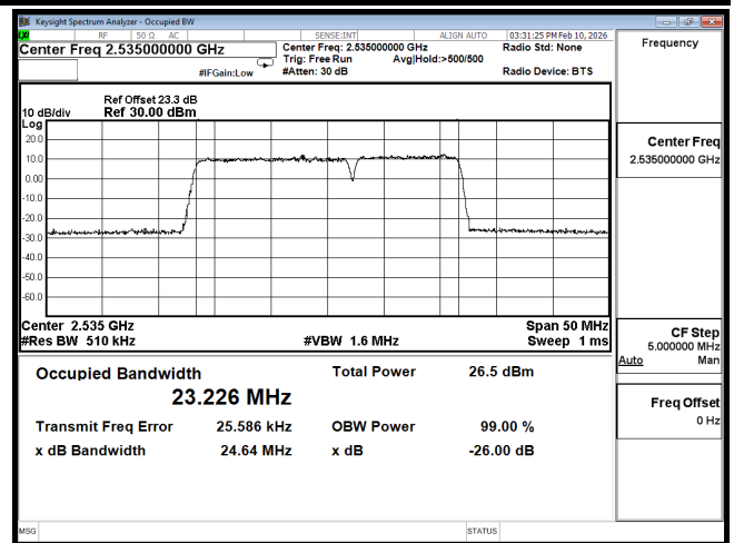
OOC B7 15M CH21051(75,0),10M CH21171(50,0) 256QAM
