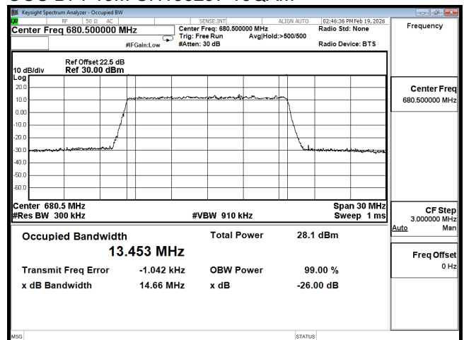
OCC B71 15M CH133297 256QAM
