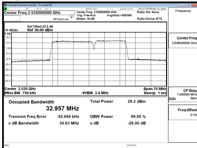
OOC B7 20M CH21026(100,0),15M CH21197(75,0) QPSK
