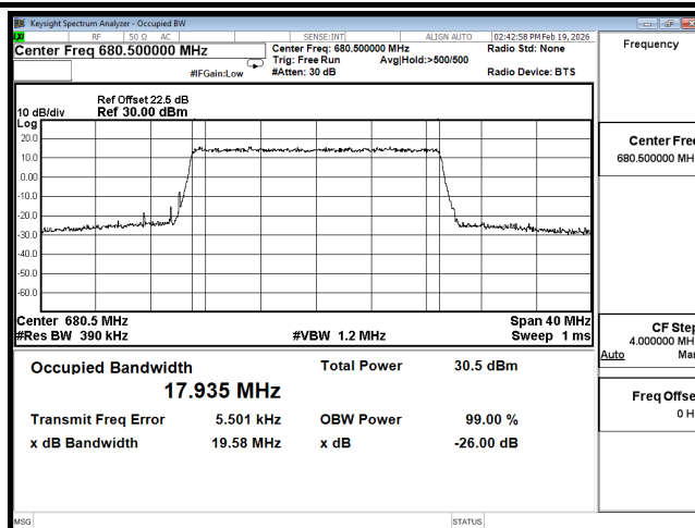
OCC B71 20M CH133297 16QAM
