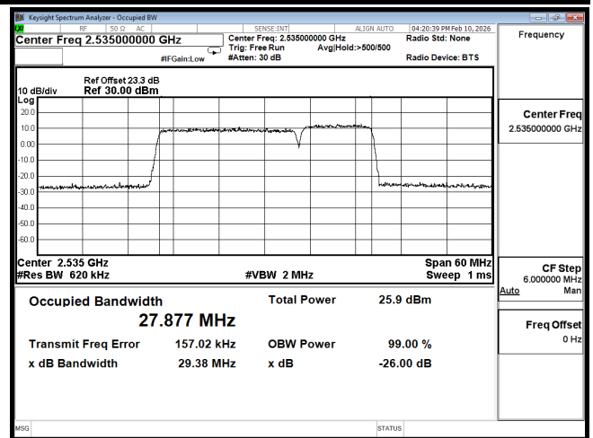
OOC B7 20M CH21051(100,0),10M CH21195(50,0) 256QAM
