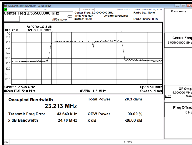
OOC B7 15M CH21051(75,0),10M CH21171(50,0) 64QAM
