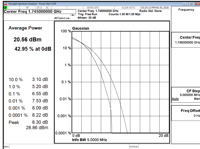
PTAR B66 5M CH132322 64QAM
