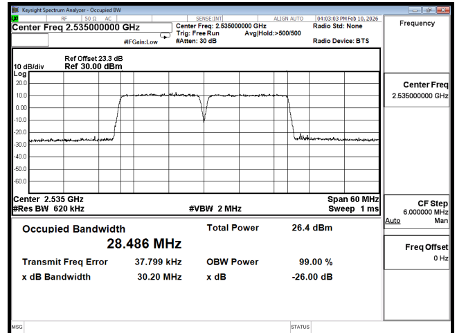
OOC B7 15M CH21025(75,0),15M CH21175(75,0) 256QAM
