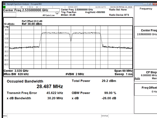
OOC B7 15M CH21025(75,0),15M CH21175(75,0) QPSK
