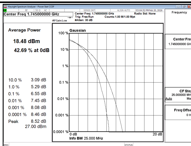
PTAR B66 15M CH132322 256QAM
