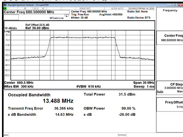
OCC B71 15M CH133297 QPSK
