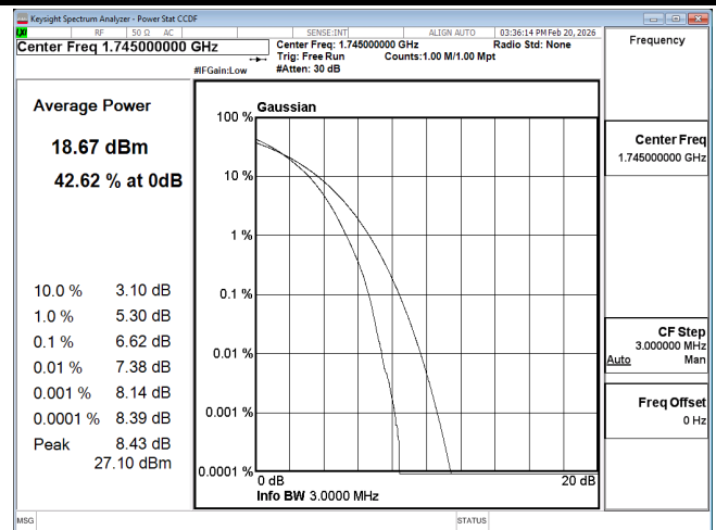
PTAR B66 3M CH132322 256QAM
