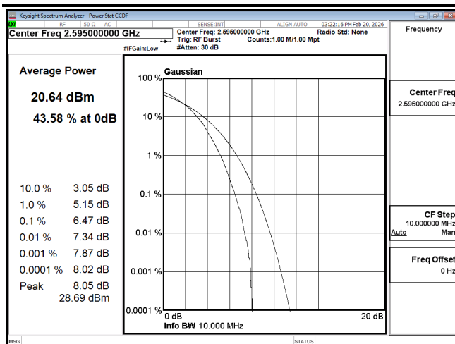
PTAR B38 10M CH38000 64QAM
