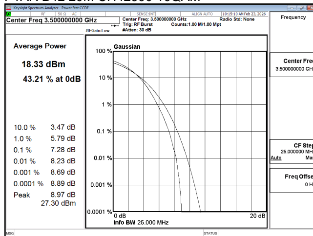
PTAR B42 20M CH42590 256QAM
