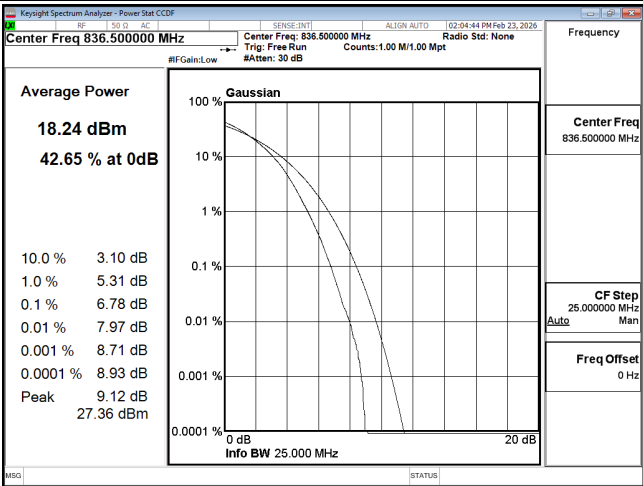
PTAR B26 15M CH26915 256QAM
