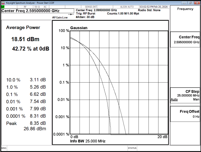
PTAR B38 20M CH38000 256QAM
