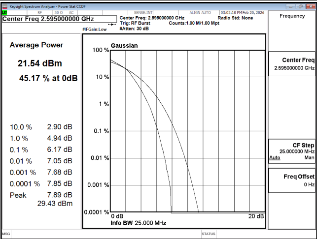
PTAR B38 20M CH38000 16QAM
