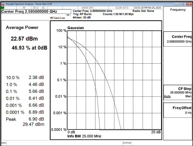
PTAR B38 20M CH38000 QPSK
