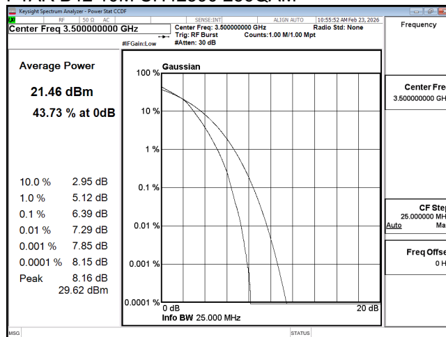
PTAR B42 15M CH42590 16QAM
