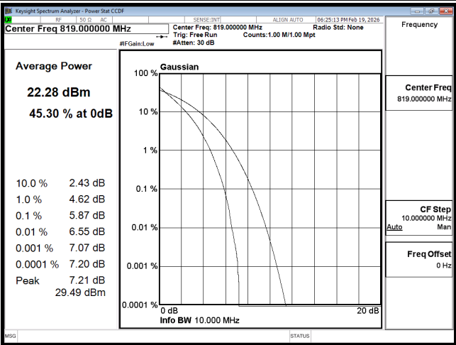
PTAR B26 10M CH26740 QPSK
