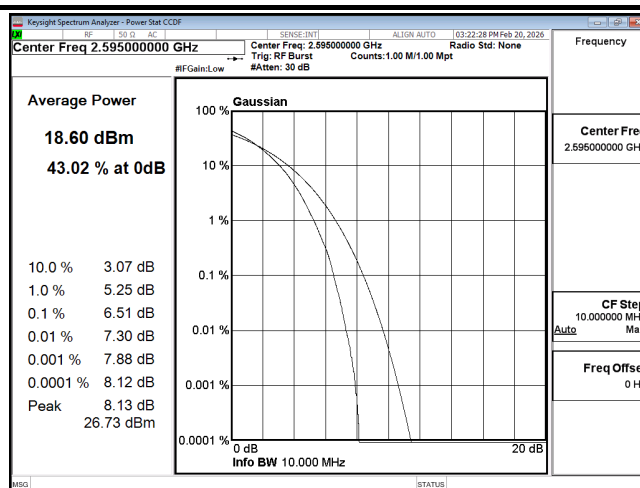
PTAR B38 10M CH38000 256QAM
