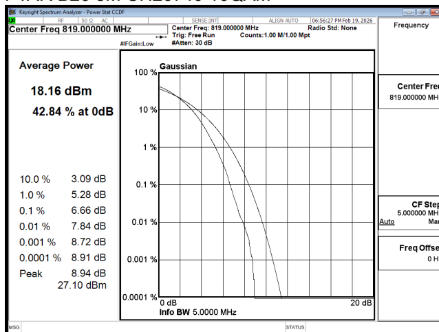
PTAR B26 5M CH26740 256QAM
