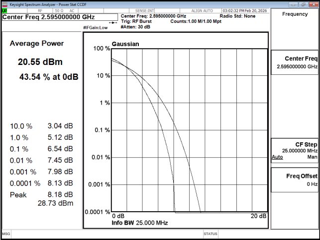
PTAR B38 20M CH38000 64QAM
