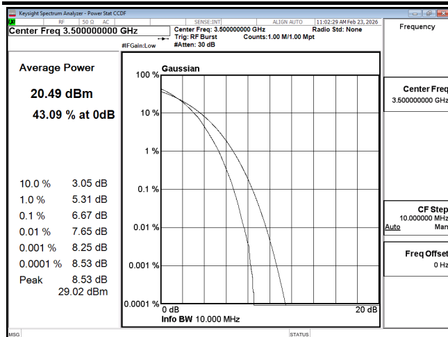
PTAR B42 10M CH42590 64QAM
