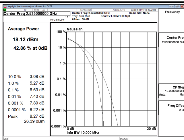
PTAR B7 10M CH21100 256QAM
