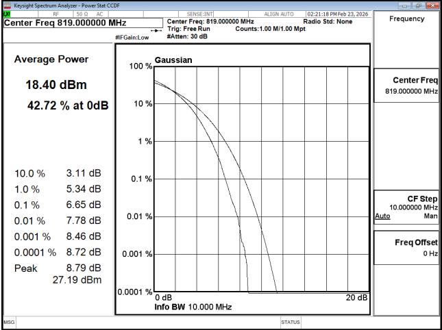
PTAR B26 10M CH26740 256QAM
