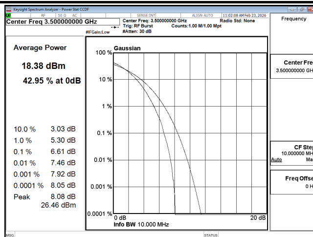
PTAR B42 10M CH42590 256QAM
