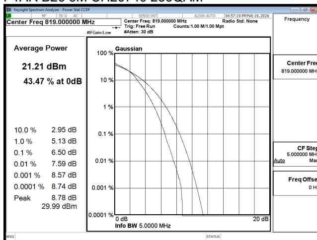
PTAR B26 5M CH26740 16QAM
