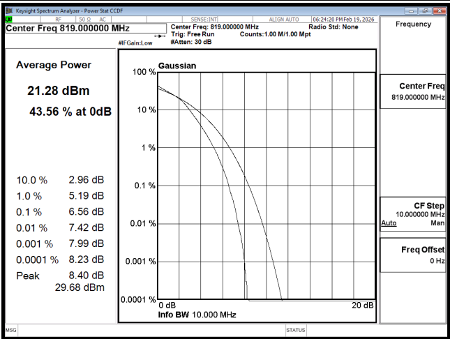
PTAR B26 10M CH26740 16QAM
