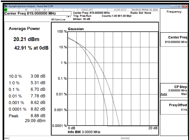
PTAR B26 3M CH26740 64QAM
