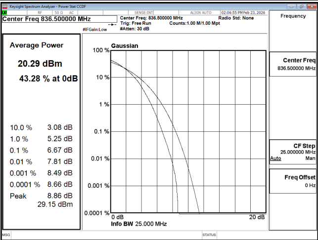
PTAR B26 15M CH26915 64QAM
