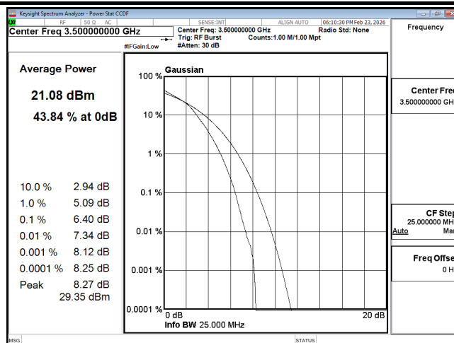
PTAR B42 20M CH42590 16QAM
