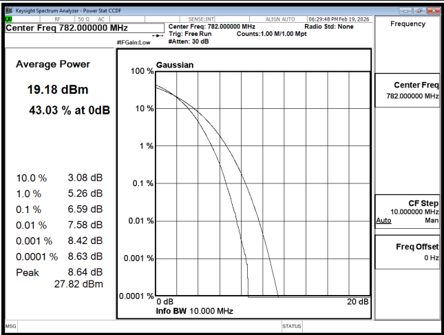
PTAR B13 10M CH23230 256QAM
