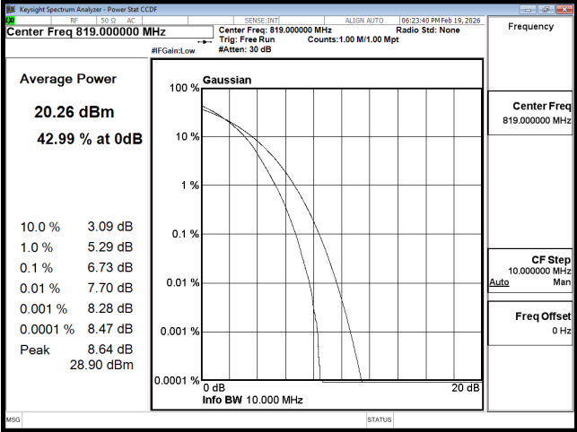
PTAR B26 10M CH26740 64QAM
