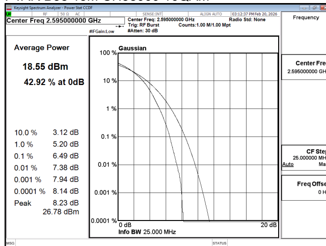
PTAR B38 15M CH38000 256QAM
