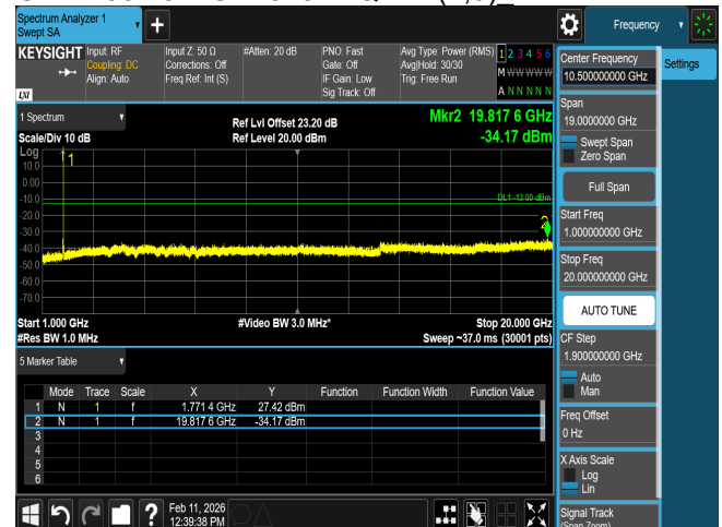
CSE B66 10M CH132622 QPSK(1,0)_
