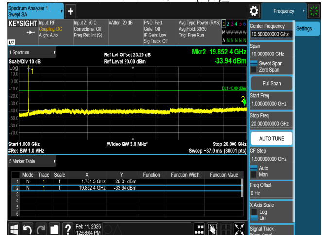
CSE B66 20M CH132572 QPSK(1,0)_
