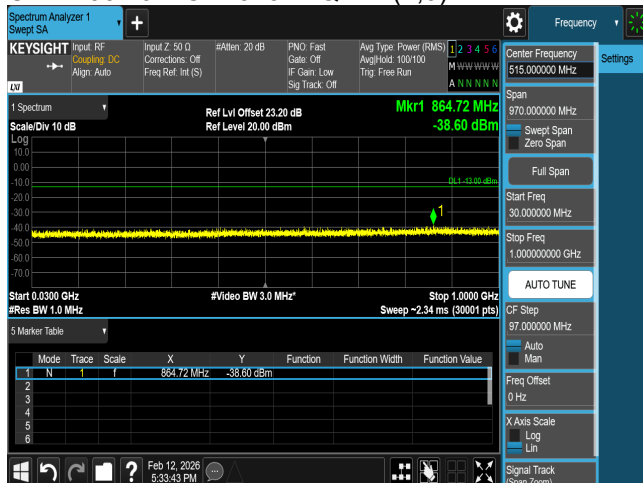
CSE B66 10M CH132622 QPSK(1,0)
