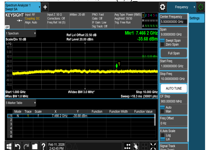
CSE B26 5M CH27015 QPSK(1,0)_
