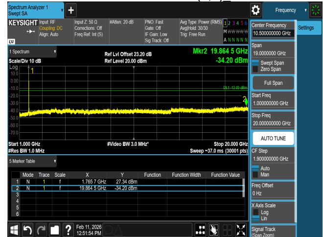
CSE B66 15M CH132597 QPSK(1,0)_
