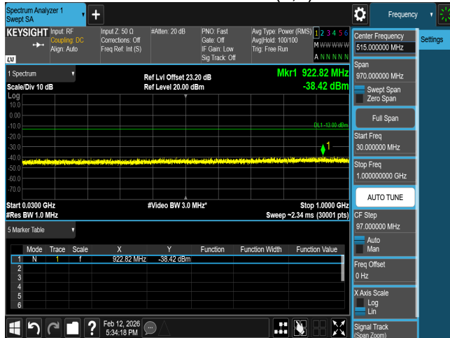
CSE B66 15M CH132322 QPSK(1,0)
