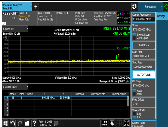
CSE B66 15M CH132047 QPSK(1,0)
