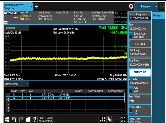
CSE B66 10M CH132022 QPSK(1,0)
