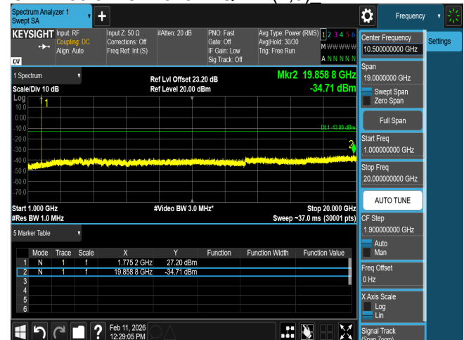
CSE B66 5M CH132647 QPSK(1,0)_
