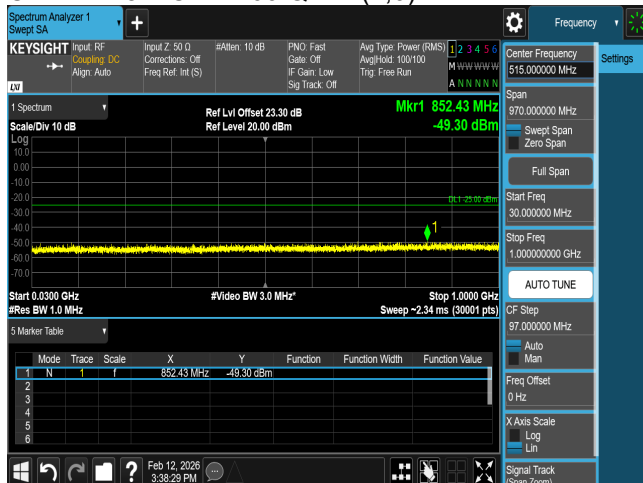
CSE B7 15M CH21375 QPSK(1,0)
