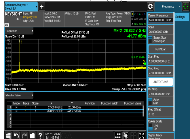
CSE B7 10M CH21400 QPSK(1,0)_
