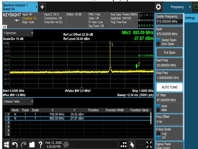
CSE B12 3M CH23095 QPSK(1,0)
