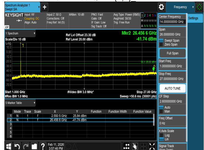
CSE B7 20M CH21350 QPSK(1,0)_
