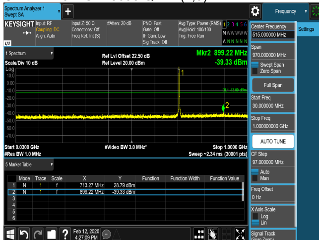
CSE B12 3M CH23165 QPSK(1,0)
