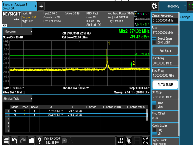
CSE B12 10M CH23060 QPSK(1,0)
