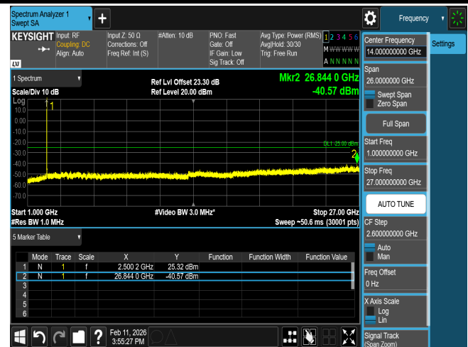
CSE B7 20M CH20850 QPSK(1,0)
