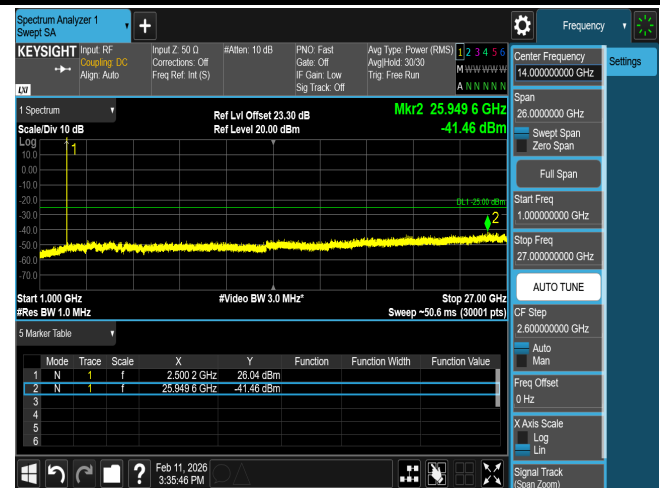
CSE B7 10M CH20800 QPSK(1,0)
