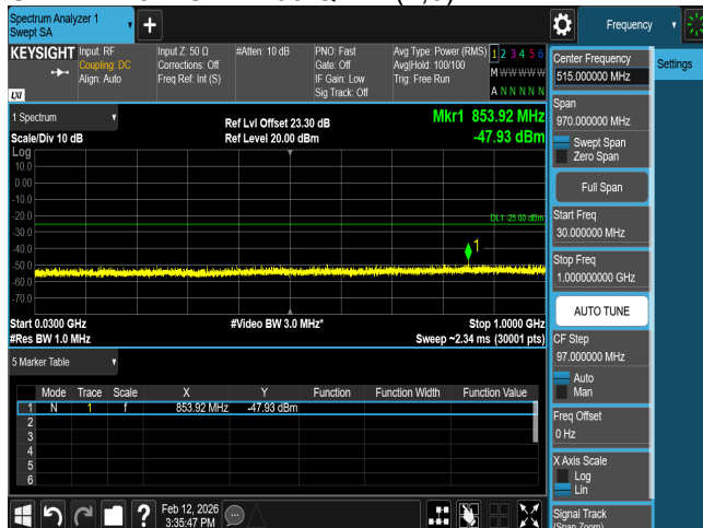
CSE B7 10M CH21400 QPSK(1,0)
