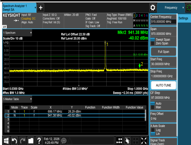
CSE B12 3M CH23025 QPSK(1,0)
