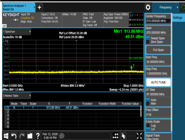
CSE B7 20M CH20850 QPSK(1,0)
