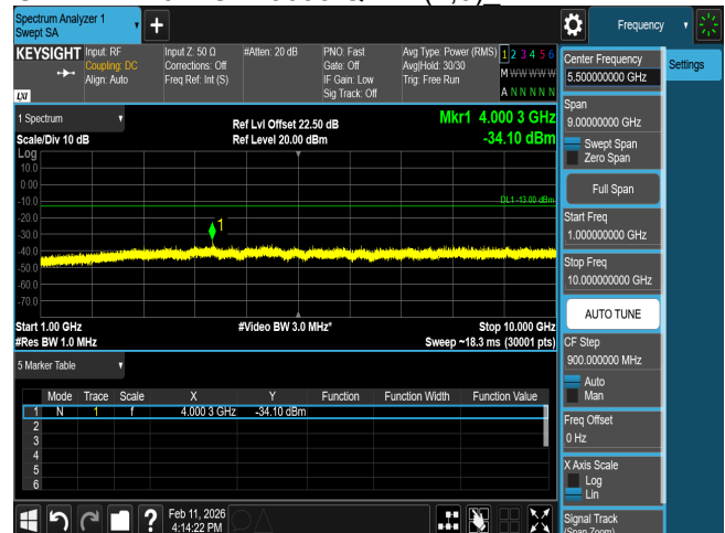
CSE B12 10M CH23095 QPSK(1,0)
