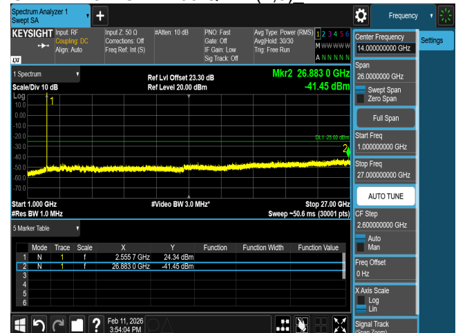
CSE B7 15M CH21375 QPSK(1,0)_
