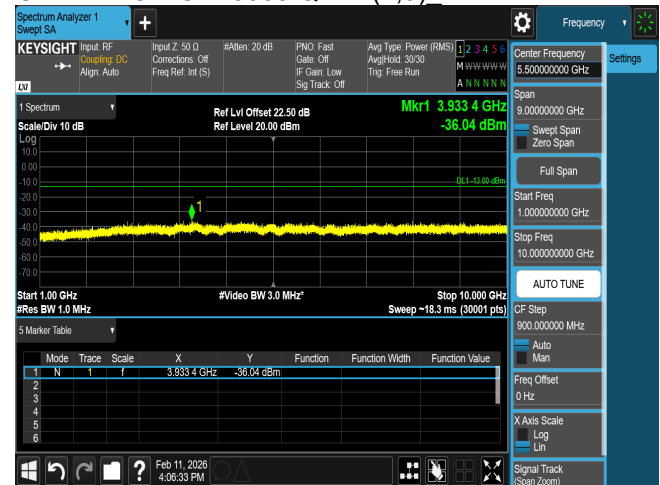
CSE B12 5M CH23035 QPSK(1,0)
