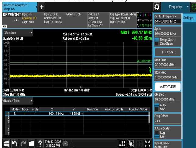
CSE B7 10M CH21100 QPSK(1,0)
