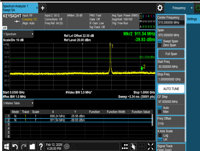
CSE B12 5M CH23035 QPSK(1,0)
