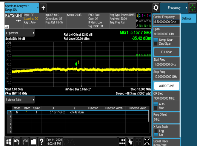
CSE B12 3M CH23025 QPSK(1,0)
