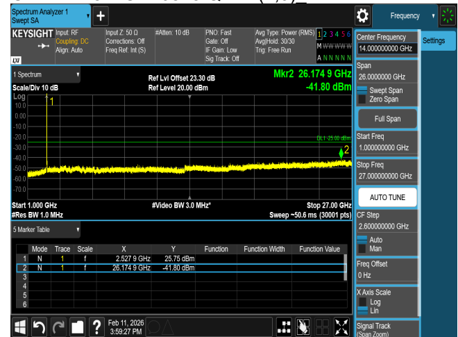
CSE B7 15M CH21100 QPSK(1,0)
