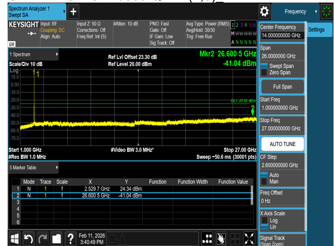
CSE B7 10M CH21100 QPSK(1,0)
