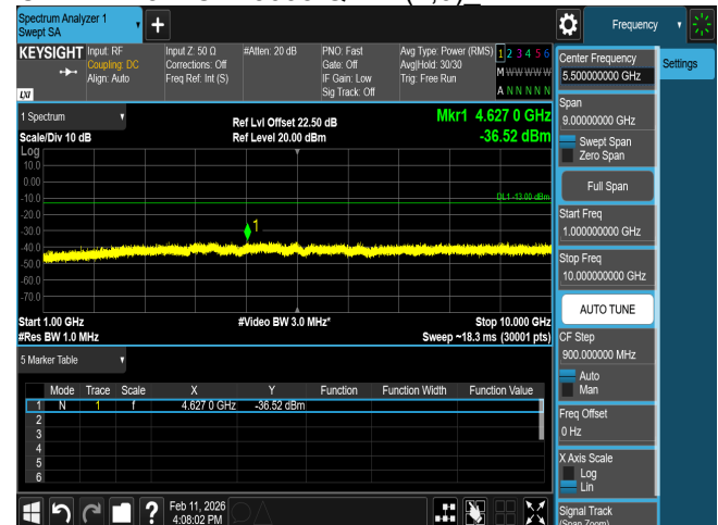
CSE B12 5M CH23155 QPSK(1,0)_
