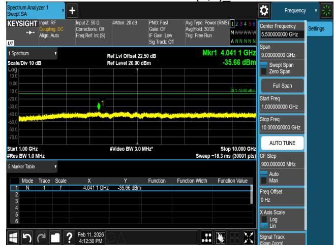
CSE B12 10M CH23060 QPSK(1,0)
