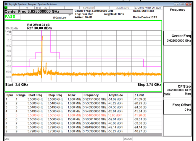
EDGE n48 15M CH637168 BPSK(1,0)
