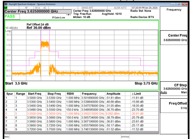
EDGE n48 15M CH637168 BPSK(36,0)
