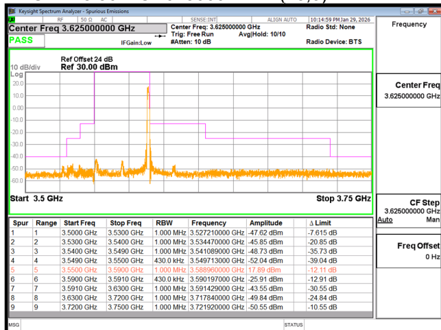
EDGE n48 40M CH638000 BPSK(1,105)
