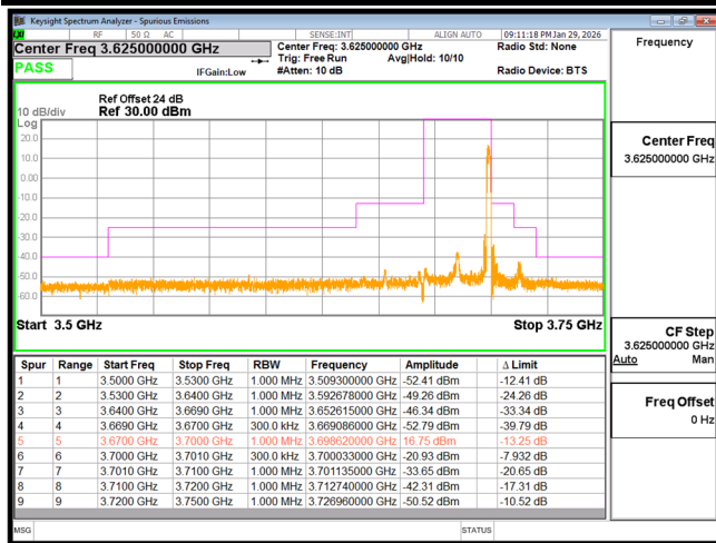
EDGE n48 30M CH645666 BPSK(1,77)
