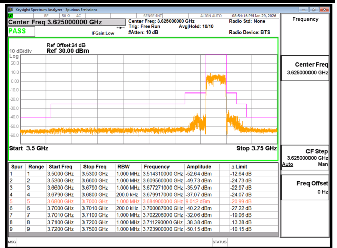
EDGE n48 20M CH646000 BPSK(50,0)
