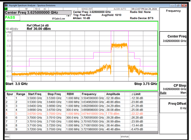
EDGE n48 30M CH645666 BPSK(75,0)
