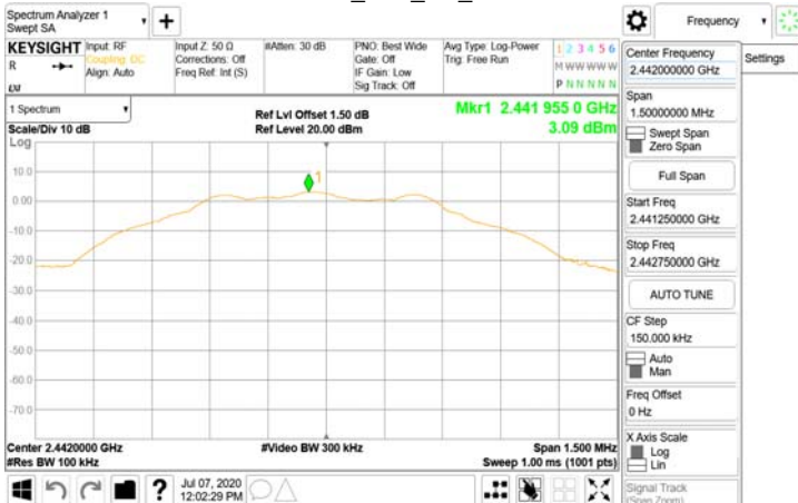
Reference Level_BLE_1M_MidCH20-2442
