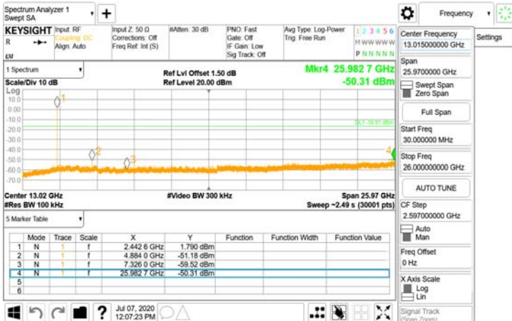
Spurious Emission_BLE_1M_MidCH20-2442
