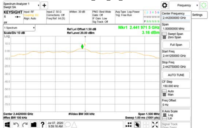
Reference Level_BLE_2M_MidCH20-2442
