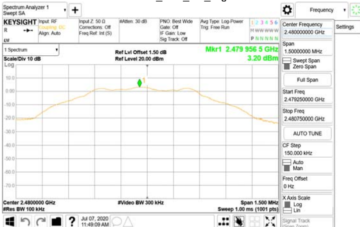
Reference Level_BLE_1M_HighCH39-2480
