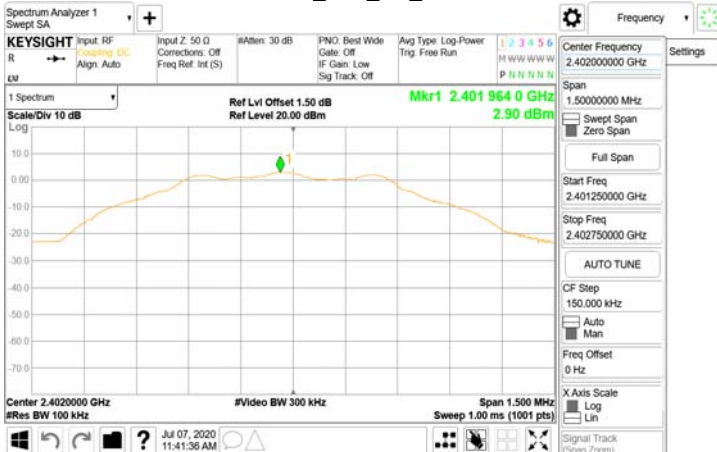
Reference Level_BLE_1M_LowCH00-2402
