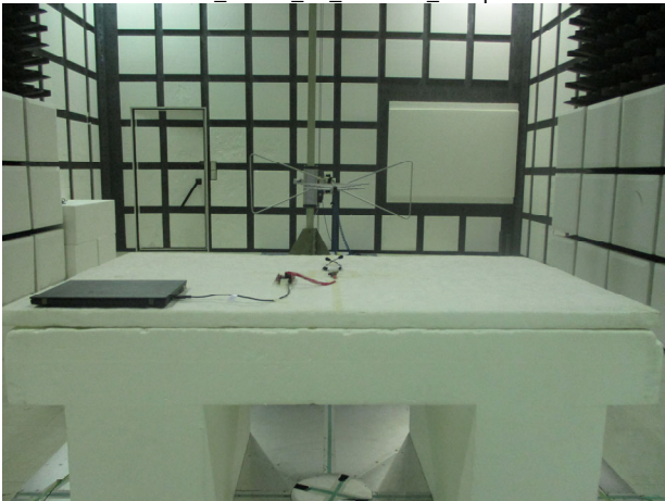
Part_15.247_LE_Radiated_Setup
