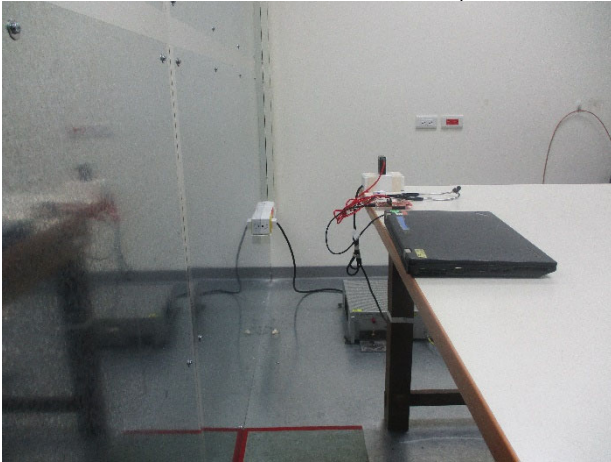
Part_15.247_LE_Conduction_Setup
