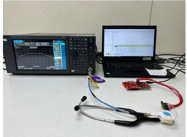
Part_15.247_LE_Conduction_Setup
