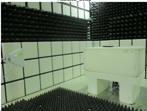
Radiated Setup
