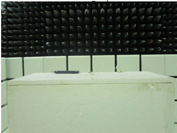
Radiated Setup
