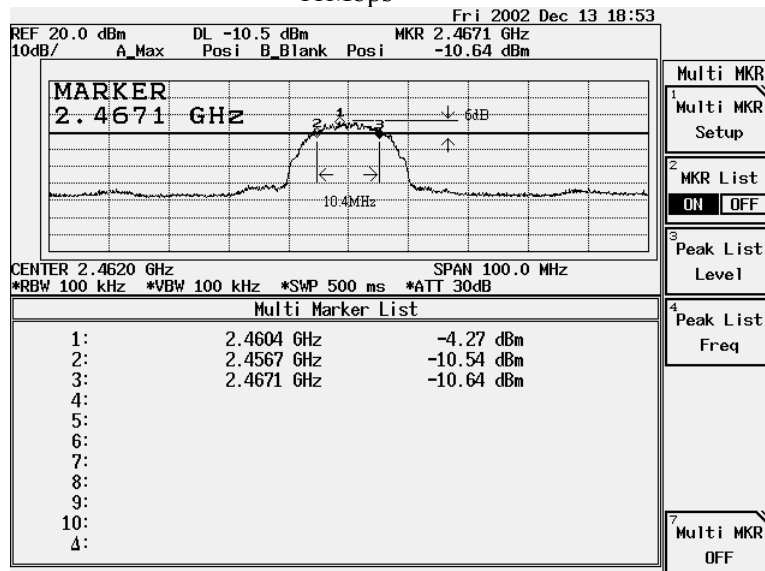
Figure Channel 11: 11Mbps
