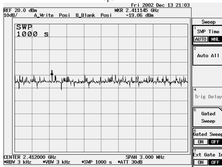
Figure Channel 1: 11Mbps
