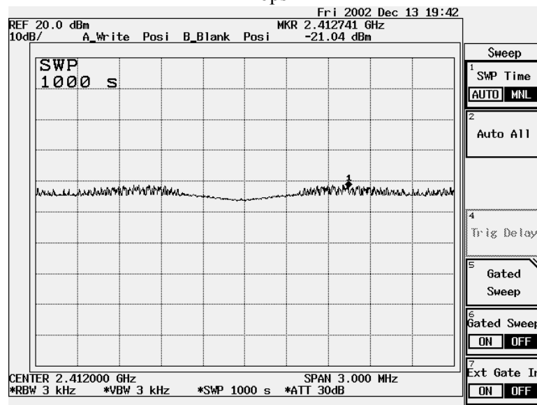
Figure Channel 1: 1Mbps
