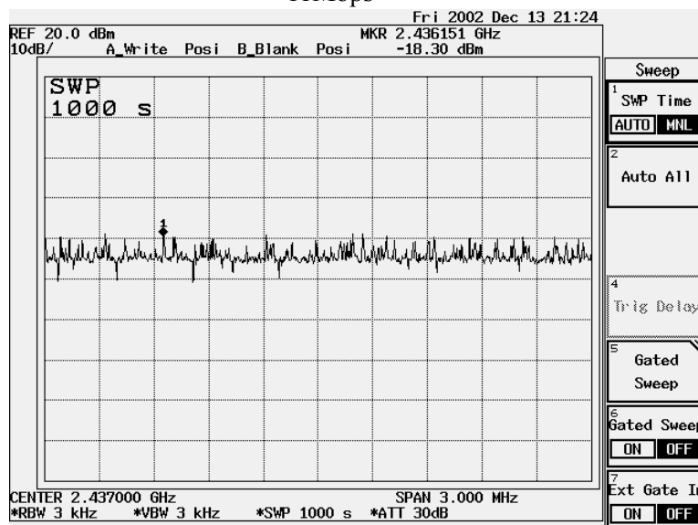
Figure Channel 6: 11Mbps
