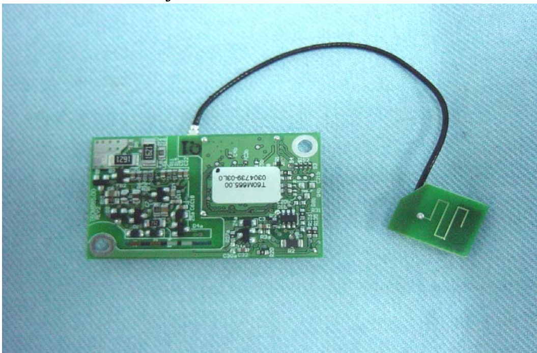
Back of Bluetooth Module with Antenna
