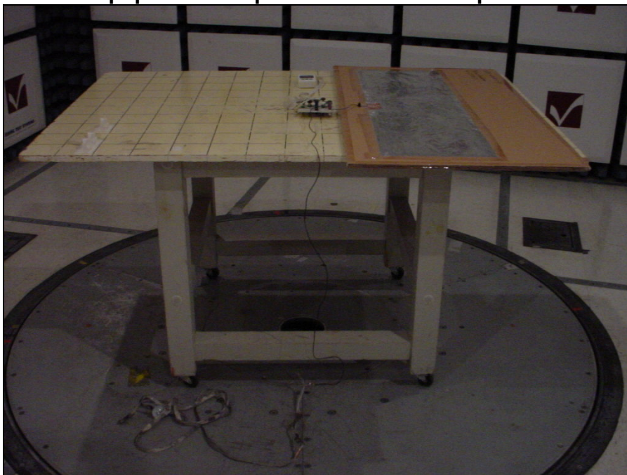
View of the equipment setup with the simulated patient connected.
