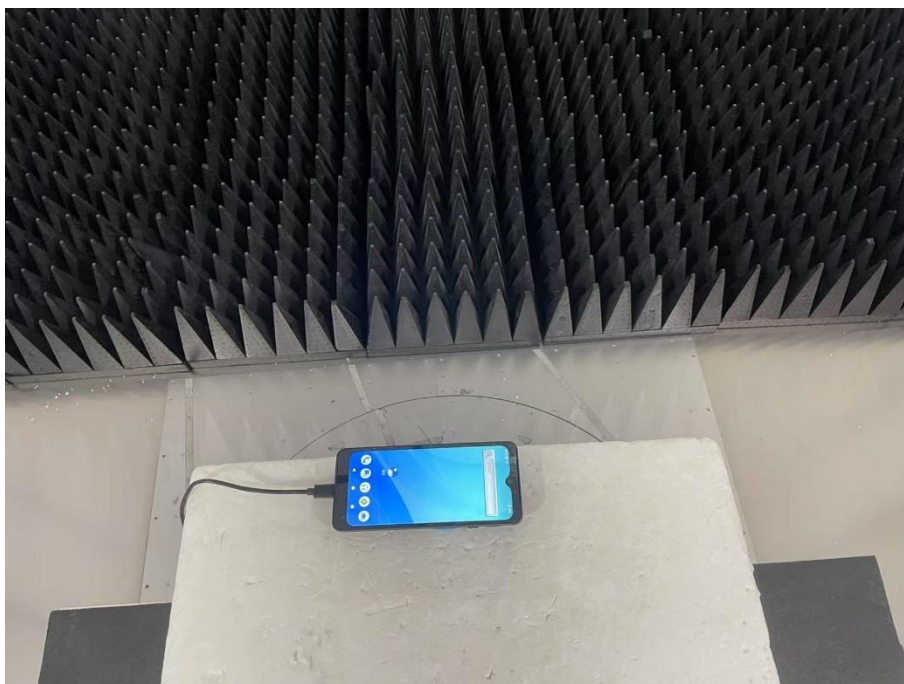
Close-up-UHF
