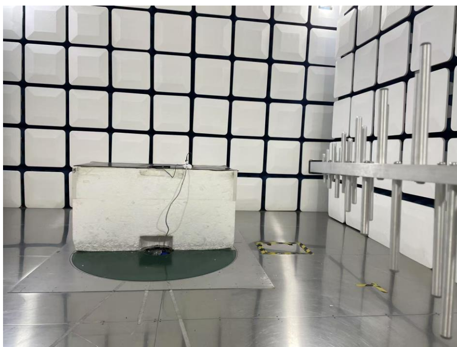
30MHz-1GHz-UHF
