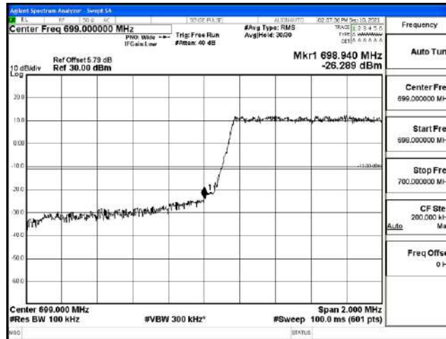
Band12-5MHz-QPSK-23155-25RB#0
