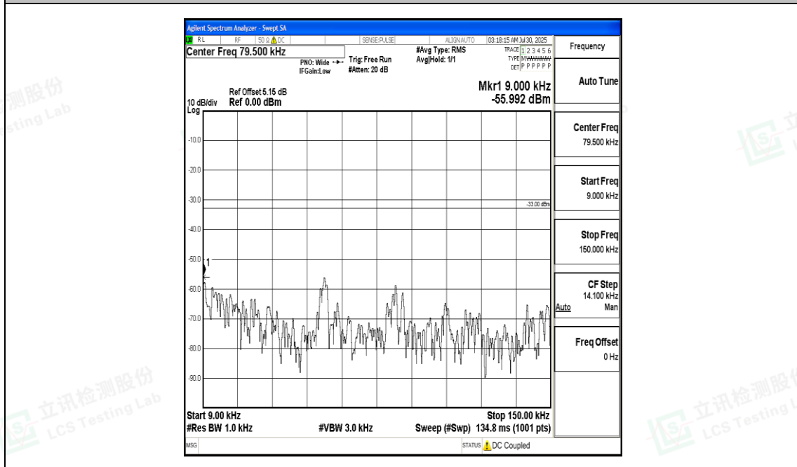
Band17_10MHz_16QAM_23790_1RB#0_0.009~0.15_0.009~0.15
