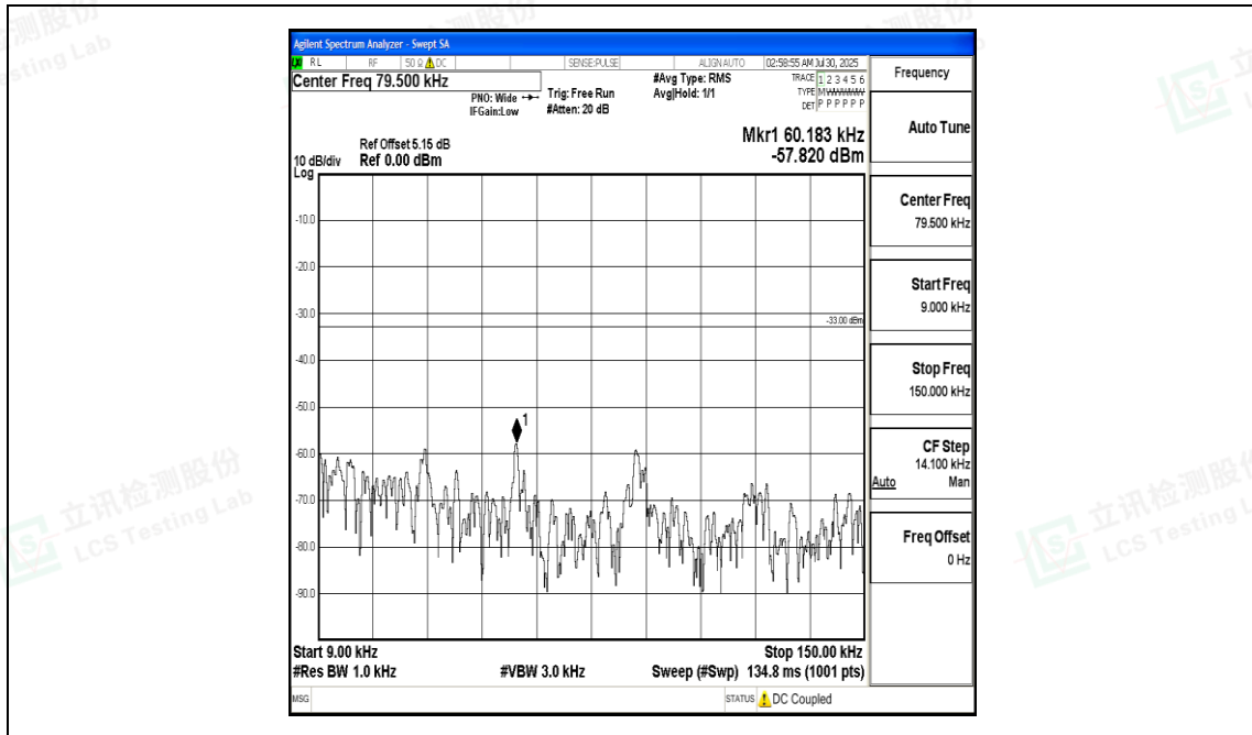
Band17_5MHz_QPSK_23790_1RB#0_0.009~0.15_0.009~0.15
