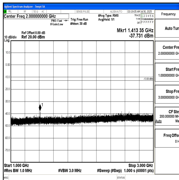
Band17_10MHz_QPSK_23800_1RB#0_1000~3000_1000~3000
