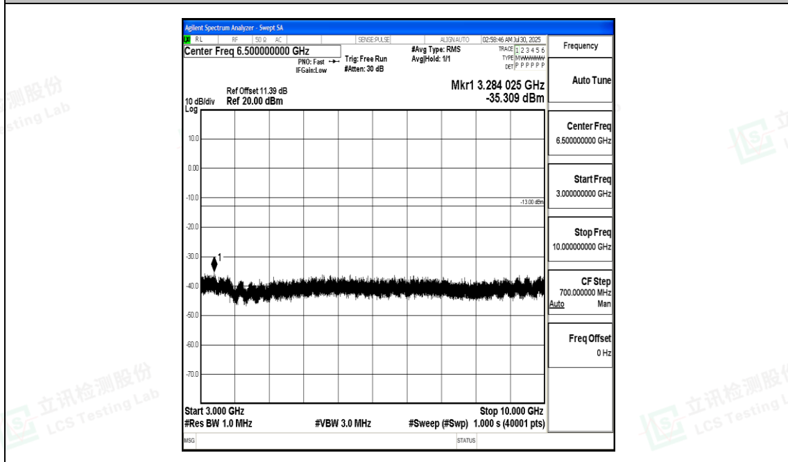
Band17_5MHz_16QAM_23755_1RB#0_3000~10000_3000~10000
