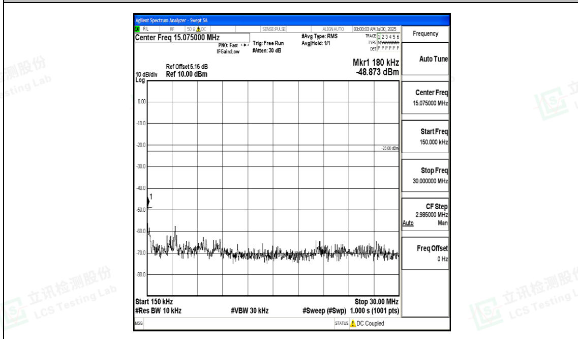
Band17_5MHz_QPSK_23825_1RB#0_0.15~30_0.15~30
