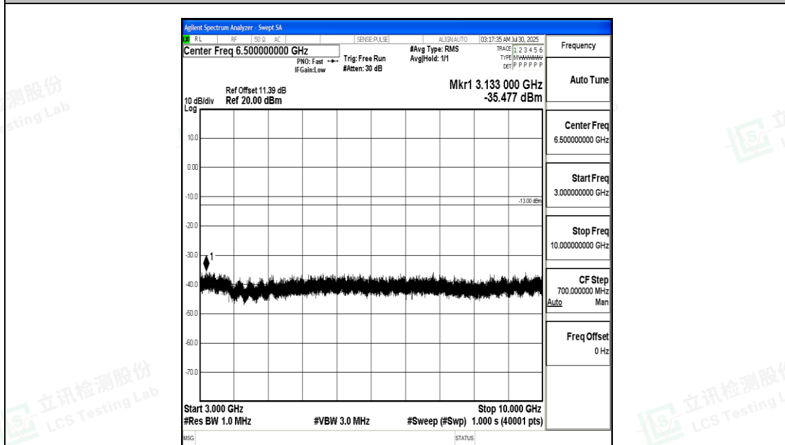
Band17_10MHz_16QAM_23780_1RB#0_3000~10000_3000~10000
