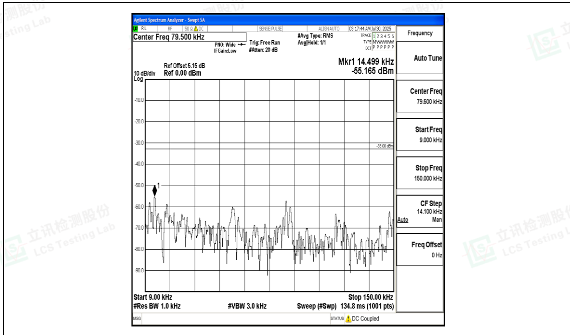
Band17_10MHz_QPSK_23790_1RB#0_0.009~0.15_0.009~0.15
