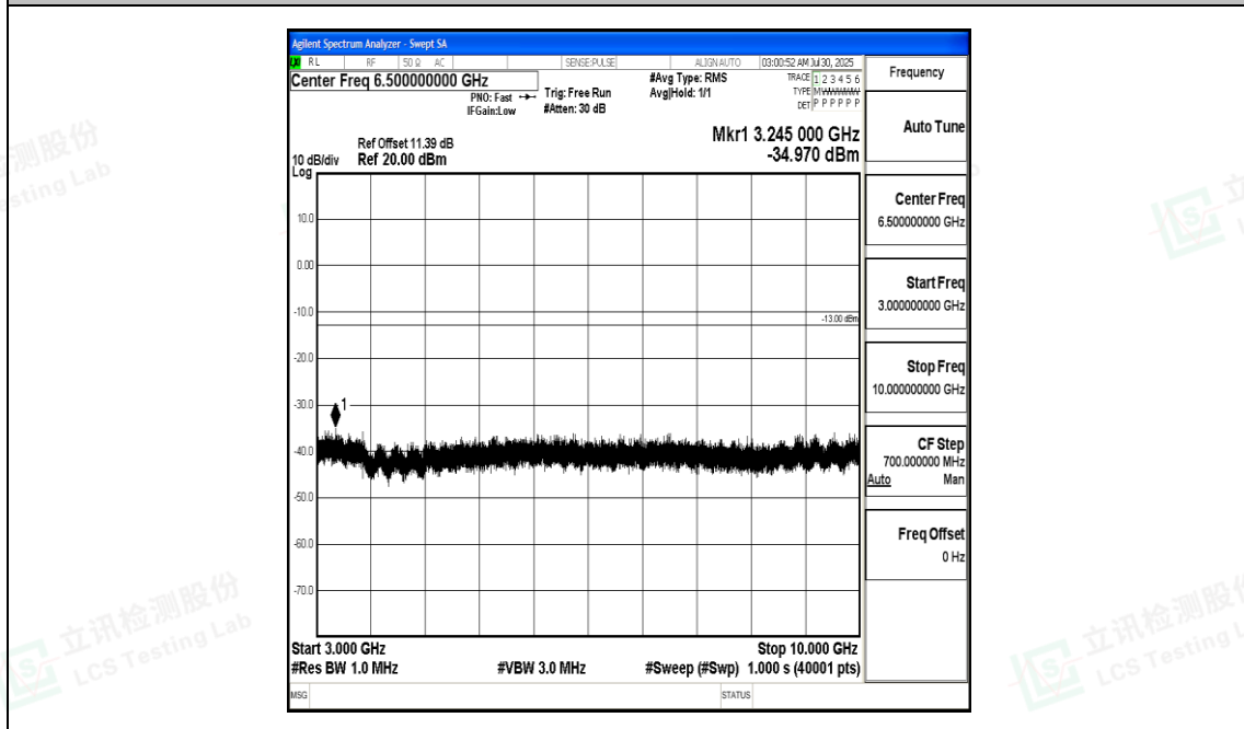
Band17_5MHz_16QAM_23825_1RB#0_3000~10000_3000~10000
