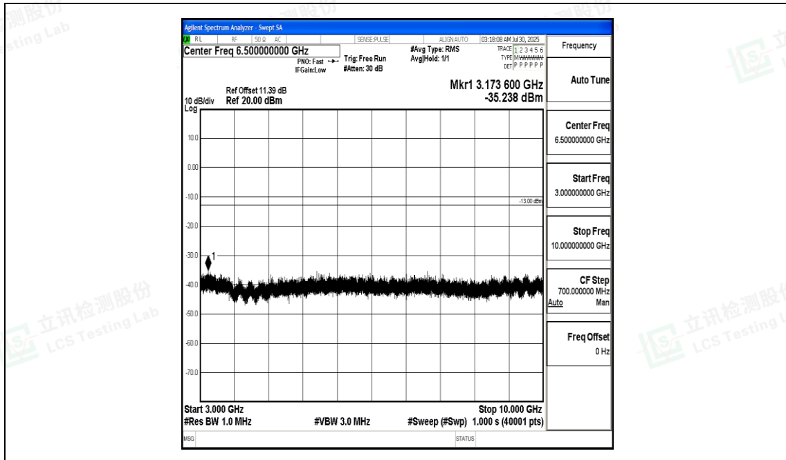
Band17_10MHz_QPSK_23790_1RB#0_3000~10000_3000~10000
