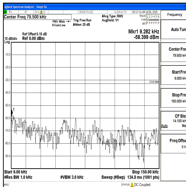
Band17_10MHz_16QAM_23780_1RB#0_0.009~0.15_0.009~0.15
