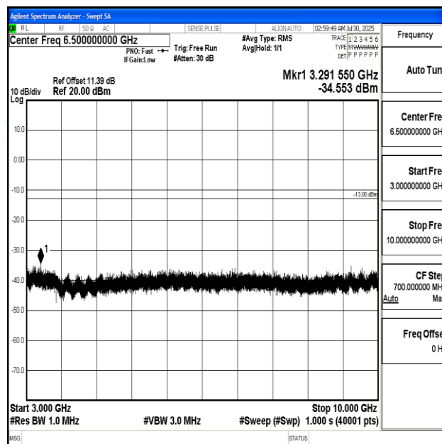
Band17_5MHz_16QAM_23790_1RB#0_3000~10000_3000~10000
