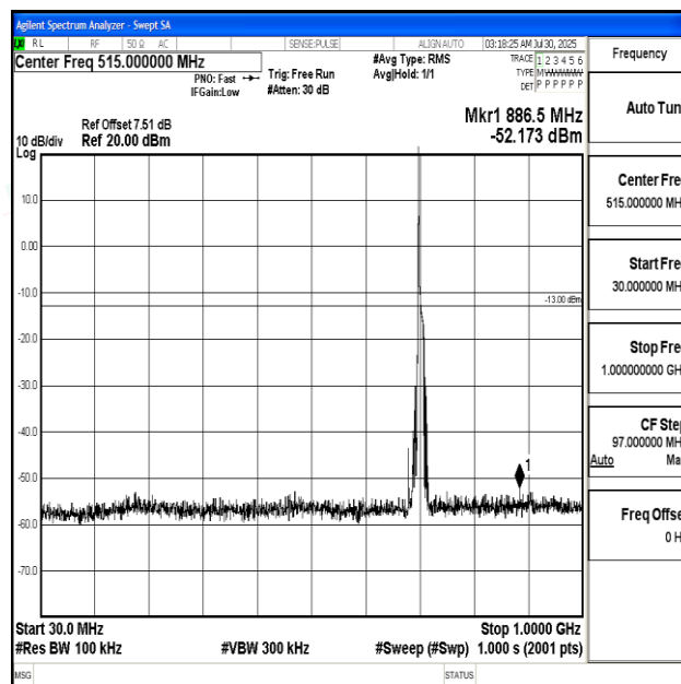
Band17_10MHz_16QAM_23790_1RB#0_30~1000_30~1000
