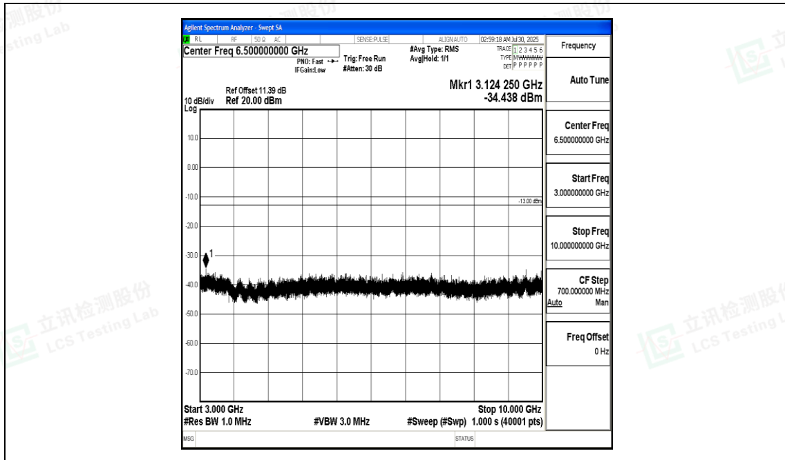
Band17_5MHz_QPSK_23790_1RB#0_3000~10000_3000~10000
