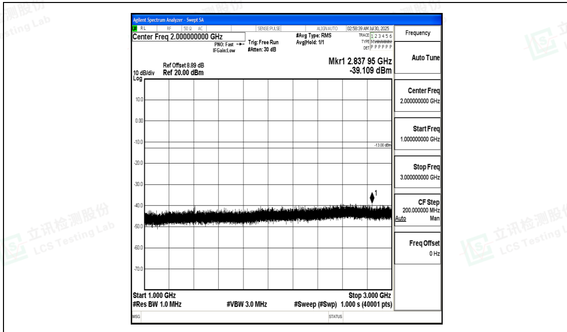
Band17_5MHz_16QAM_23755_1RB#0_1000~3000_1000~3000
