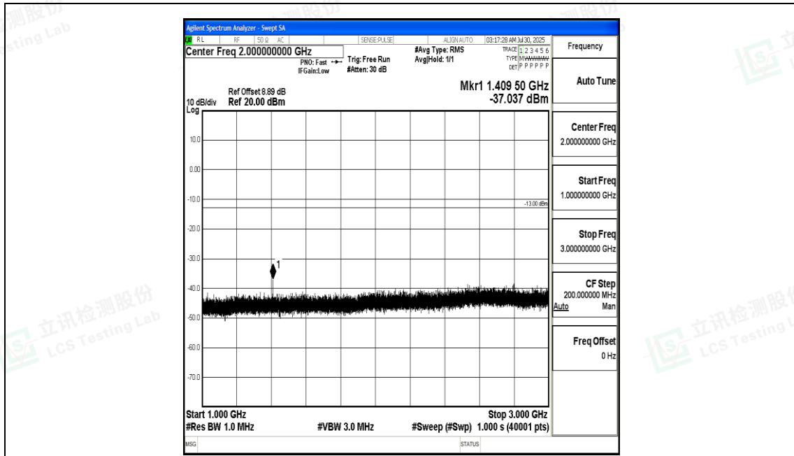
Band17_10MHz_16QAM_23780_1RB#0_1000~3000_1000~3000
