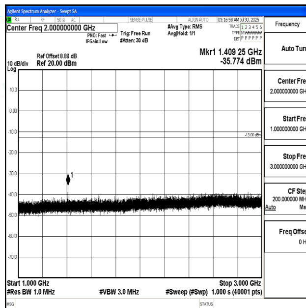
Band17_10MHz_QPSK_23780_1RB#0_1000~3000_1000~3000
