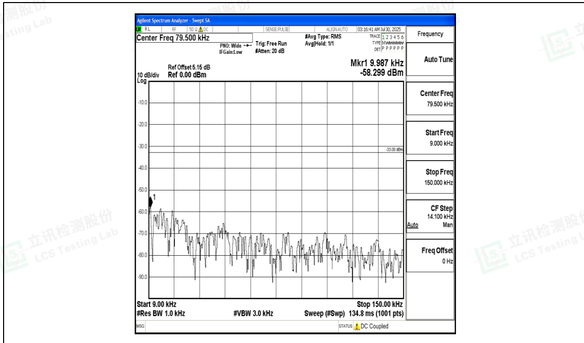
Band17_10MHz_QPSK_23780_1RB#0_0.009~0.15_0.009~0.15
