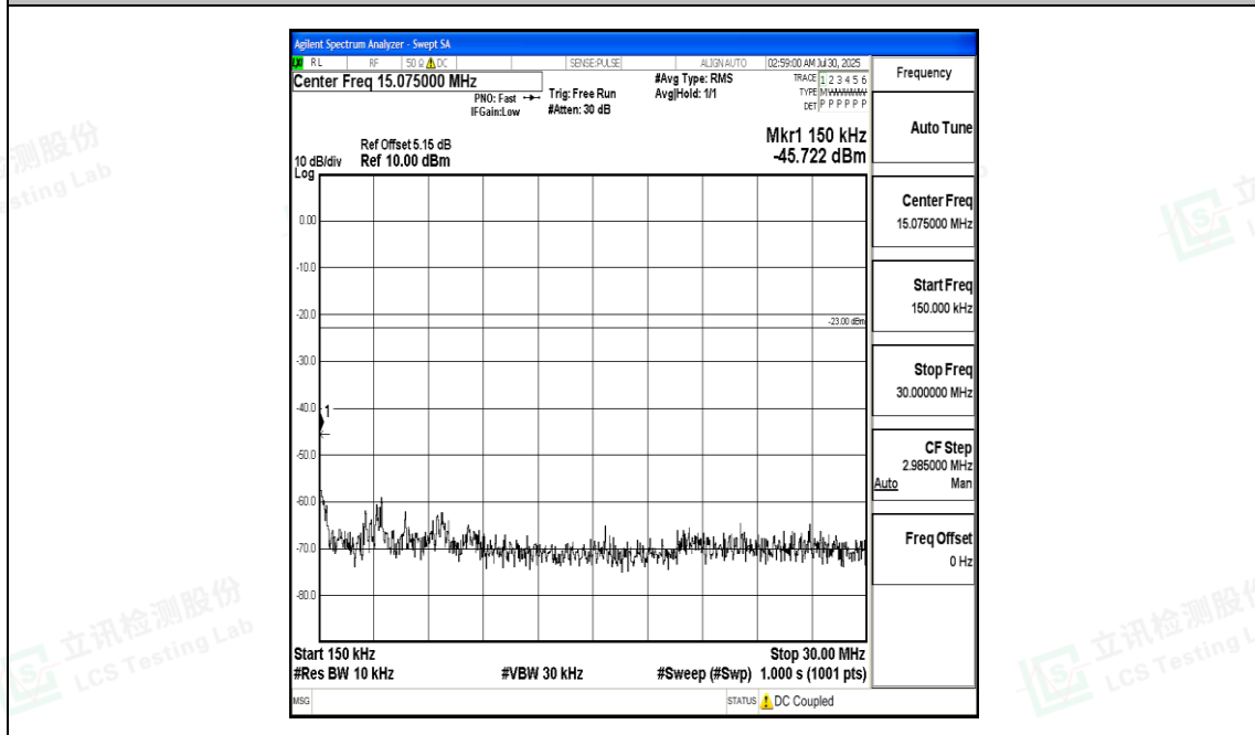
Band17_5MHz_QPSK_23790_1RB#0_0.15~30_0.15~30
