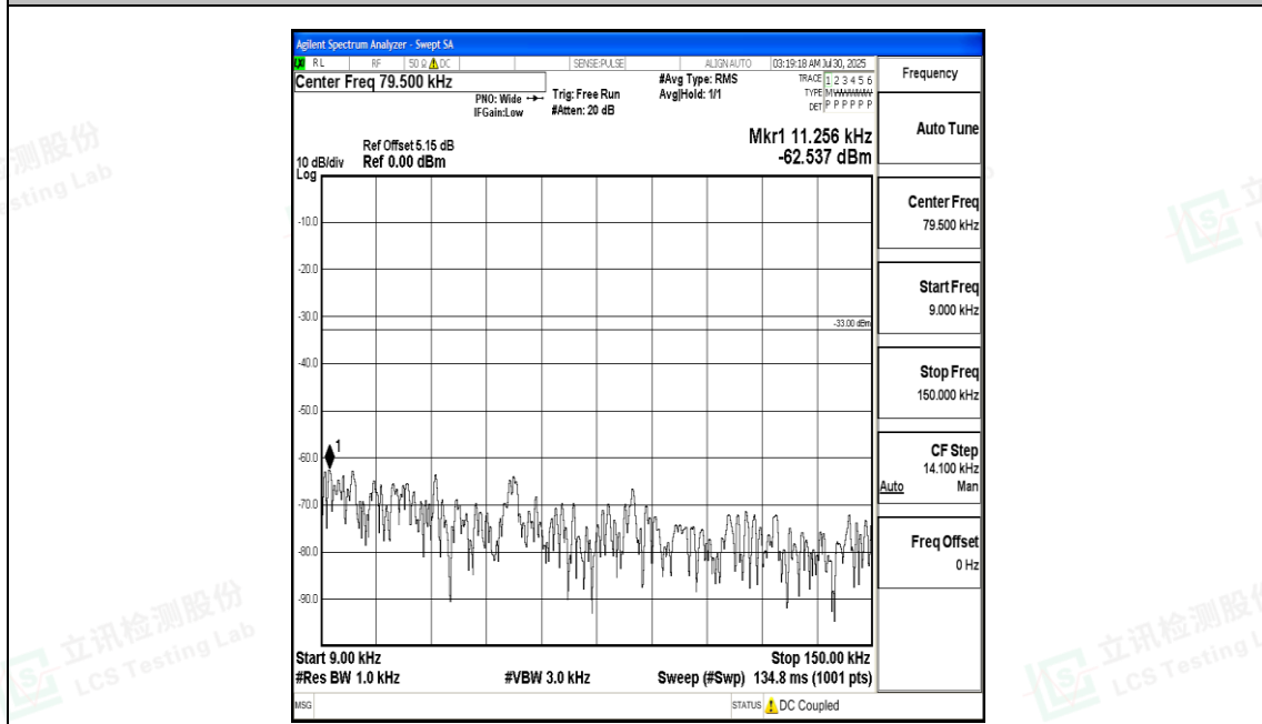
Band17_10MHz_16QAM_23800_1RB#0_0.009~0.15_0.009~0.15
