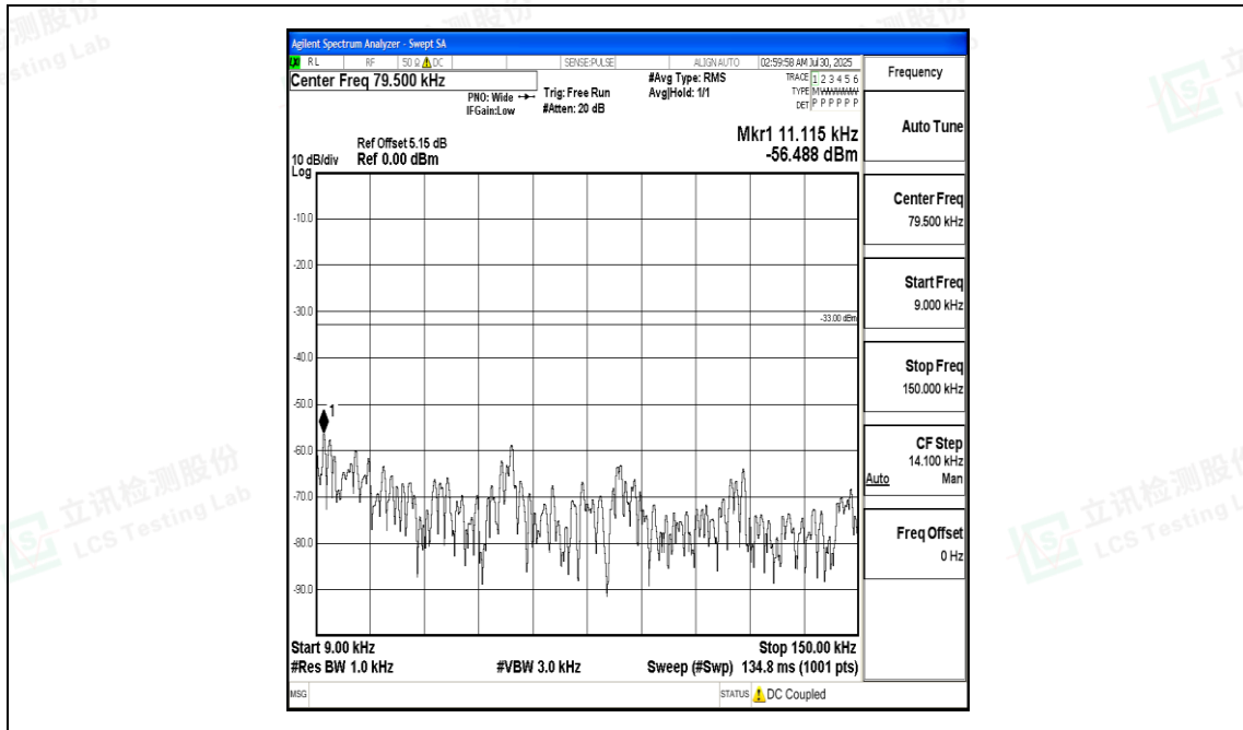
Band17_5MHz_QPSK_23825_1RB#0_0.009~0.15_0.009~0.15
