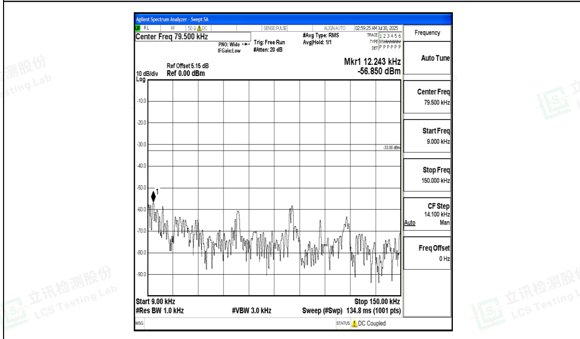
Band17_5MHz_16QAM_23790_1RB#0_0.009~0.15_0.009~0.15
