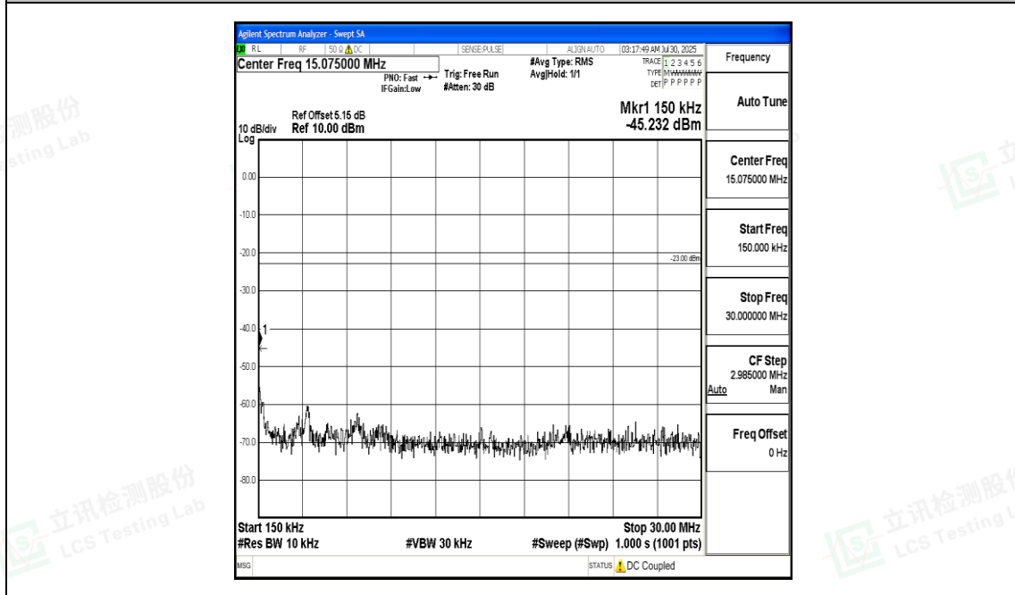
Band17_10MHz_QPSK_23790_1RB#0_0.15~30_0.15~30
