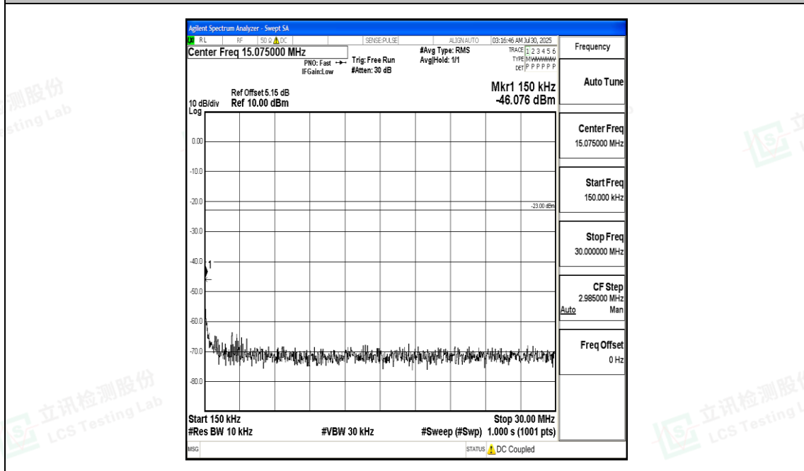
Band17_10MHz_QPSK_23780_1RB#0_0.15~30_0.15~30
