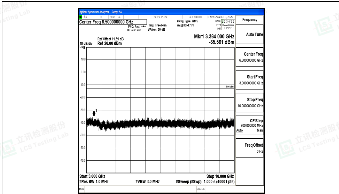
Band17_10MHz_QPSK_23800_1RB#0_3000~10000_3000~10000
