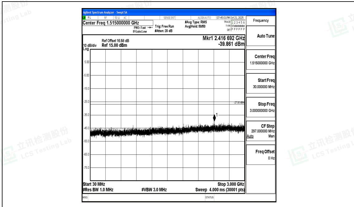
11AX40SISO-Ant0-6445-30~3000-PASS
