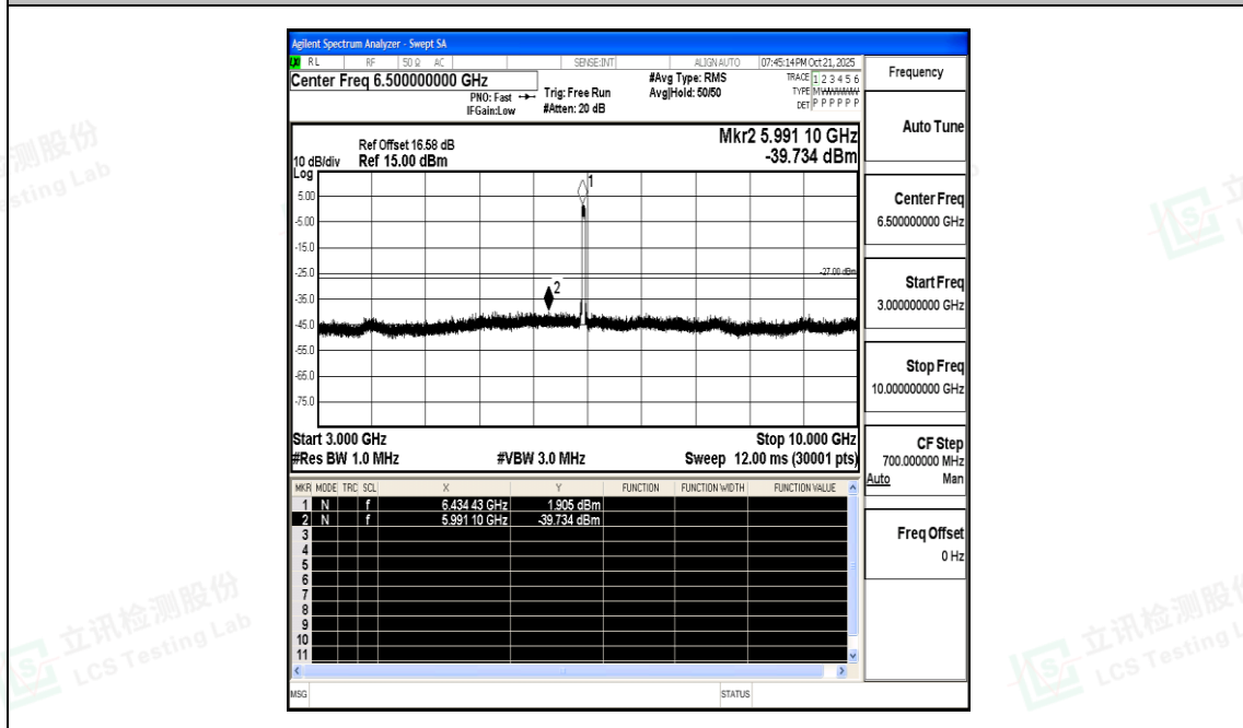
11AX40SISO-Ant0-6445-3000~10000-PASS
