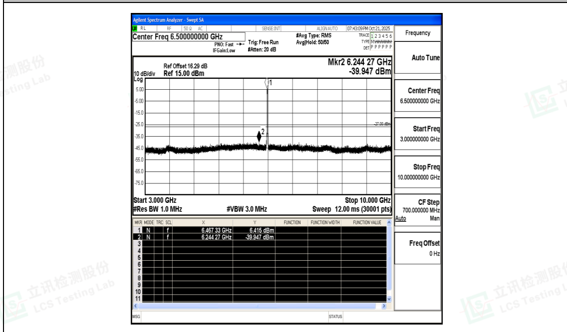
11AX20SISO-Ant0-6475-3000~10000-PASS
