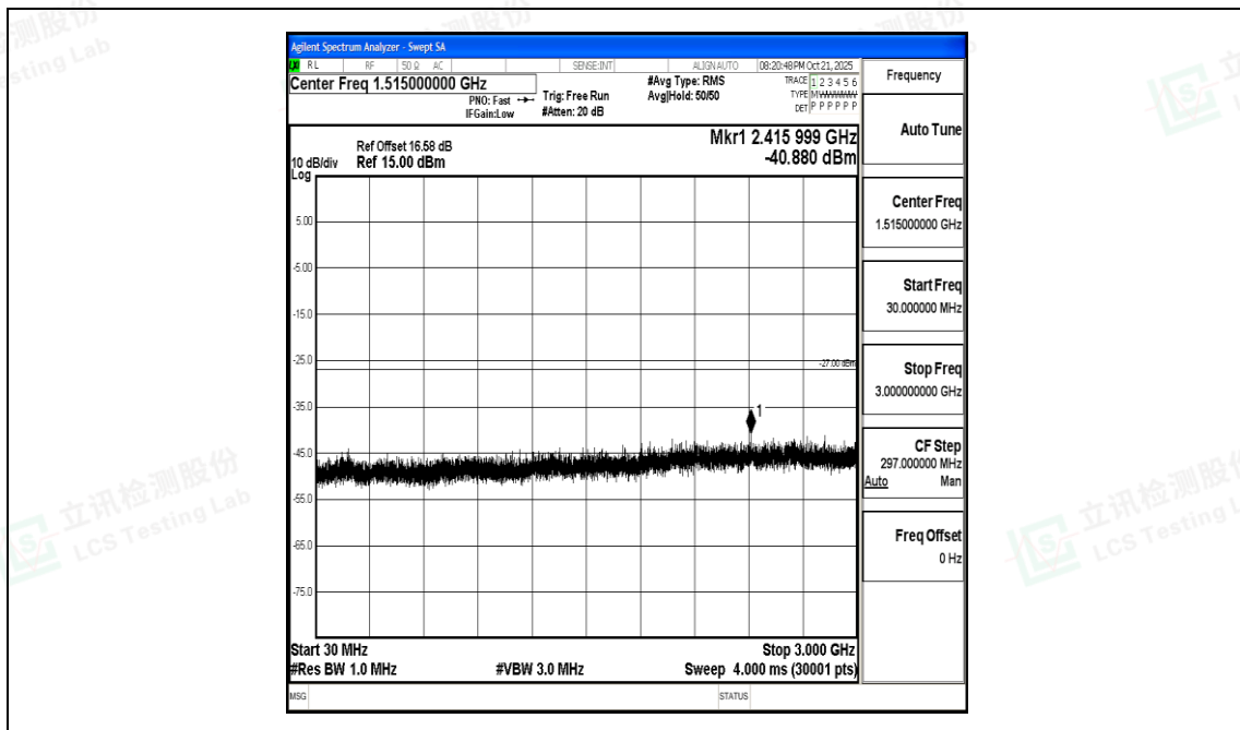
11AX40SISO-Ant1-6445-30~3000-PASS
