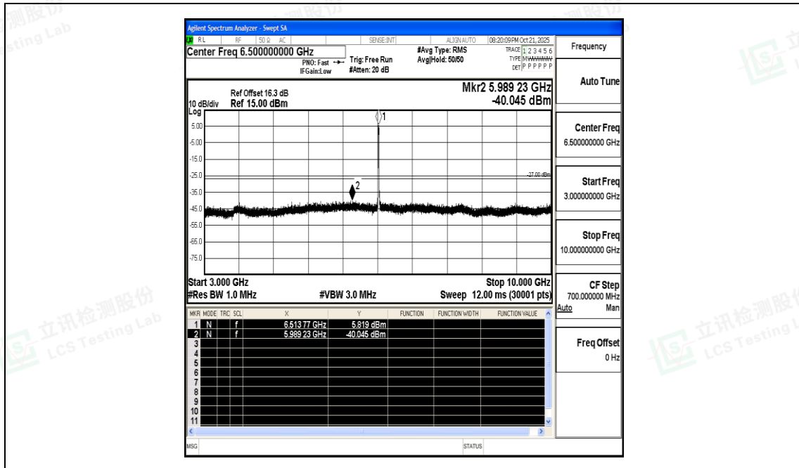
11AX20SISO-Ant1-6515-3000~10000-PASS
