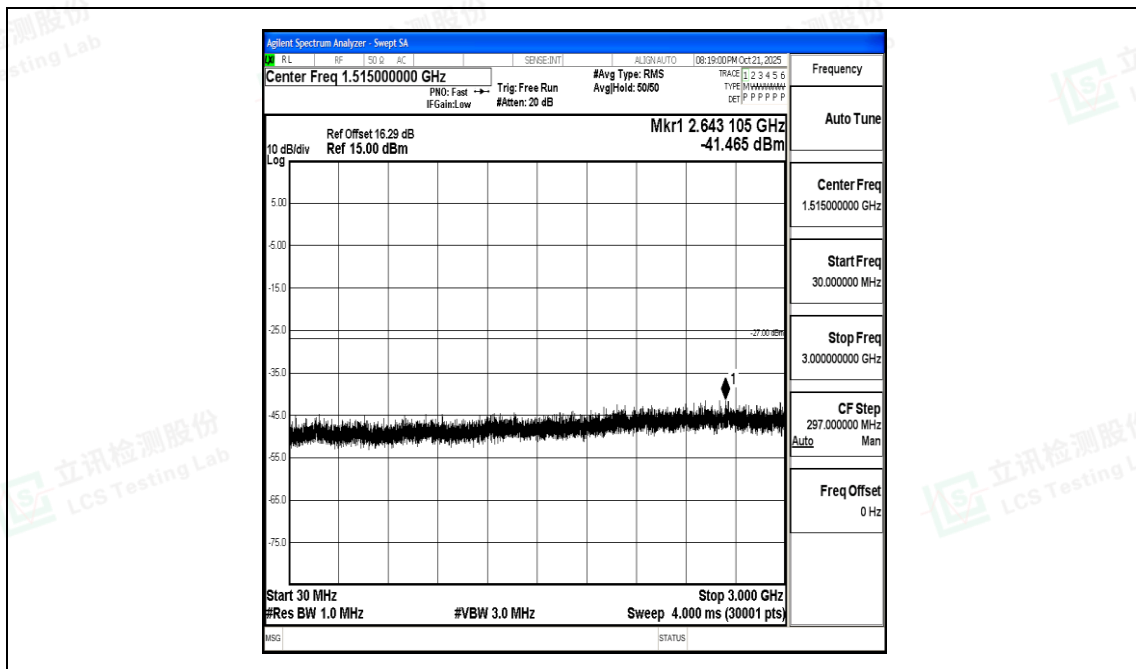
11AX20SISO-Ant1-6475-30~3000-PASS
