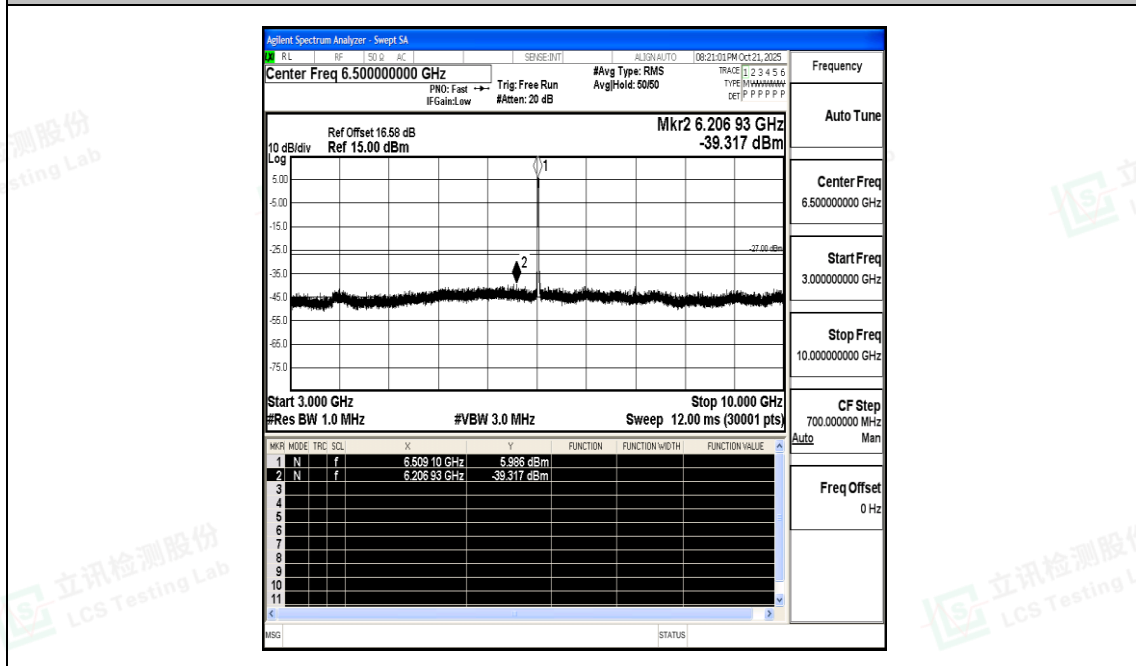
11AX40SISO-Ant1-6445-3000~10000-PASS
