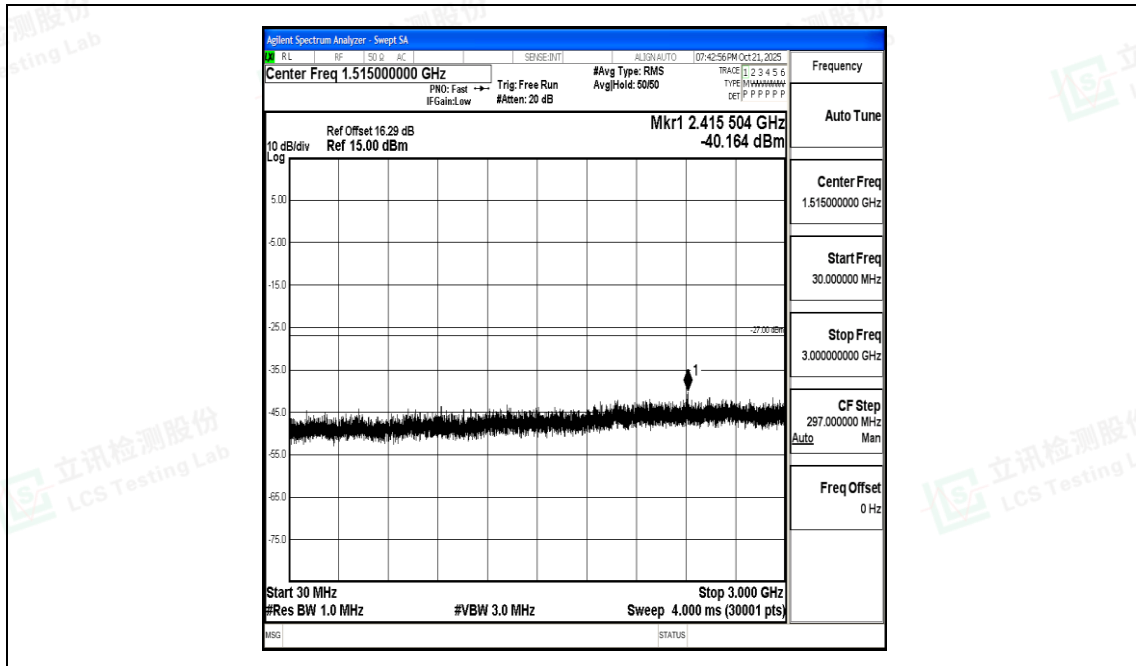
11AX20SISO-Ant0-6475-30~3000-PASS
