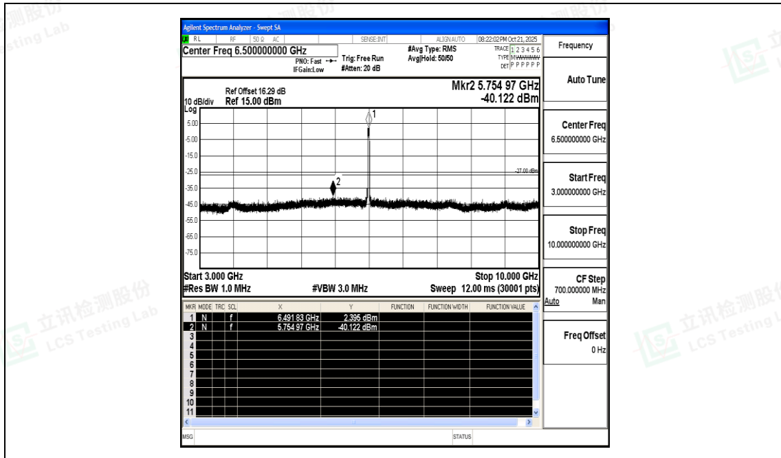
11AX40SISO-Ant1-6485-3000~10000-PASS
