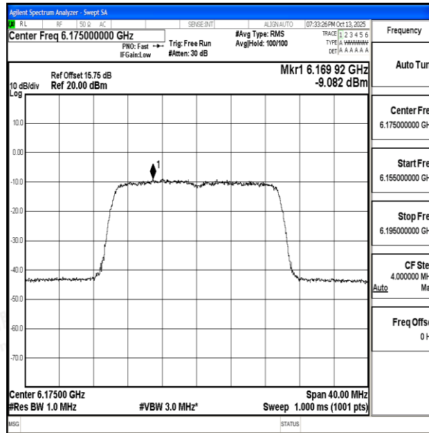
11AX20SISO-Ant1-6175-PASS
