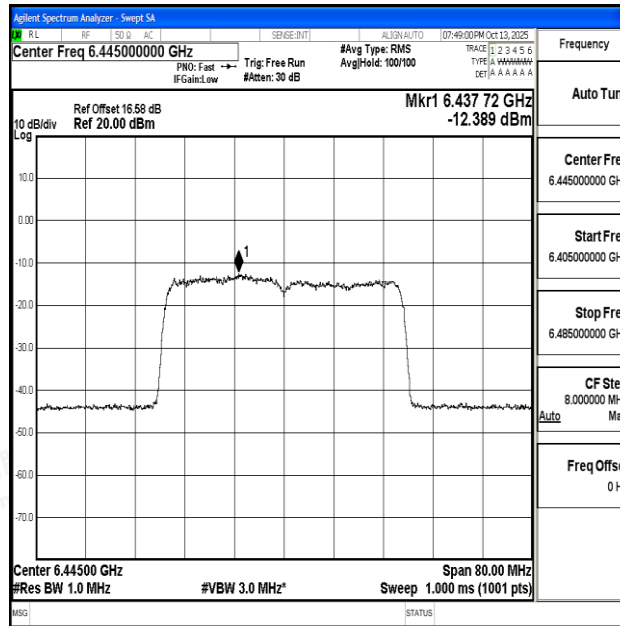
11AX40SISO-Ant0-6445-PASS
