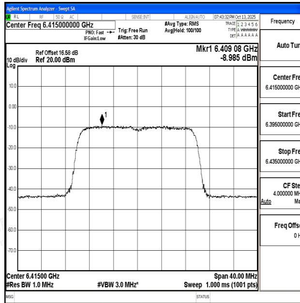
11AX20SISO-Ant0-6415-PASS
