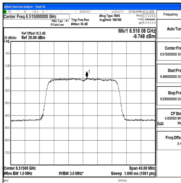
11AX20SISO-Ant0-6515-PASS
