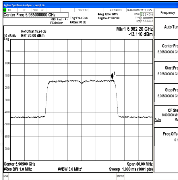
11AX40SISO-Ant1-5965-PASS
