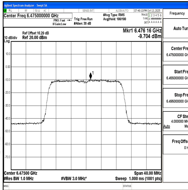
11AX20SISO-Ant0-6475-PASS
