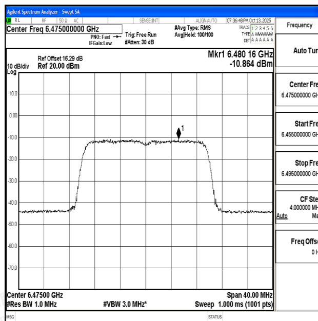
11AX20SISO-Ant1-6475-PASS
