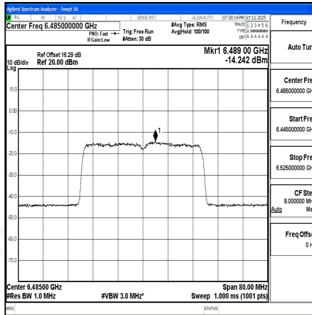
11AX40SISO-Ant1-6485-PASS
