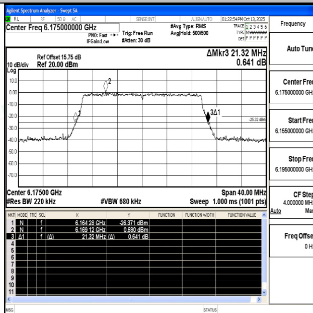
11AX20S|SO-Ant0-6175
