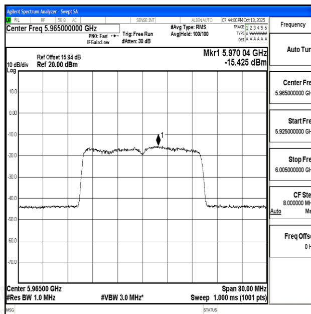
11AX40SISO-Ant0-5965-PASS
