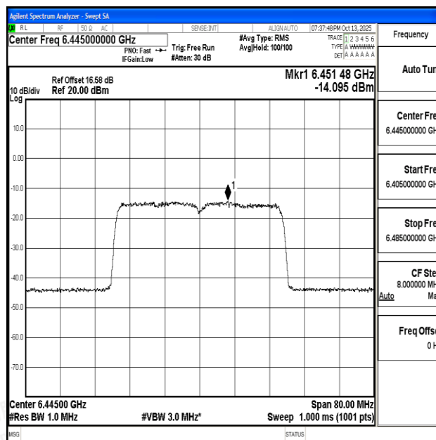
11AX40SISO-Ant1-6445-PASS
