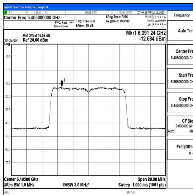
11AX40SISO-Ant0-6405-PASS
