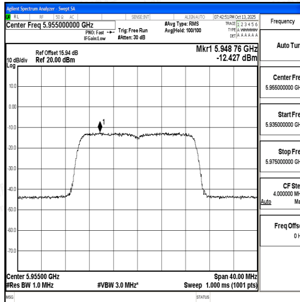
11AX20SISO-Ant0-5955-PASS
