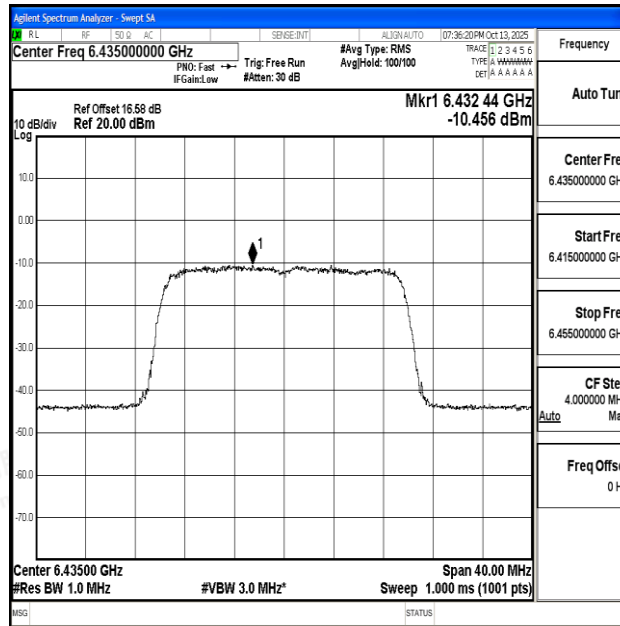
11AX20SISO-Ant1-6435-PASS
