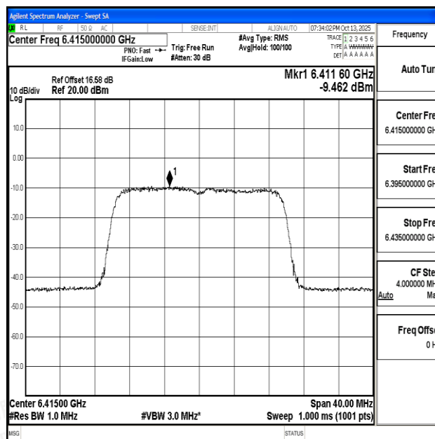
11AX20SISO-Ant1-6415-PASS
