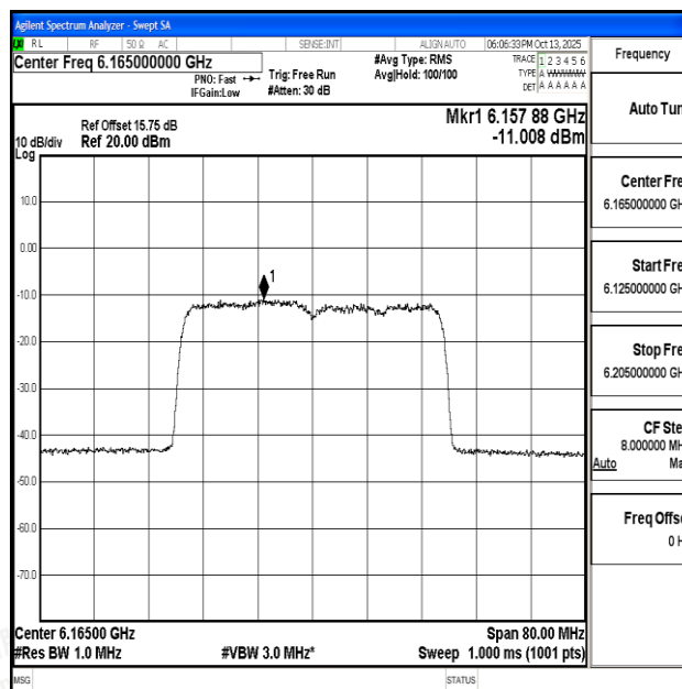
11AX40SISO-Ant1-6165-PASS
