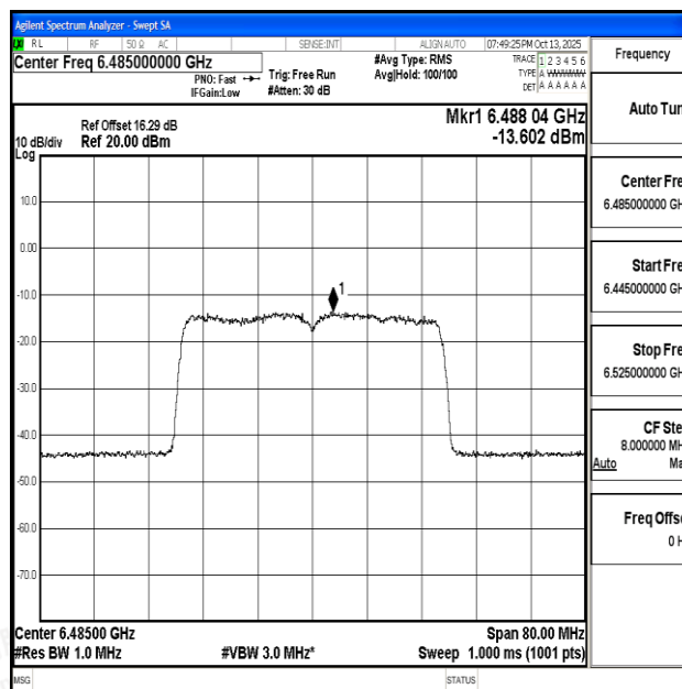
11AX40SISO-Ant0-6485-PASS
