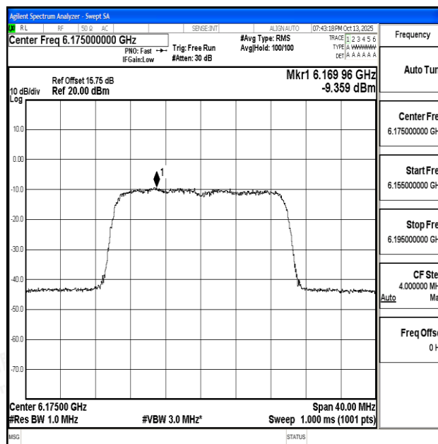
11AX20SISO-Ant0-6175-PASS
