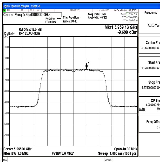
11AX20SISO-Ant1-5955-PASS
