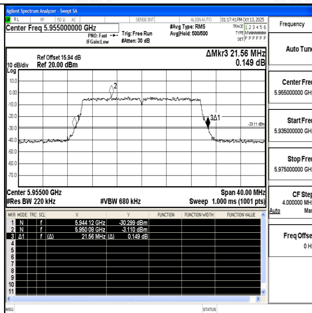
11AX20SISO-Ant0-5955
