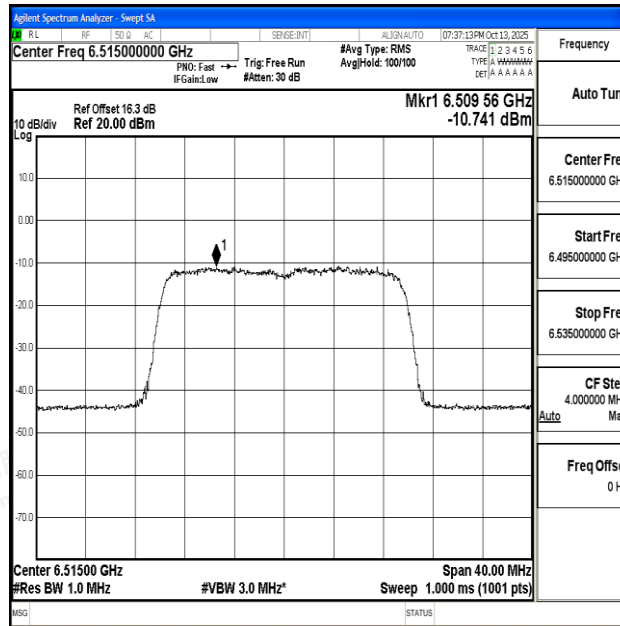
11AX20SISO-Ant1-6515-PASS
