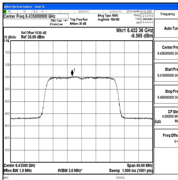
11AX20SISO-Ant0-6435-PASS
