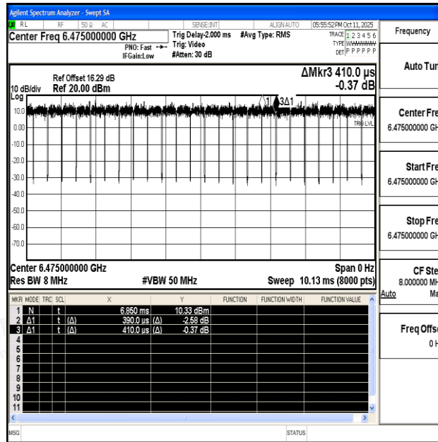
NTNV-11AX20SISO-Ant0-6475
