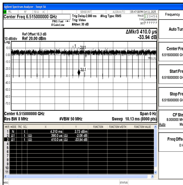
NTNV-11AX20SISO-Ant1-6515
