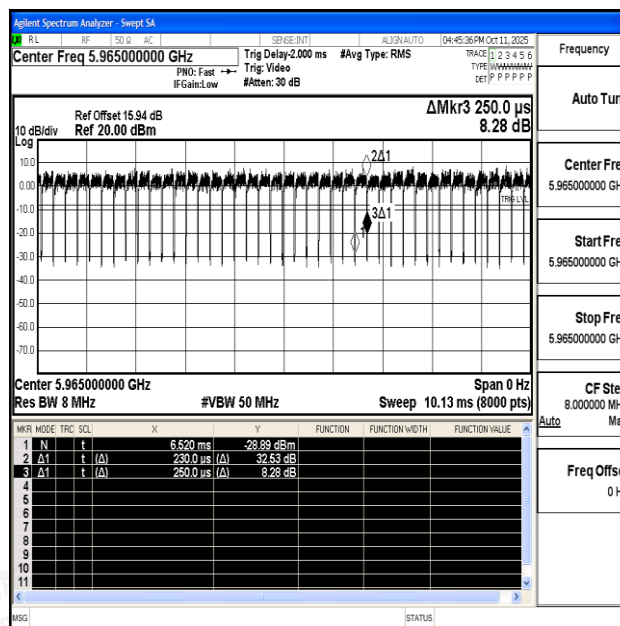
NTNV-11AX40SISO-Ant1-5965
