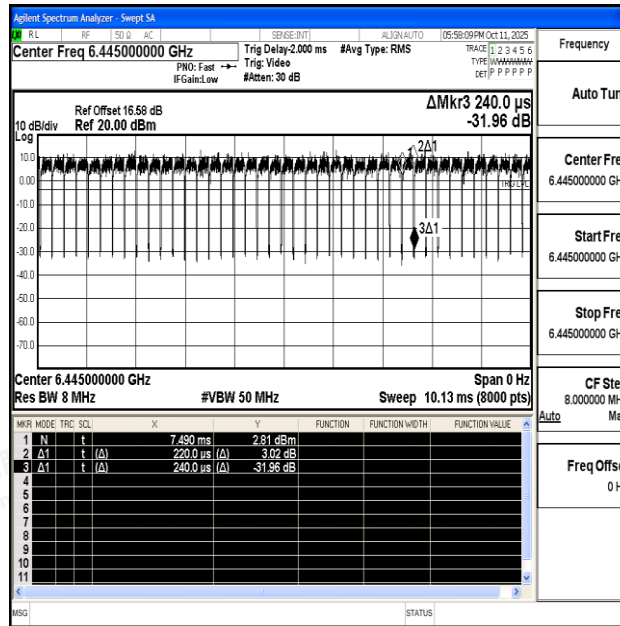
NTNV-11AX40SISO-Ant0-6445
