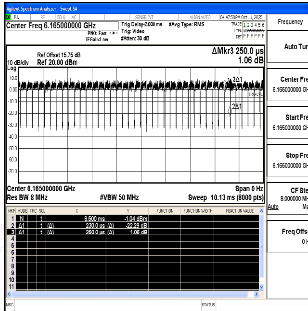
NTNV-11AX40SISO-Ant1-6165
