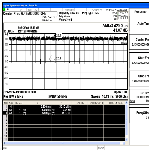
NTNV-11AX20SISO-Ant0-6435
