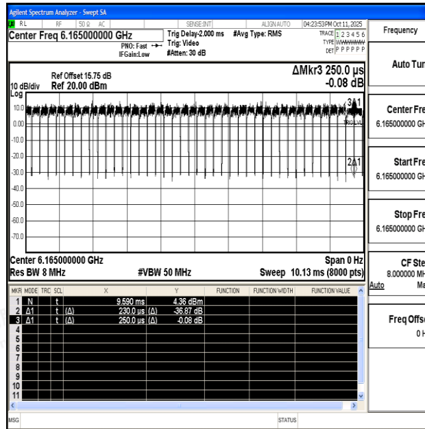
NTNV-11AX40SISO-Ant0-6165
