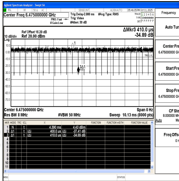
NTNV-11AX20SISO-Ant1-6475
