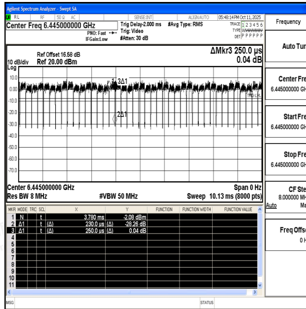
NTNV-11AX40SISO-Ant1-6445
