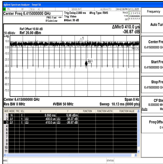
NTNV-11AX20SISO-Ant1-6415
