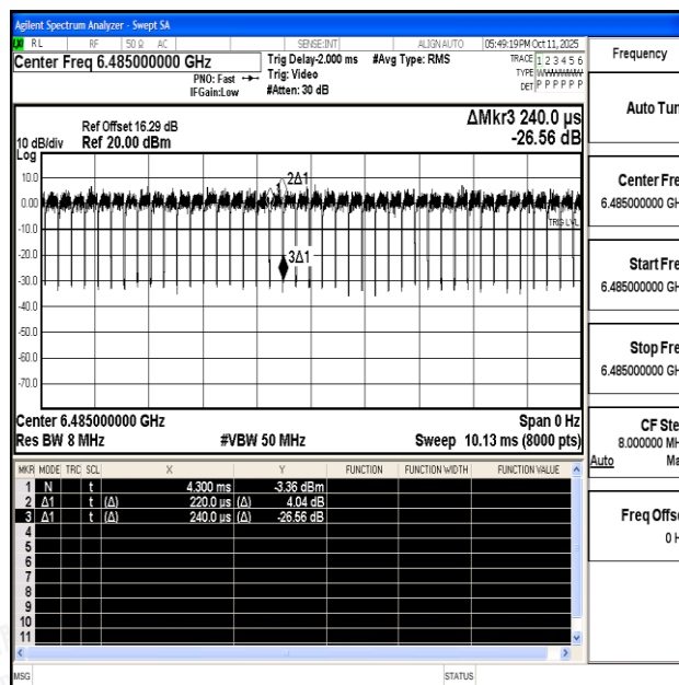
NTNV-11AX40SISO-Ant1-6485
