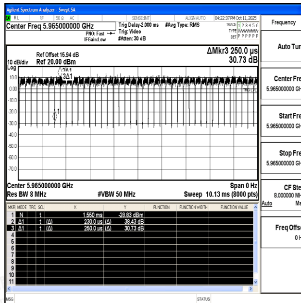
NTNV-11AX40SISO-Ant0-5965
