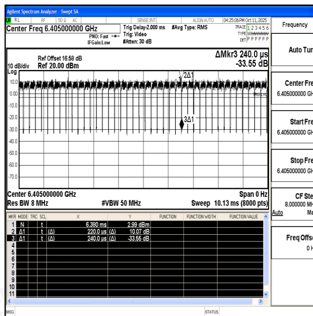
NTNV-11AX40SISO-Ant0-6405
