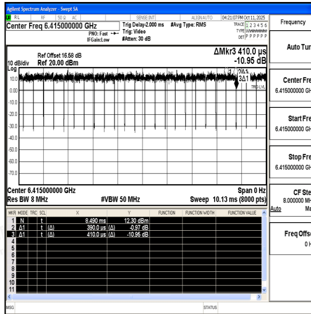
NTNV-11AX20SISO-Ant0-6415
