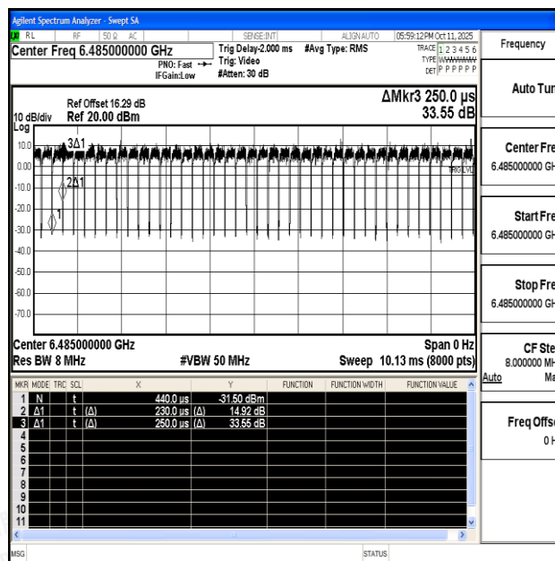
NTNV-11AX40SISO-Ant0-6485
