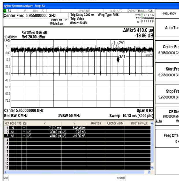
NTNV-11AX20SISO-Ant1-5955
