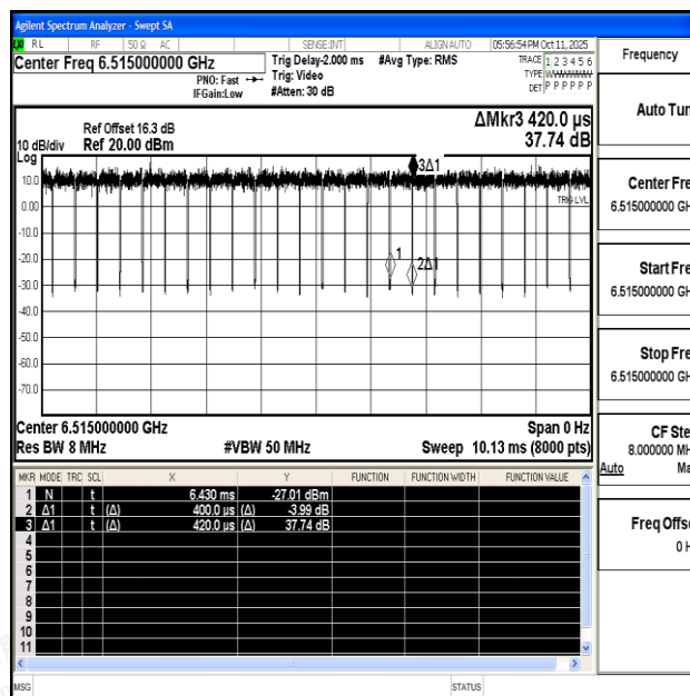
NTNV-11AX20SISO-Ant0-6515
