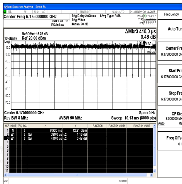
NTNV-11AX20SISO-Ant0-6175
