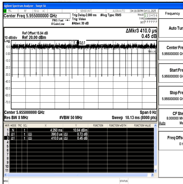
NTNV-11AX20SISO-Ant0-5955
