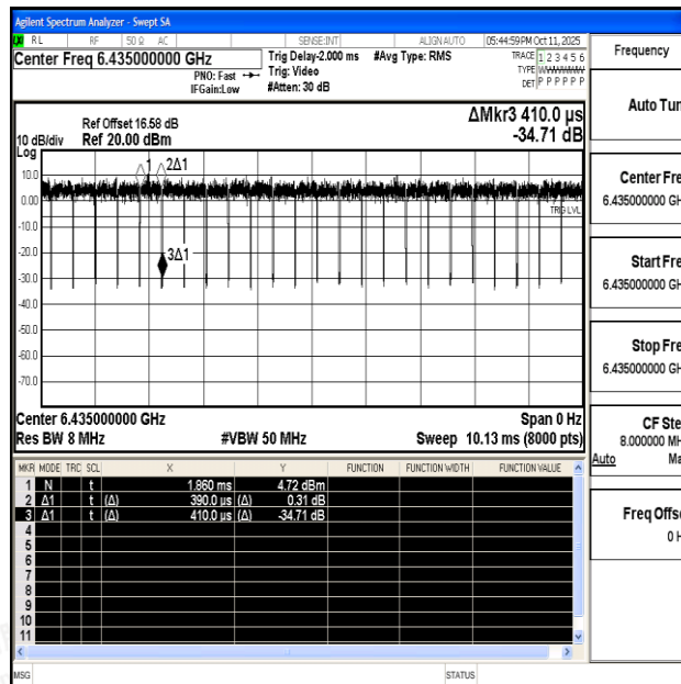
NTNV-11AX20SISO-Ant1-6435
