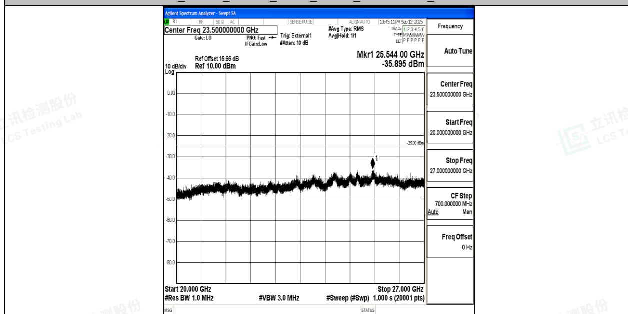
Band38_20MHz_16QAM_37850_1RB#0_20000~27000_20000~27000
