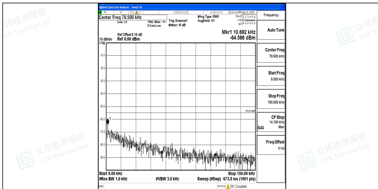
Band38_20MHz_QPSK_37850_1RB#0_0.009~0.15_0.009~0.15
