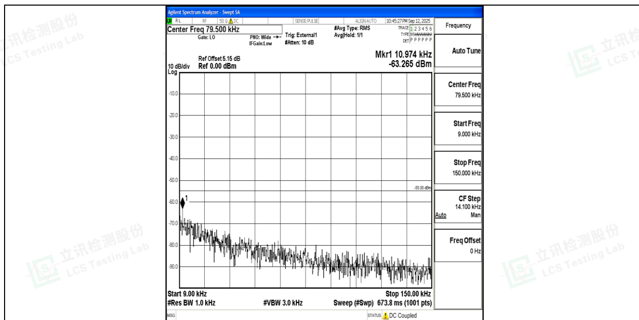
Band38_20MHz_QPSK_38000_1RB#0_0.009~0.15_0.009~0.15
