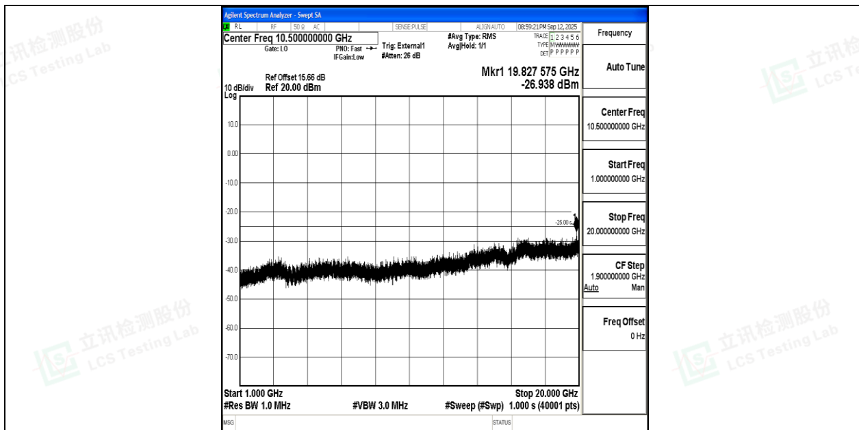
Band38_15MHz_16QAM_38175_1RB#0_1000~20000_1000~20000
