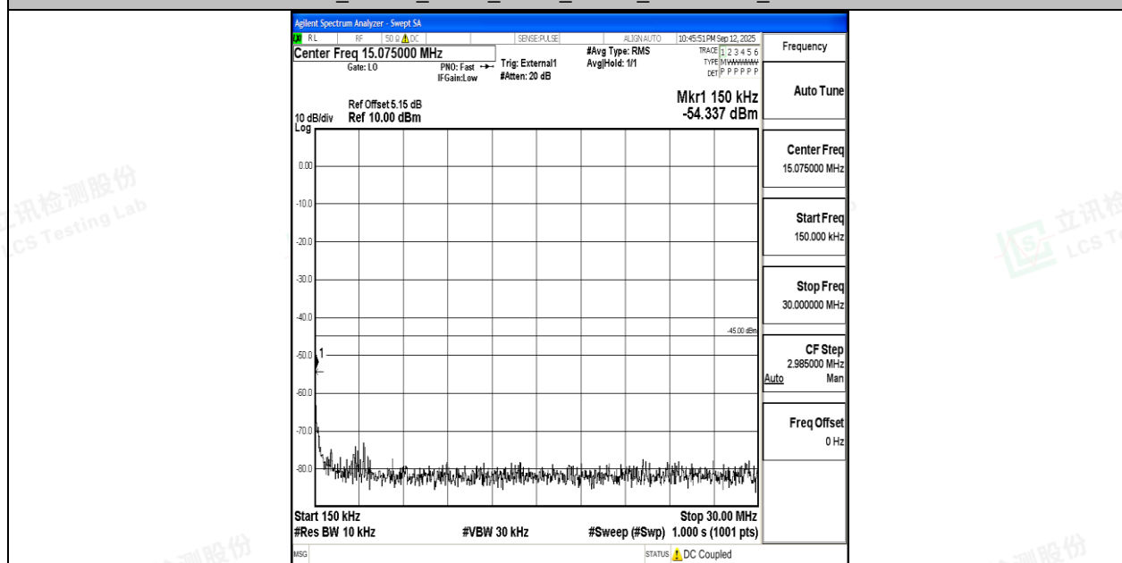
Band38_20MHz_QPSK_38000_1RB#0_0.15~30_0.15~30
