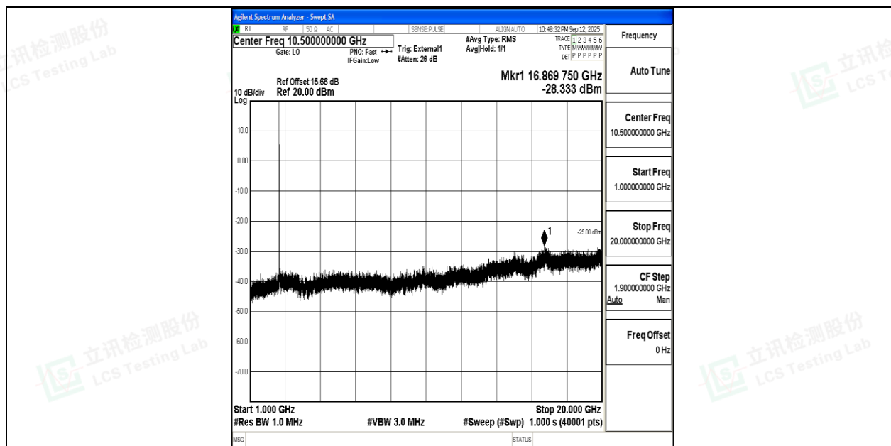
Band38_20MHz_16QAM_38000_1RB#0_1000~20000_1000~20000
