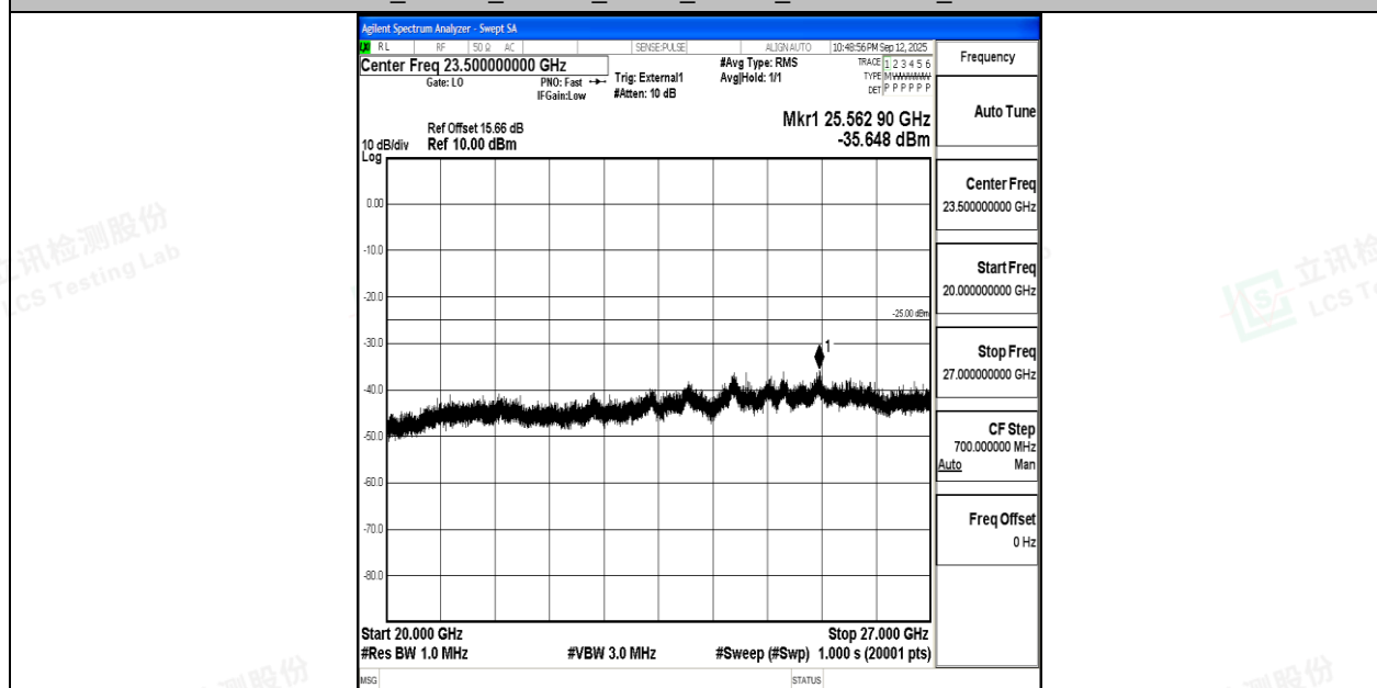
Band38_20MHz_16QAM_38000_1RB#0_20000~27000_20000~27000
