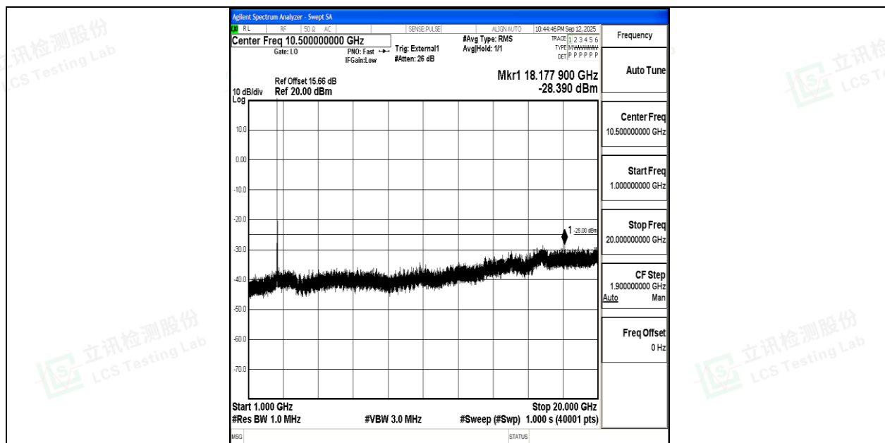
Band38_20MHz_16QAM_37850_1RB#0_1000~20000_1000~20000
