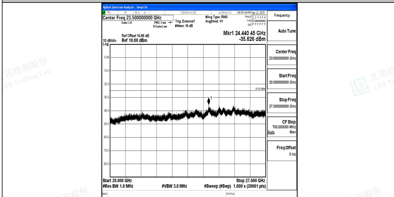
Band38_15MHz_16QAM_38175_1RB#0_20000~27000_20000~27000
