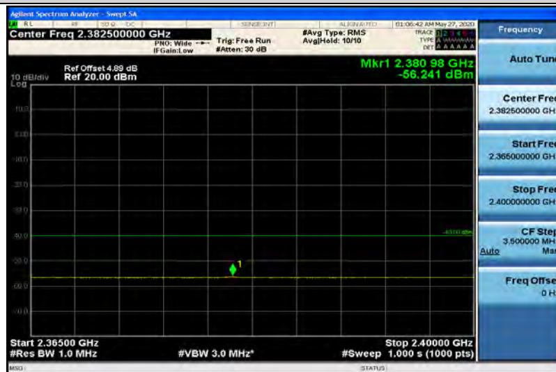
Band40-5MHz-16QAM-38775-1RB#0-Range14:2365~2400MHz
