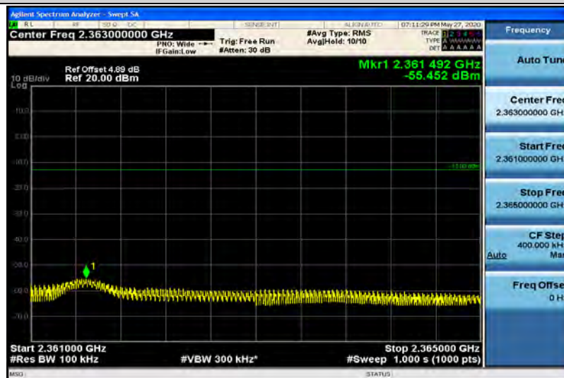
Band40-5MHz-16QAM-39200-1RB#24-Range14:2361~2365MHz
