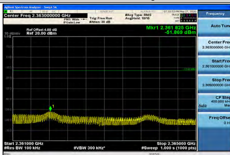
Band40-5MHz-16QAM-39225-1RB#24-Range13:2361~2365MHz
