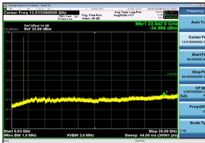
FDD02_HighRange_20MHz_30MHz~26GHz
