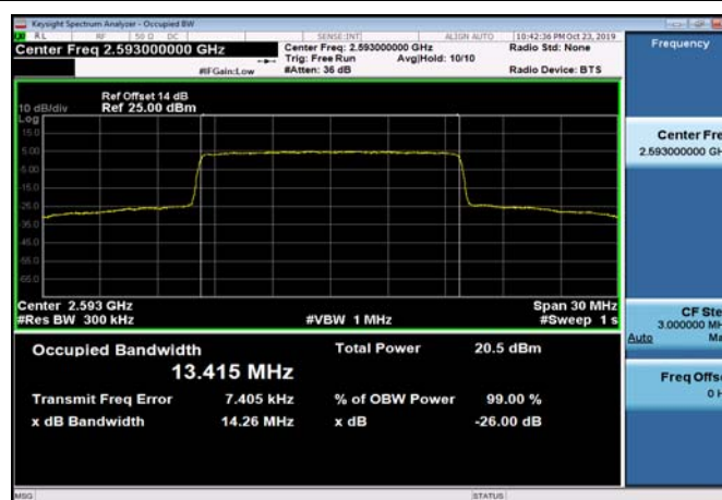
TDD41_MidRange_15MHz_2593MHz_Q16
