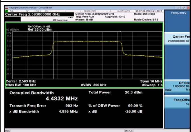
TDD41_MidRange_5_2593_Q16
