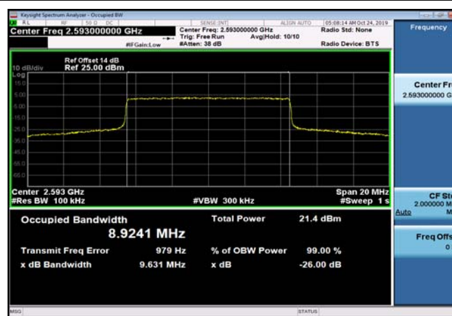
TDD41_MidRange_15_2593_QPSK
