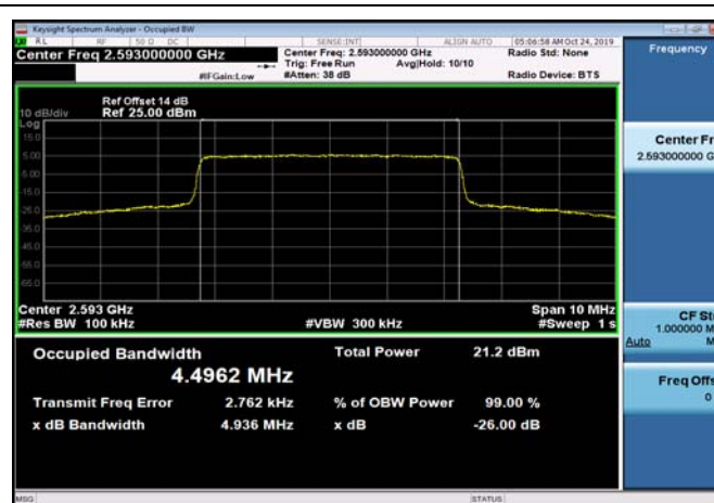
TDD41_MidRange_5_2593_QPSK
