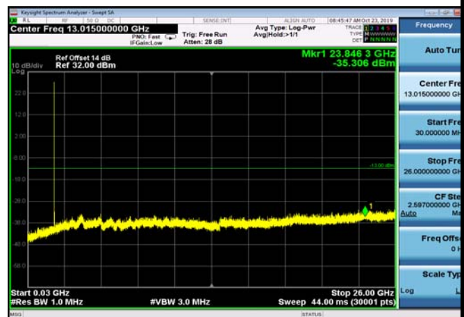
FDD02_LowRange_1.4MHz_30MHz~26GHz
