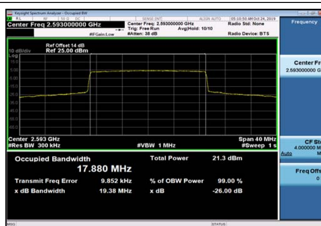
TDD41_MidRange_20_2593_QPSK
