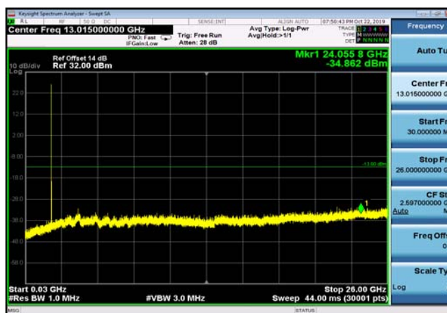
FDD02_HighRange_5MHz_30MHz~26GHz
