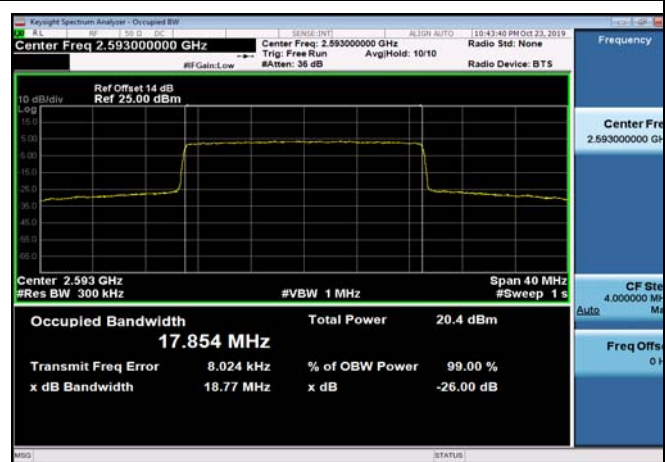
TDD41_MidRange_20MHz_2593MHz_Q16
