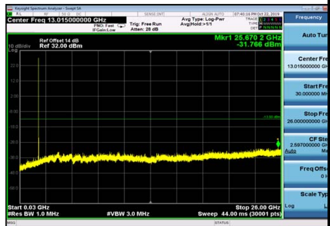
FDD02_HighRange_3MHz_30MHz~26GHz
