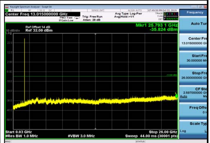
FDD02_MidRange_10MHz_30MHz~26GHz
