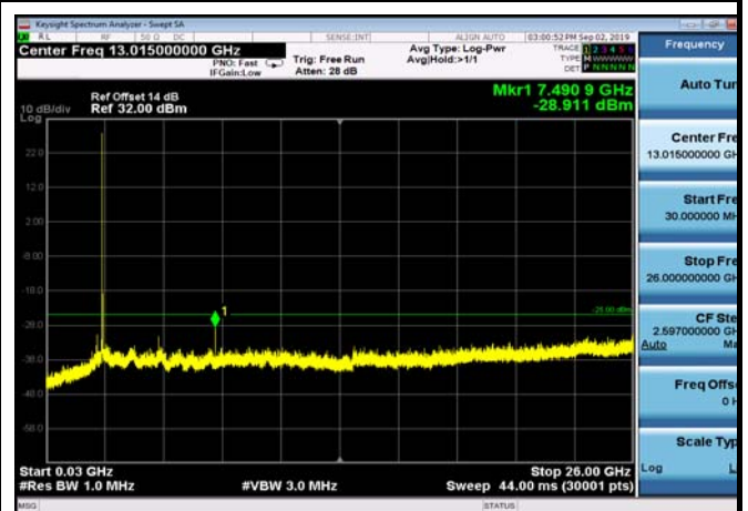
TDD41_MidRange_15MHz_30MHz~26GHz
