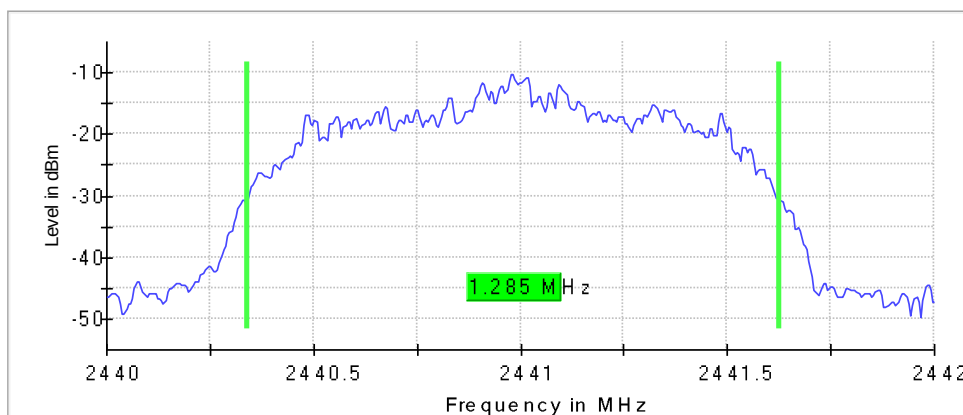
20 dB Bandwidth
