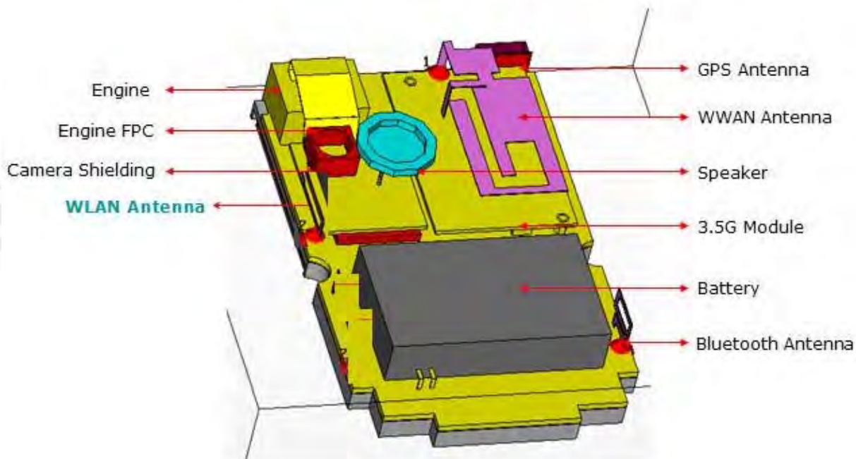
Fig.13 Antenna position of EUT
