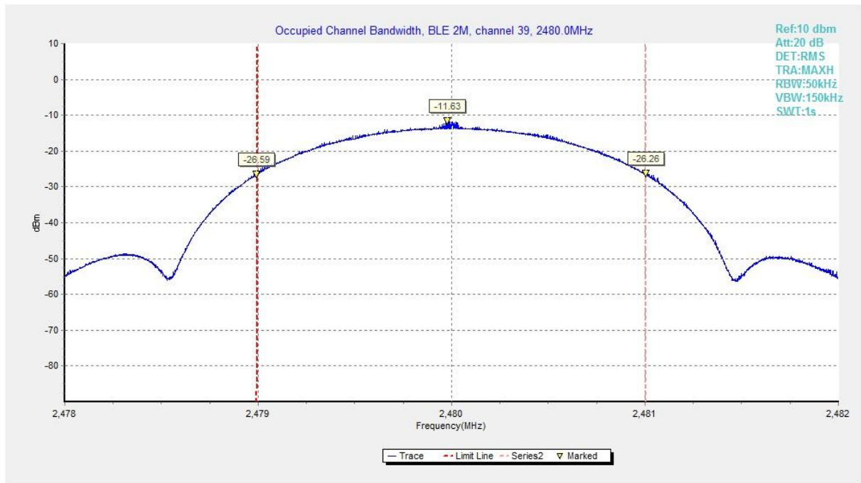
Fig.56 99% Occupied Bandwidth (Ch 39), LE 2M
