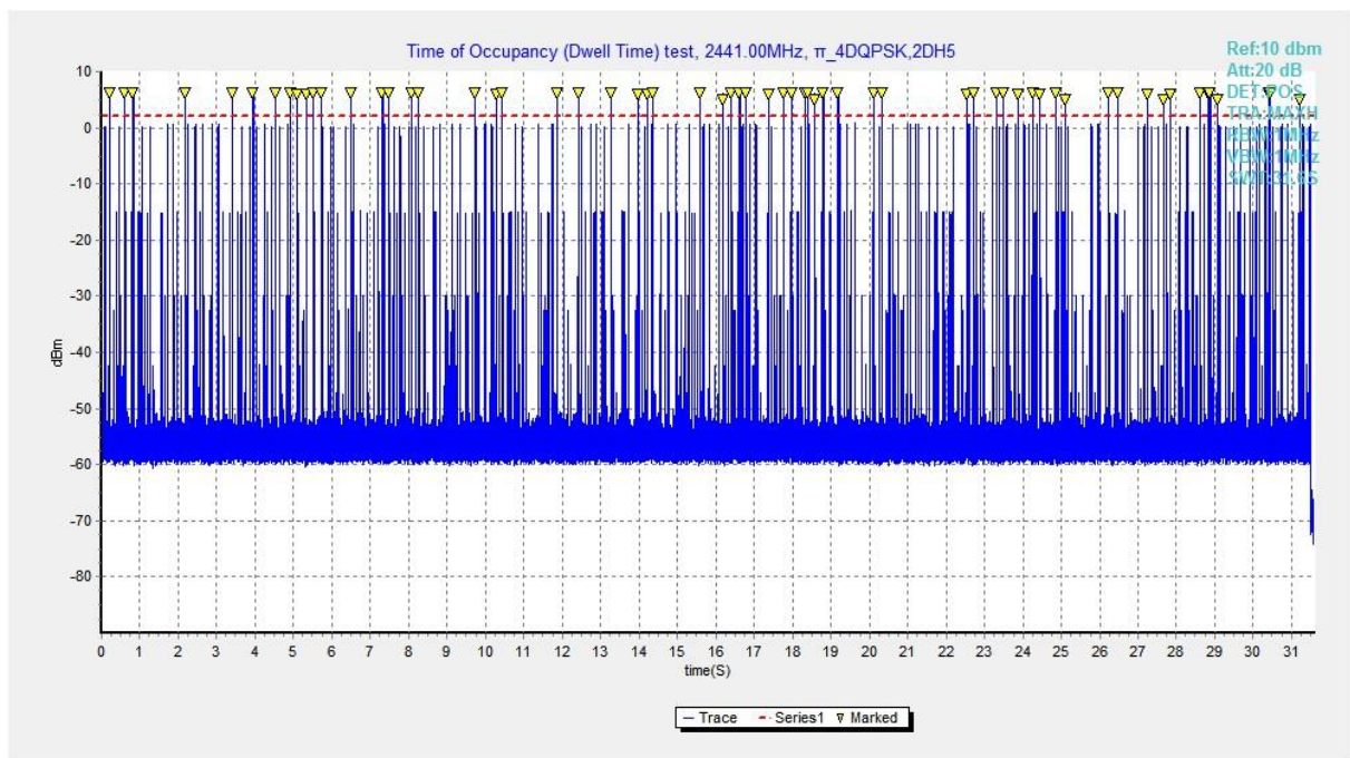
Fig. 63 Time of Occupancy(Dwell Time) ( \pi /4 DQPSK, Ch39)
