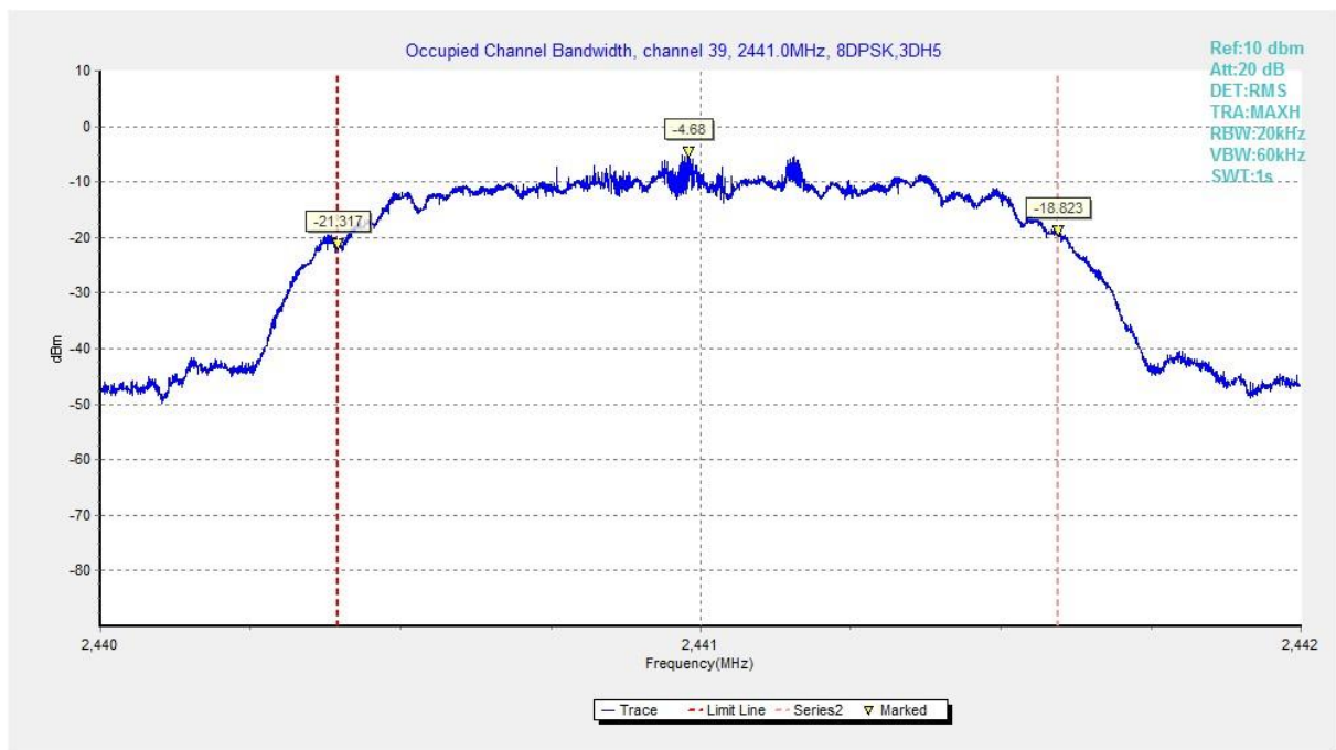
Fig. 84 99% Occupied Bandwidth (8DPSK, Ch 39)
