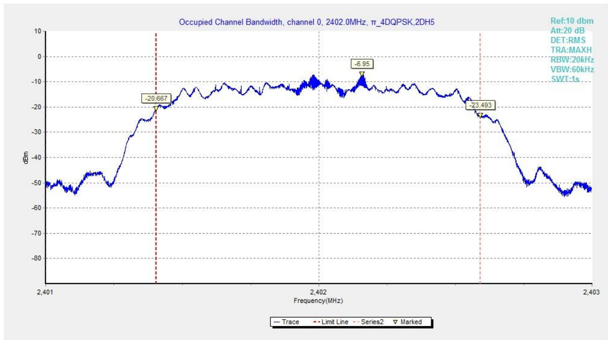
Fig. 80 99% Occupied Bandwidth ( \pi /4 DQPSK, Ch 0)
