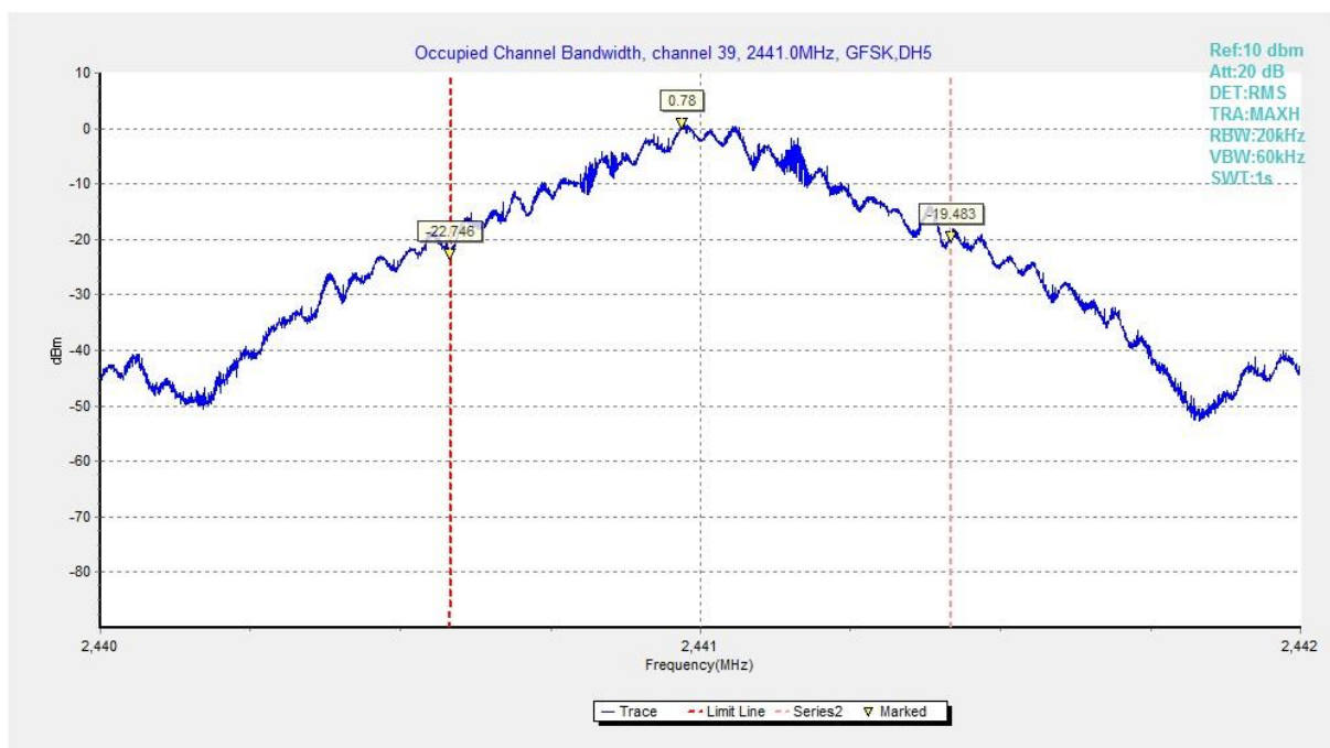
Fig. 78 99% Occupied Bandwidth (GFSK, Ch 39)
