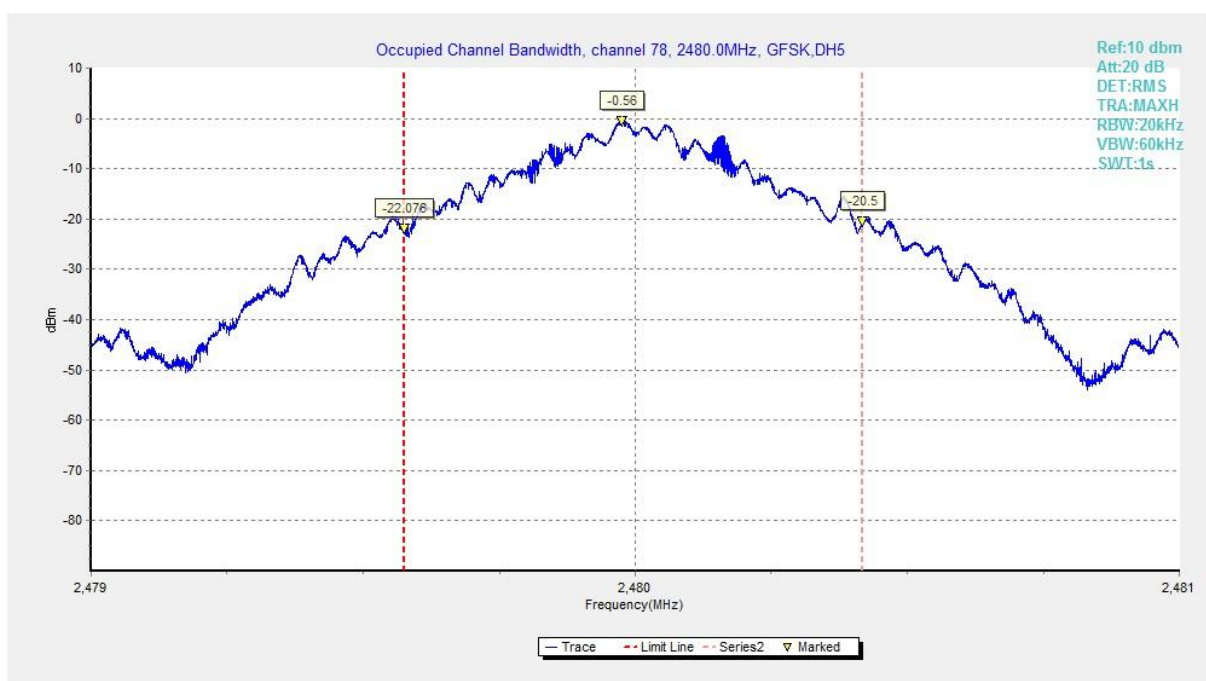
Fig. 79 99% Occupied Bandwidth (GFSK, Ch 78)
