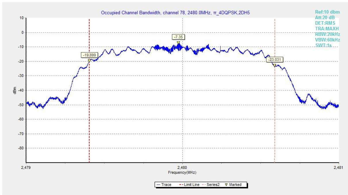
Fig. 82 99% Occupied Bandwidth ( \pi/4 DQPSK, Ch 78)
