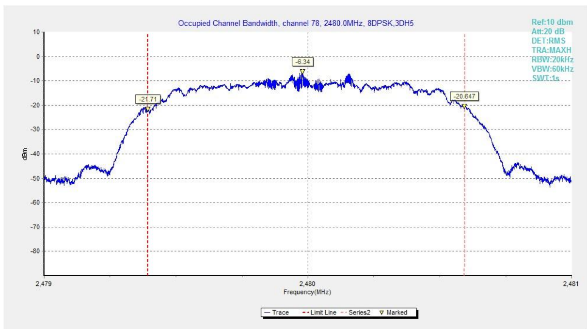
Fig. 85 99% Occupied Bandwidth (8DPSK, Ch 78)
