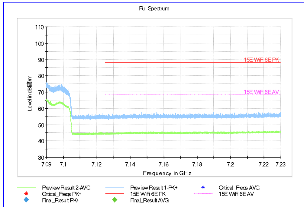
Fig.140 Band Edges (802.11ax VHT-40, 7085MHz)
